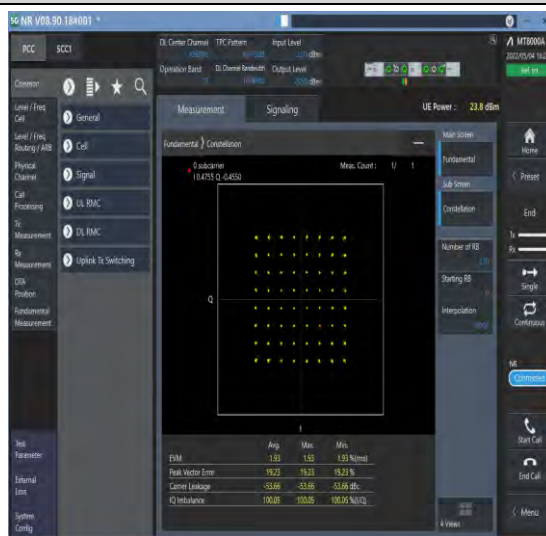
1-N77-3700-3980-PC2-30-100-M-4-DFT-64QAM-Out_Full-270@0-Ant1-see graph-PASS
