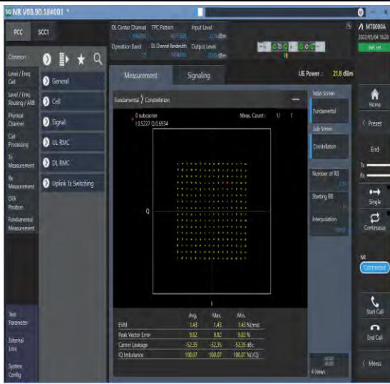
1-N77-3700-3980-PC2-30-100-M-5-DFT-256QAM-Outer_Full-270@0-Ant1-see graph-PASS
