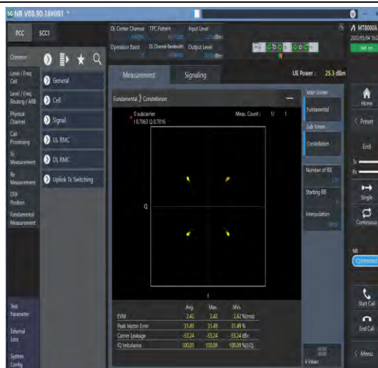
1-N77-3700-3980-PC2-30-100-M-2-DFT-QPSK-Out_Full-270@0-Ant1-see graph-PASS
