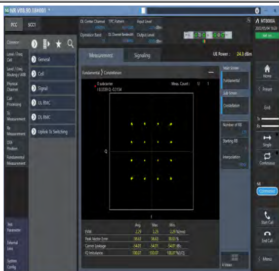
1-N77-3700-3980-PC2-30-100-M-3-DFT-16QAM-Out_Full-270@0-Ant1-see graph-PASS
