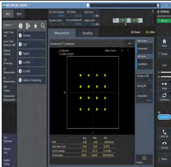
1-N77-3700-3980-PC2-30-100-M-7-CP-16QAM-Outer_Full-273@0-Ant1-see graph-PASS
