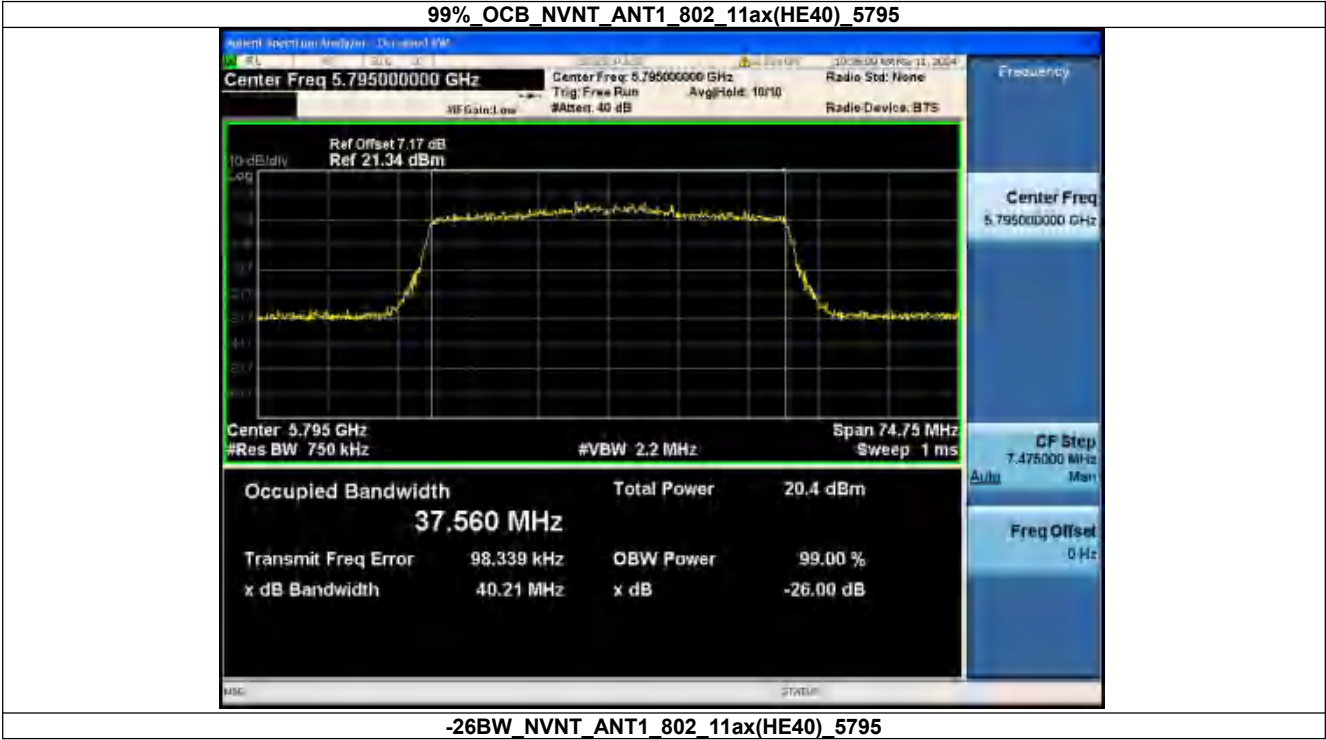
99%_OCB_NVNT_ANT1_802_11ax(HE40)_5795
