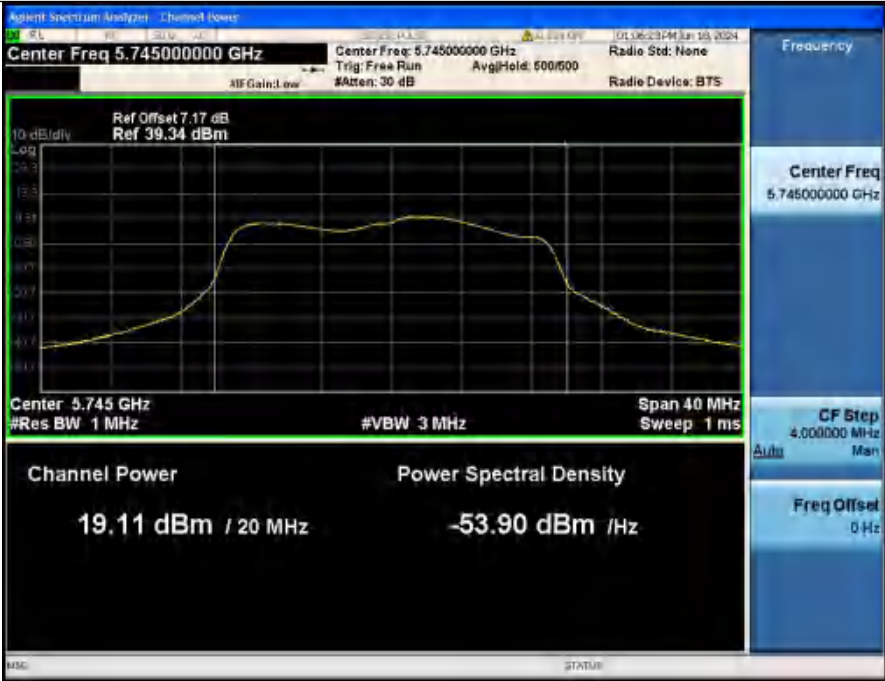
Maximum Conducted Output Power NVNT_ANT2_802_11n(HT20)_5745
