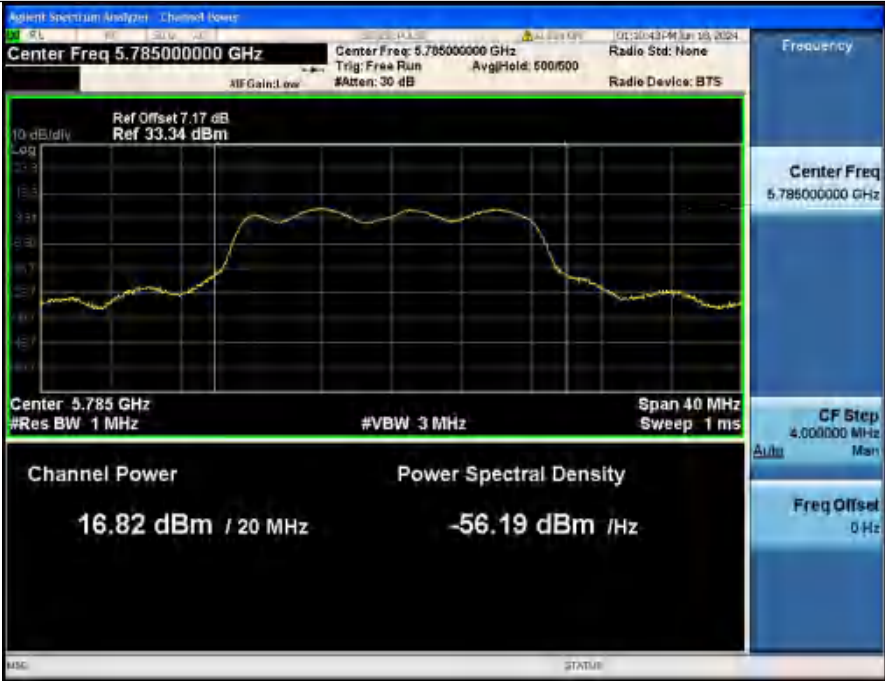
Maximum Conducted Output Power NVNT_ANT2_802_11a_5785
