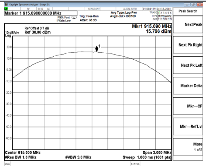
Channel 13 / 915 MHz
