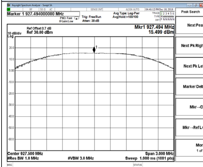
Channel 26 / 927.5 MHz
