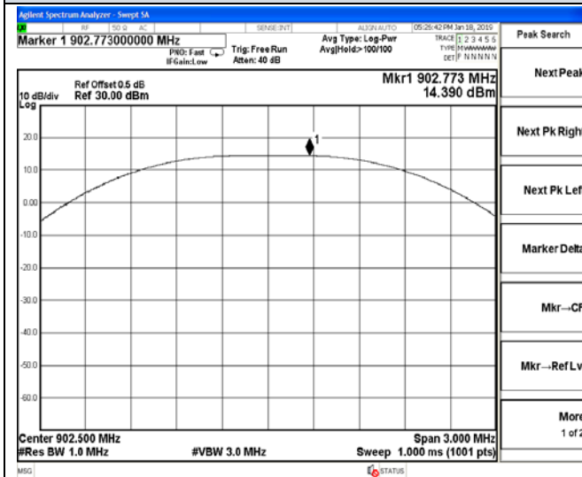
Channel 0 / 902.5 MHz
