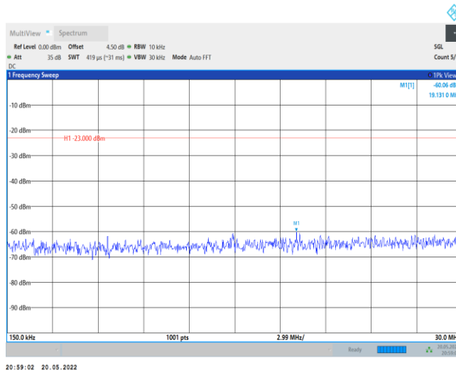
Band26-15MHz-QPSK-26865-1RB#0-Range2:0.15~30MHz
