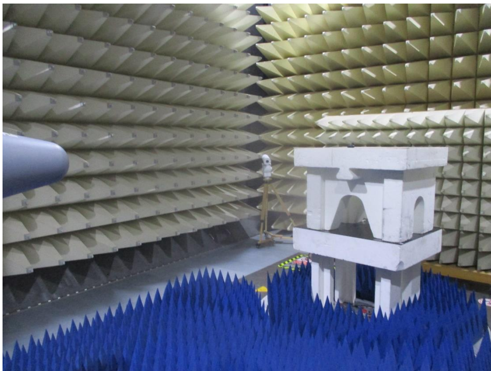
Photograph 2: Set-up photo for Radiated Emission, 1GHz - 6GHz
