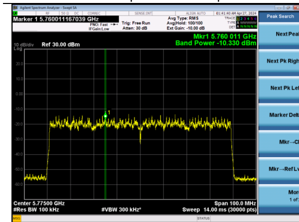
802.11ax80 | Channel 155 | MCS11
