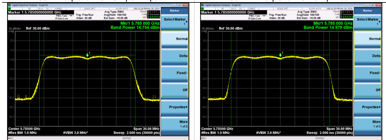
802.11ac20 | Channel 157 | MCS0
