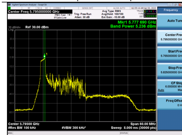
802.11ax40 | Channel 159 | MCS0 | RU26
