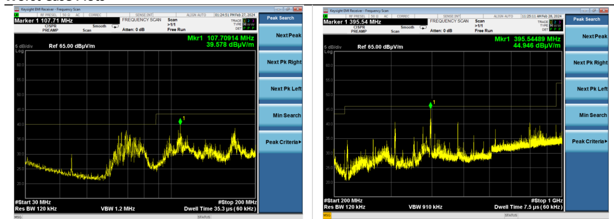
802.11a | Channel 165 | 6 Mbps | Y Plane 30-200 MHz | Horizontal
