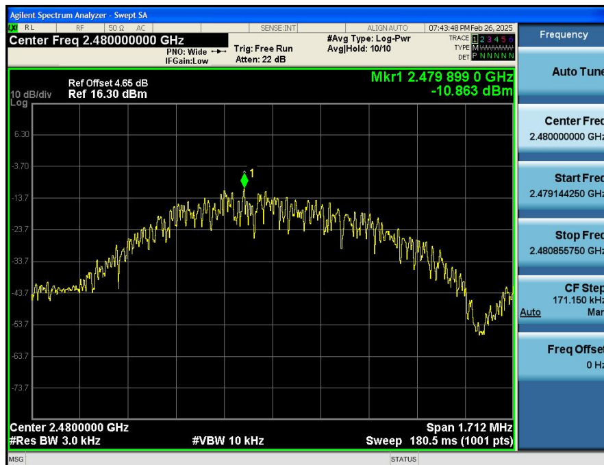
Power_Spectral_Density_NVNT_ANT1_1Mbps_2480
