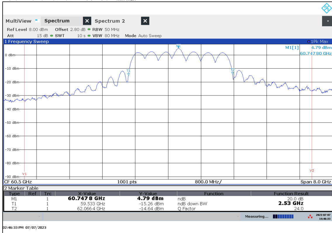
Plot 27: 20 dB-Bandwidth at T= 50 °C / V min-max
