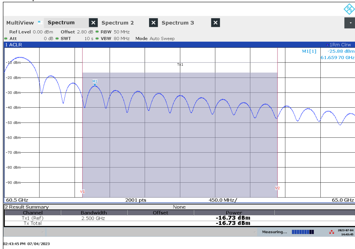
Plot 5: Channel power within 61.5 to 64 GHz with lens
