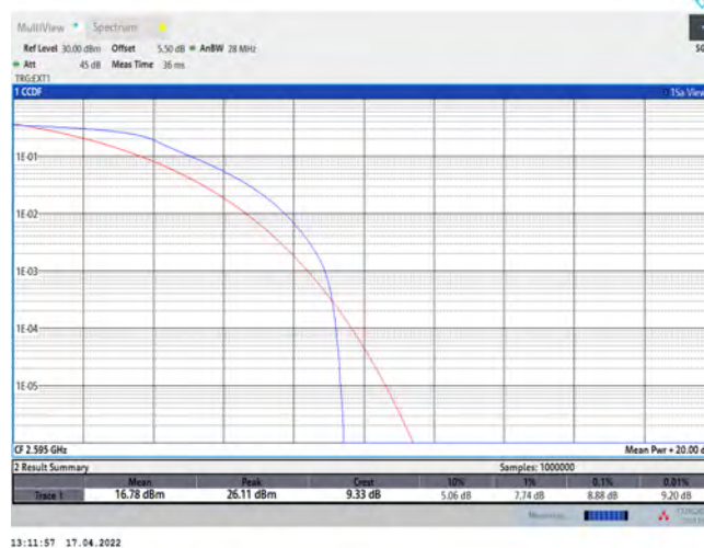
Band38-20MHz-QPSK-38000-100RB#0
