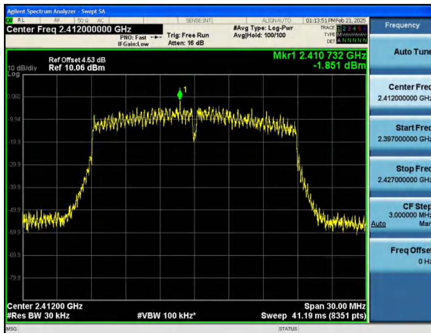
Power_Spectral_Density_NVNT_ANT2_802_11n(HT20)_2412
