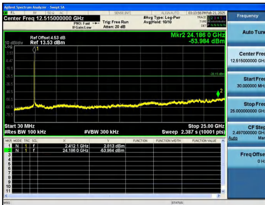
2_Spurious_Emission_NVNT_MIMO_802_11ax(HE20)_2412
