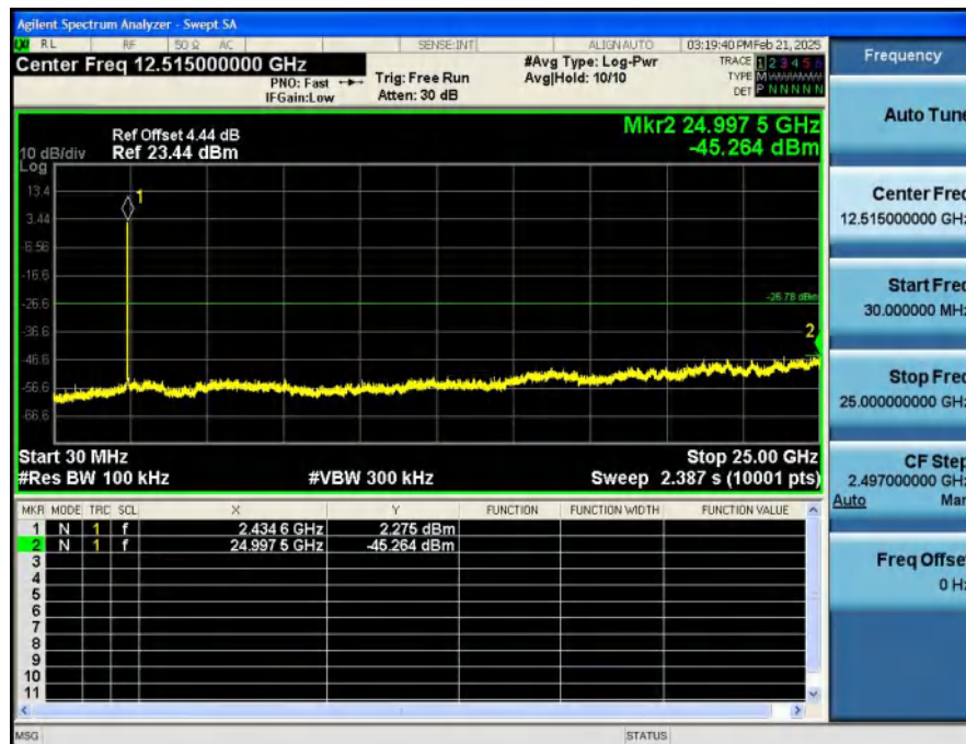
2_Spurious_Emission_NVNT_MIMO_802_11ax(HE20)_2437
