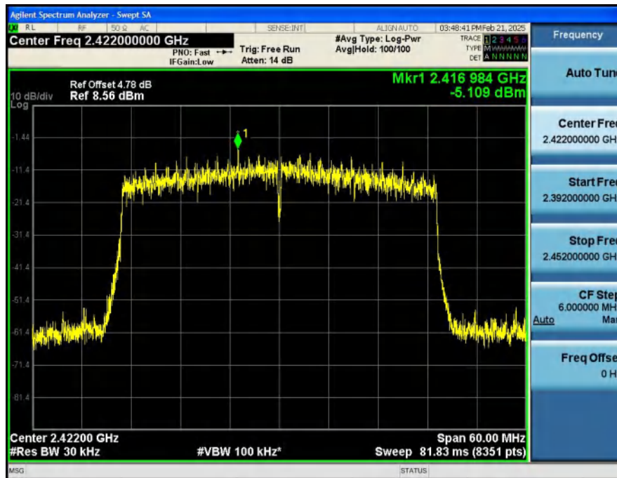
Power_Spectral_Density_NVNT_ANT2_802_11ax(HE40)_2422
