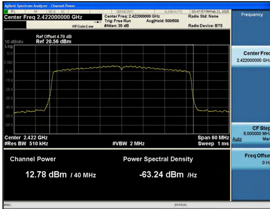
MAX__Output_Power_NVNT_ANT2_802_11ax(HE40)_2422
