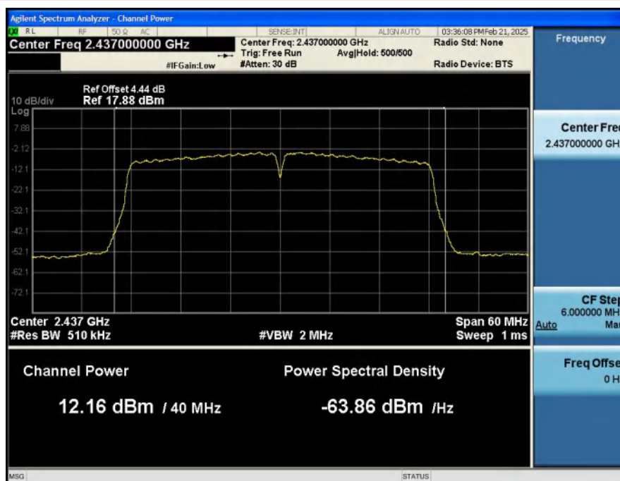
MAX__Output_Power_NVNT_ANT2_802_11n(HT40)_2437
