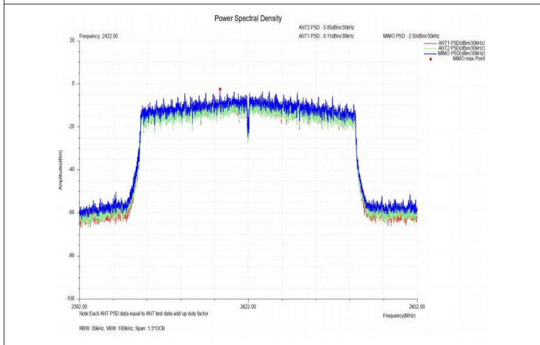
NVNT_MIMO_TX_802_11ax(HE40)_Power_Spectral_Density_2422
