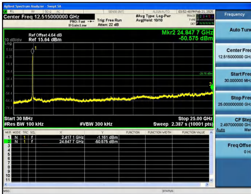
2_Spurious_Emission_NVNT_MIMO_802_11ax(HE40)_2422
