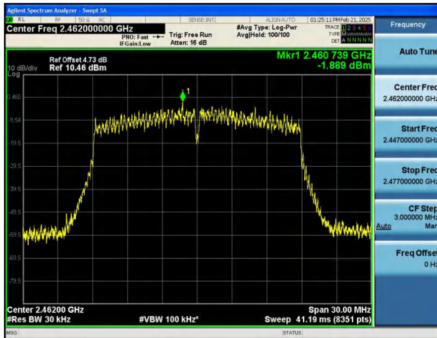
Power_Spectral_Density_NVNT_ANT2_802_11n(HT20)_2462
