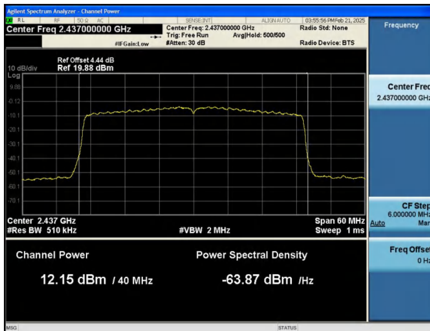
MAX__Output_Power_NVNT_ANT2_802_11ax(HE40)_2437
