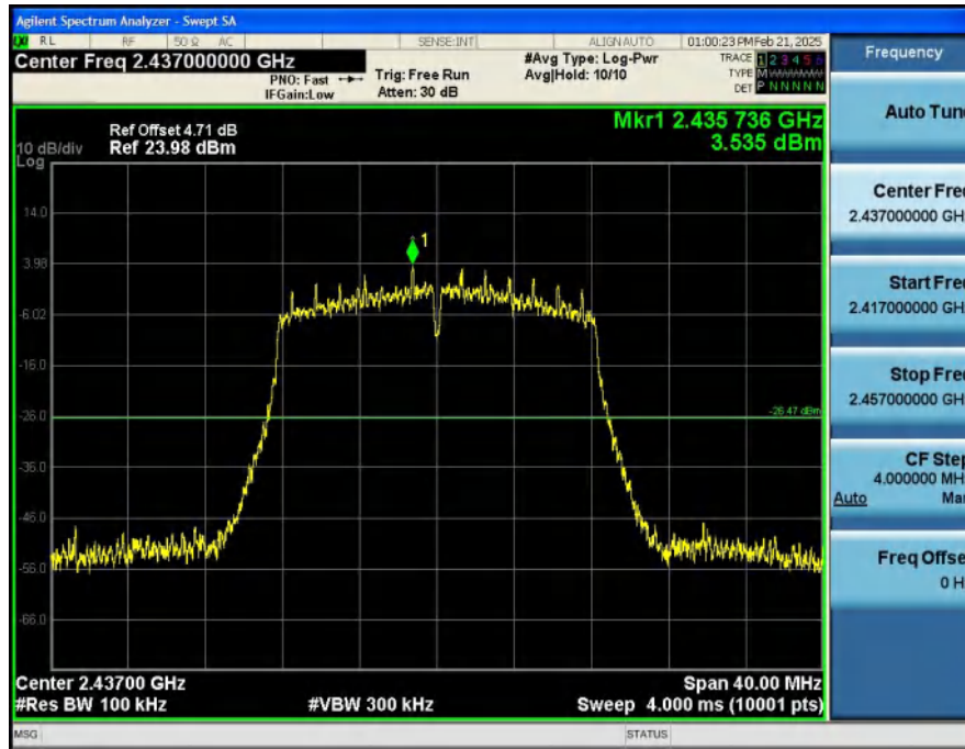
1_Reference_Level_NVNT_ANT2_802_11g_2437
