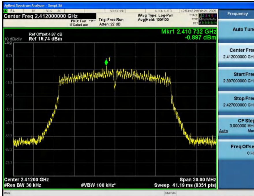
Power_Spectral_Density_NVNT_ANT2_802_11g_2412
