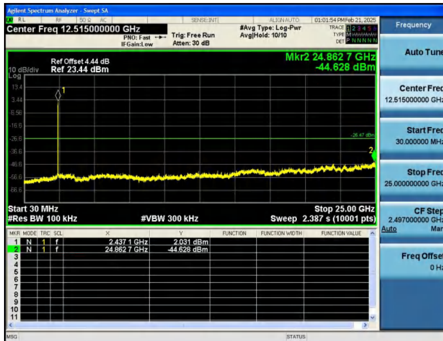
2_Spurious_Emission_NVNT_ANT2_802_11g_2437
