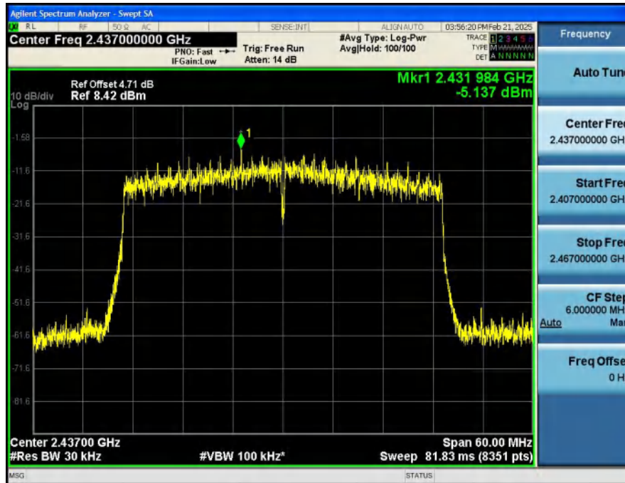
Power_Spectral_Density_NVNT_ANT2_802_11ax(HE40)_2437
