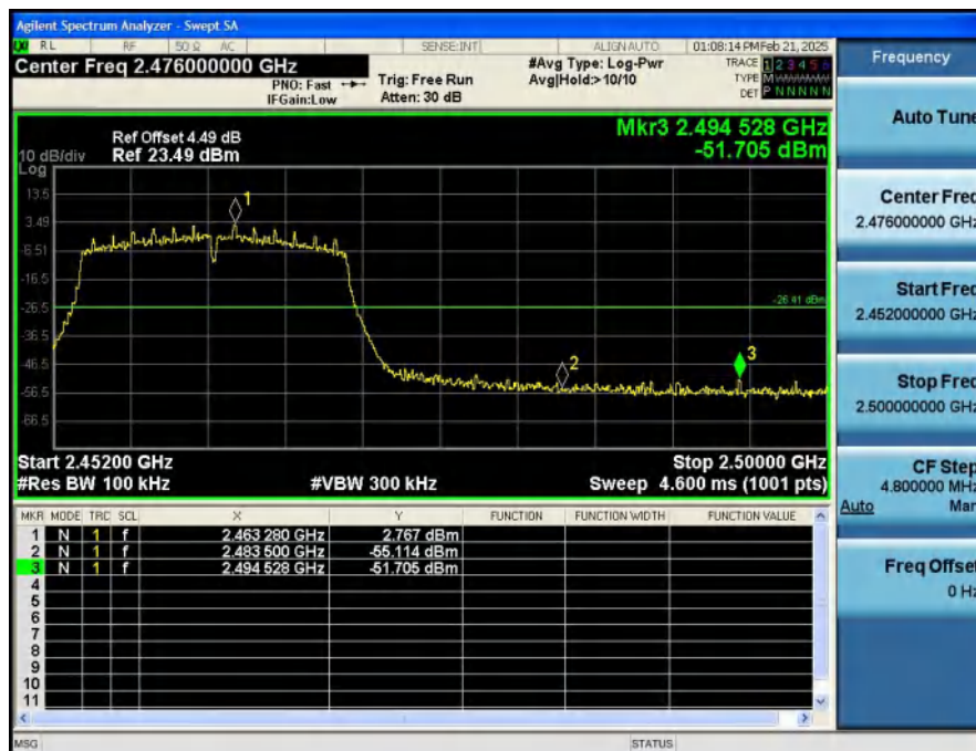
2_Bandedge_NVNT_ANT2_802_11g_2462
