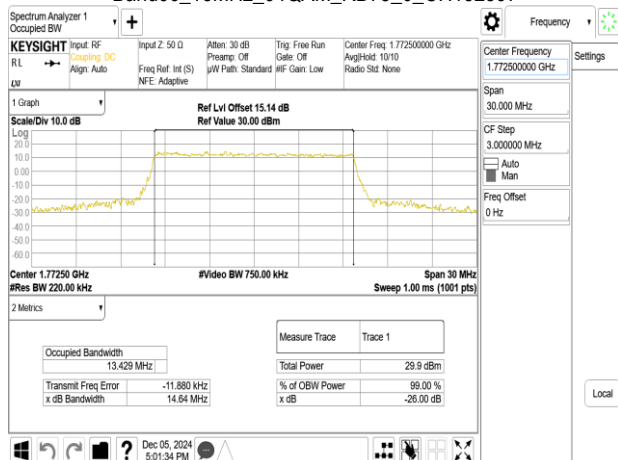
Band66_15MHz_256QAM_RB75_0_CH132597
