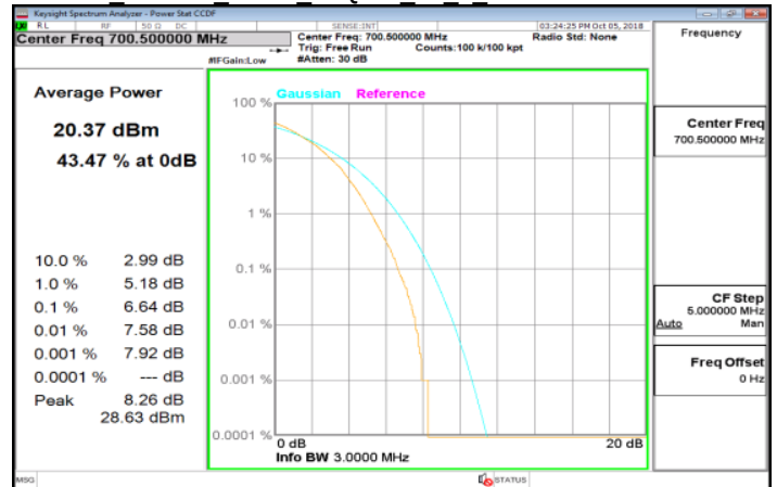
LTE Band12 3MHz 64QAM 15 0 LowCH23025-700.5
