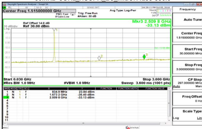
30MHz~3GHz_HSUPA_B5_MidCH4183-836.6
