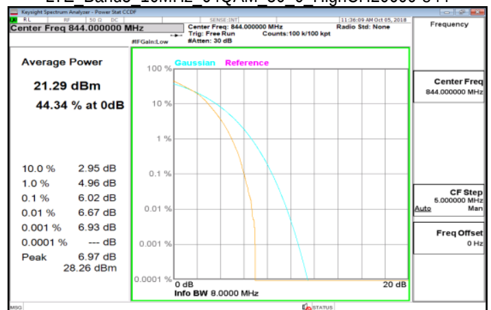
LTE Band5 10MHz 64QAM 50 0 HighCH20600-844
