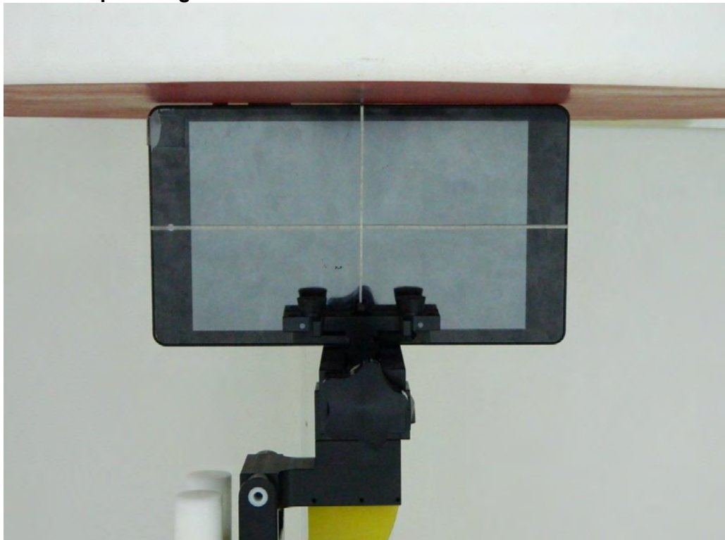
Photograph 6: Set-up for Edge 2 of NS-P08A7100
