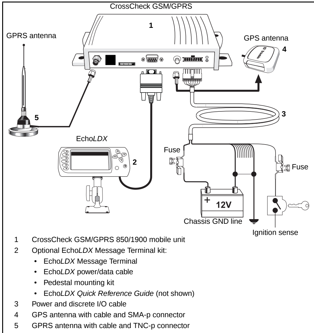
Figure 1.1 CrossCheck GSM/GPRS system components
