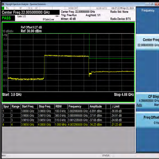
NTNV-N77-3700-3980-PC2-30-100-H-CP-QPSK-Outer_Full-Ant3-PASS
