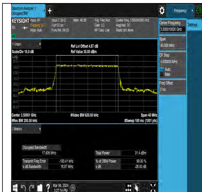
NTNV-N78-3450-3550-PC2-30-20-M-DFT-PI2BPSK-Outer_Full-Ant5-PASS
