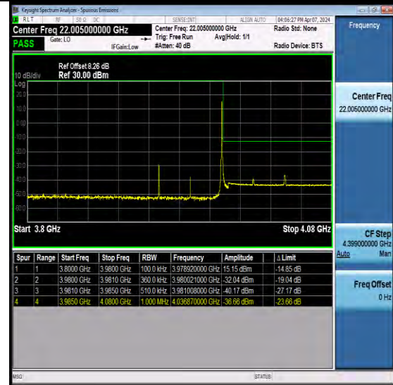
NTNV-N77-3700-3980-PC2-30-60-H-CP-QPSK-Edge_1RB_ Right-Ant5-PASS
