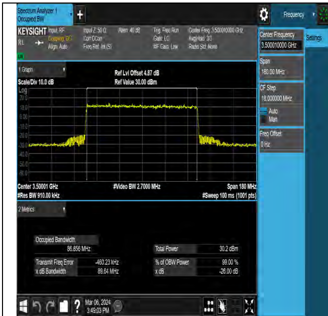
NTNV-N78-3450-3550-PC2-30-90-M-DFT-16QAM-Outer_Ful I-Ant5-PASS
