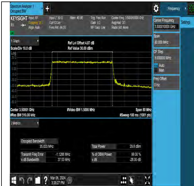
NTNV-N78-3450-3550-PC2-30-40-M-DFT-16QAM-Outer_Full-Ant5-PASS
