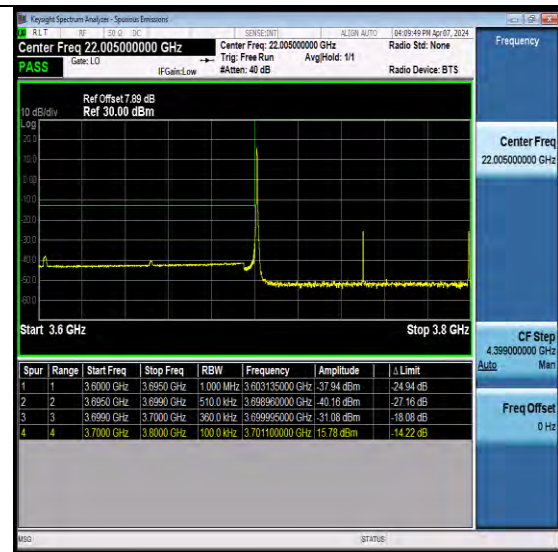
NTNV-N77-3700-3980-PC2-30-100-L-CP-QPSK-Edge_1RB_Left-Ant5-PASS
