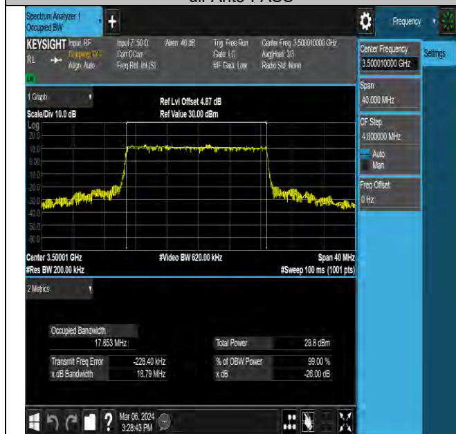
NTNV-N78-3450-3550-PC2-30-20-M-DFT-16QAM-Outer_Full-Ant5-PASS
