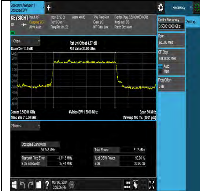
NTNV-N78-3450-3550-PC2-30-40-M-DFT-PI2BPSK-Outer_Full-Ant5-PASS
