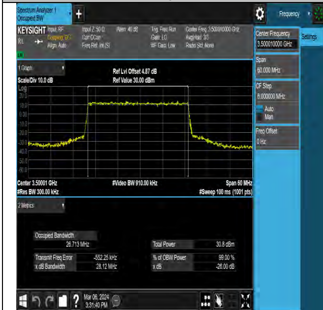
NTNV-N78-3450-3550-PC2-30-30-M-DFT-QPSK-Outter_Ful Ant5-PASS
