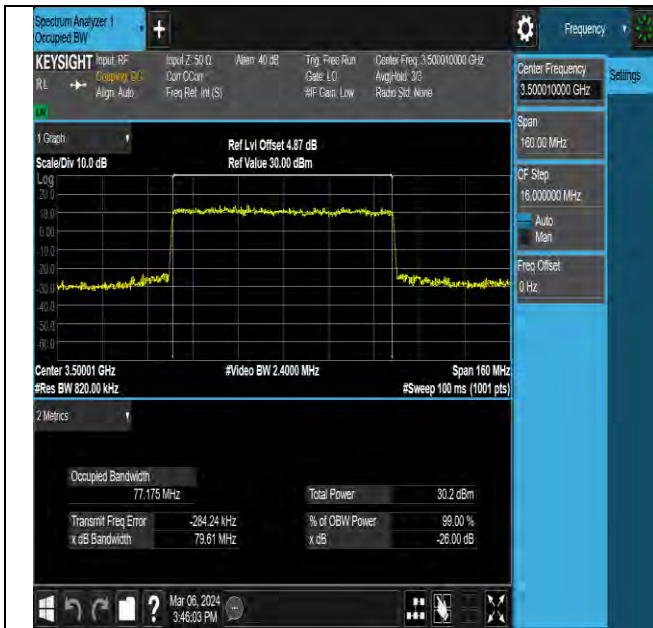
NTNV-N78-3450-3550-PC2-30-80-M-DFT-64QAM-Outer_Full-Ant5-PASS
