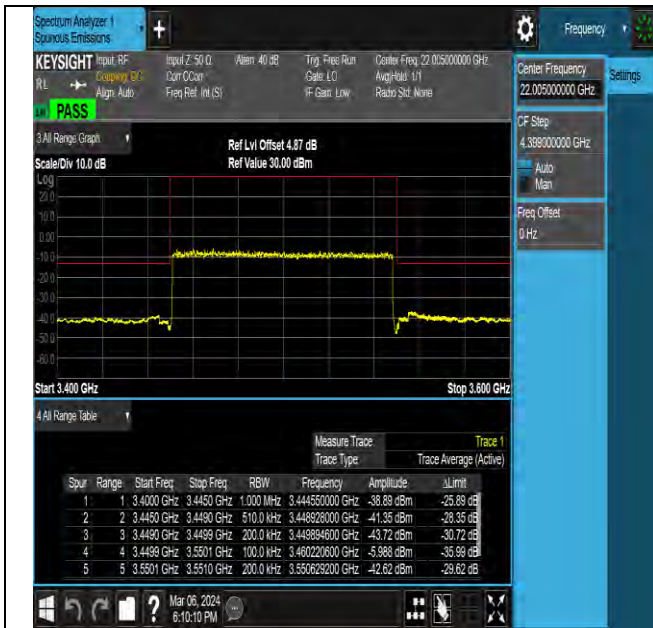
NTNV-N78-3450-3550-PC2-30-100-M-DFT-QPSK-Outer_Ful I-Ant5-PASS
