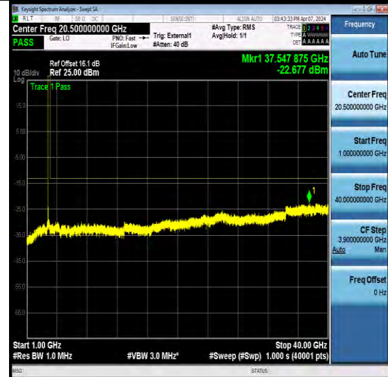
NTNV-N77-3700-3980-PC2-30-60-L-CP-QPSK-Edge_1RB_L eft-Ant3-PASS
