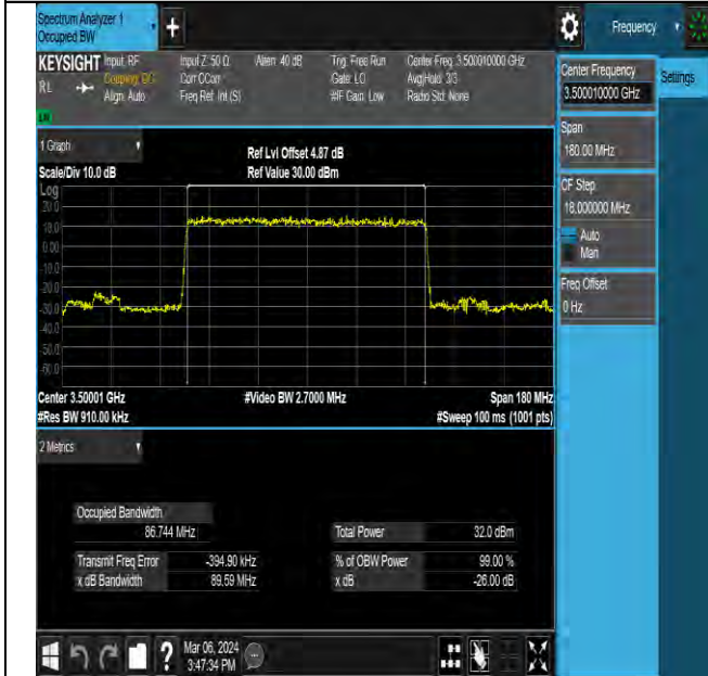
NTNV-N78-3450-3550-PC2-30-90-M-DFT-PI2BPSK-Outer_Full-Ant5-PASS
