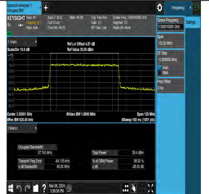
NTNV-N78-3450-3550-PC2-30-60-M-DFT-256QAM-Outter_Full-Ant5-PASS
