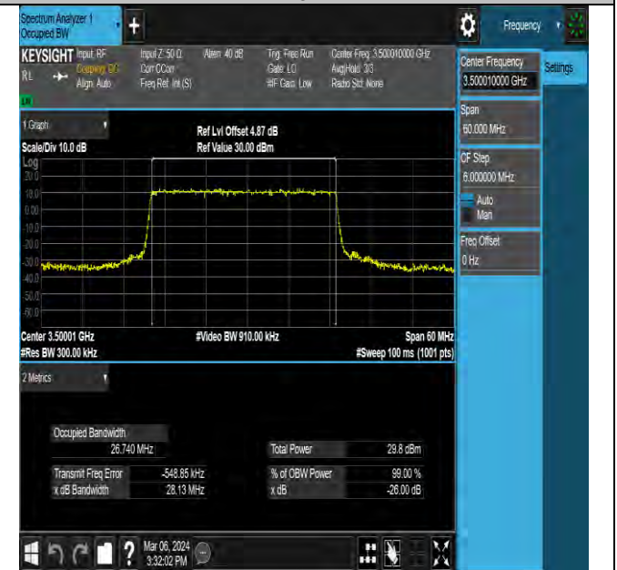
NTNV-N78-3450-3550-PC2-30-30-M-DFT-16QAM-Outter_Ful I-Ant5-PASS
