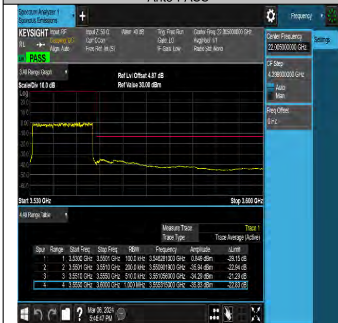
NTNV-N78-3450-3550-PC2-30-20-H-DFT-QPSK-Outer_Full-Ant5-PASS
