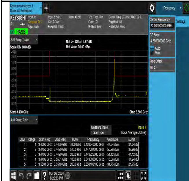
NTNV-N78-3450-3550-PC2-30-100-M-DFT-QPSK-Edge_1R B Right-Ant5-PASS
