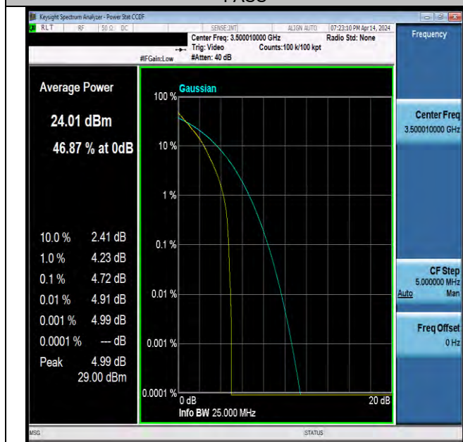
NTNV-N78-3450-3550-PC2-30-20-M-DFT-QPSK-Outer_Full-PASS
