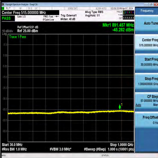
NTNV-N77-3700-3980-PC2-30-100-M-CP-QPSK-Edge_1RB Left-Ant3-PASS
