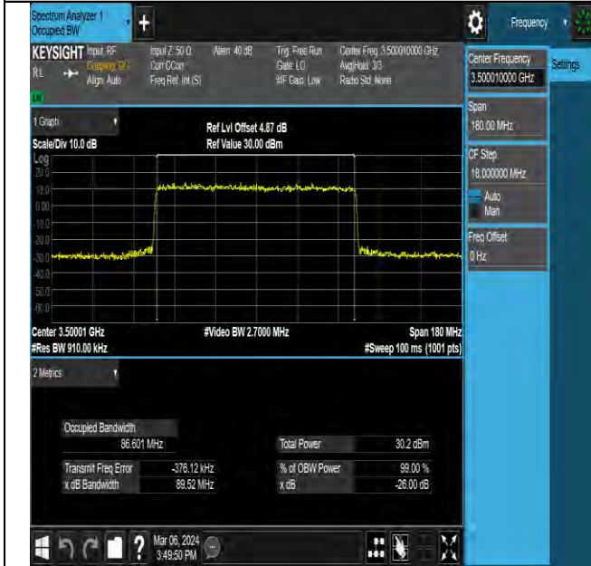
NTNV-N78-3450-3550-PC2-30-90-M-DFT-256QAM-Outer_Full-Ant5-PASS
