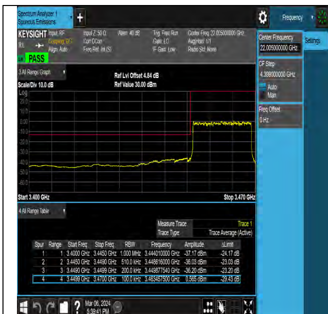
NTNV-N78-3450-3550-PC2-30-20-L-DFT-QPSK-Outer_Full-Ant5-PASS
