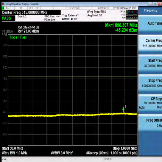
NTNV-N77-3700-3980-PC2-30-60-L-CP-QPSK-Edge_1RB_L eft-Ant3-PASS
