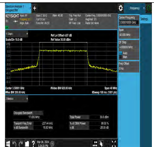
NTNV-N78-3450-3550-PC2-30-20-M-DFT-QPSK-Outer_Full-Ant5-PASS
