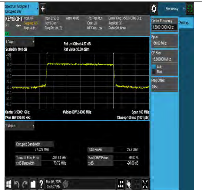
NTNV-N78-3450-3550-PC2-30-80-M-DFT-256QAM-Outer_Full-Ant5-PASS
