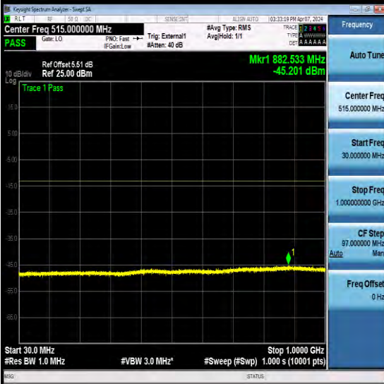
NTNV-N77-3700-3980-PC2-30-100-M-CP-QPSK-Edge_1RB Left-Ant5-PASS
