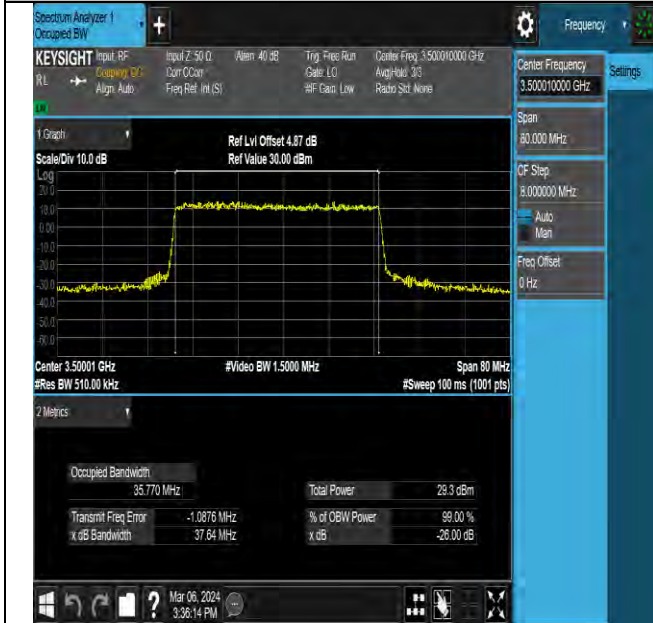
NTNV-N78-3450-3550-PC2-30-40-M-DFT-256QAM-Outer_Full-Ant5-PASS
