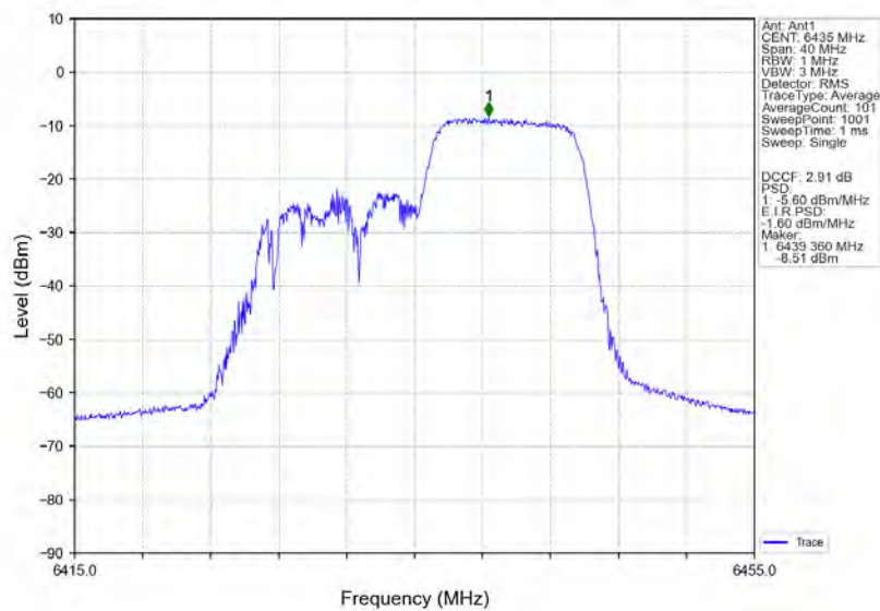
802.11ax(HE20)_LCH_6435MHz_RU106_Right_Ant1_NTNV
