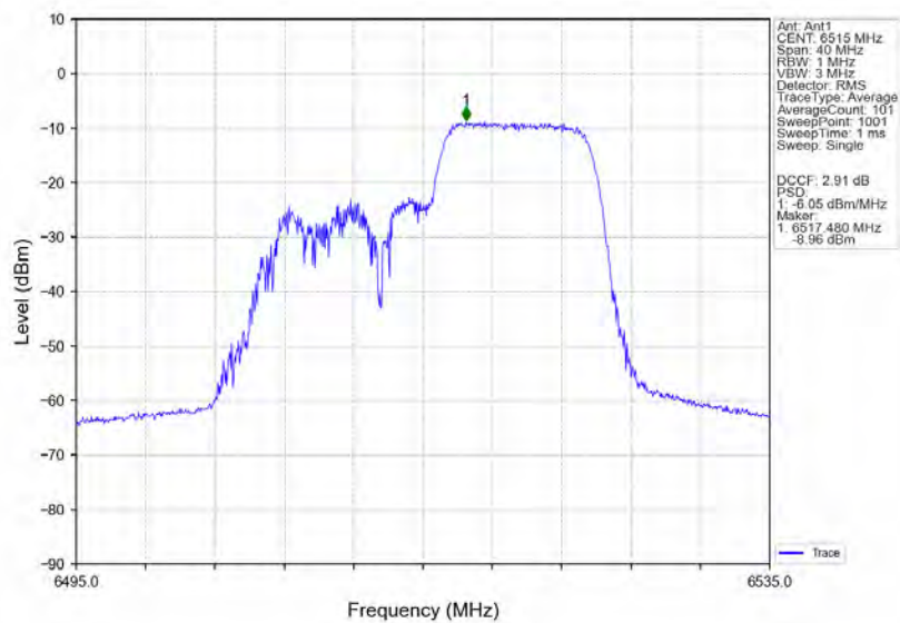
802.11ax(HE20)_HCH_6515MHz_RU106_Right_Ant1_NTNV
