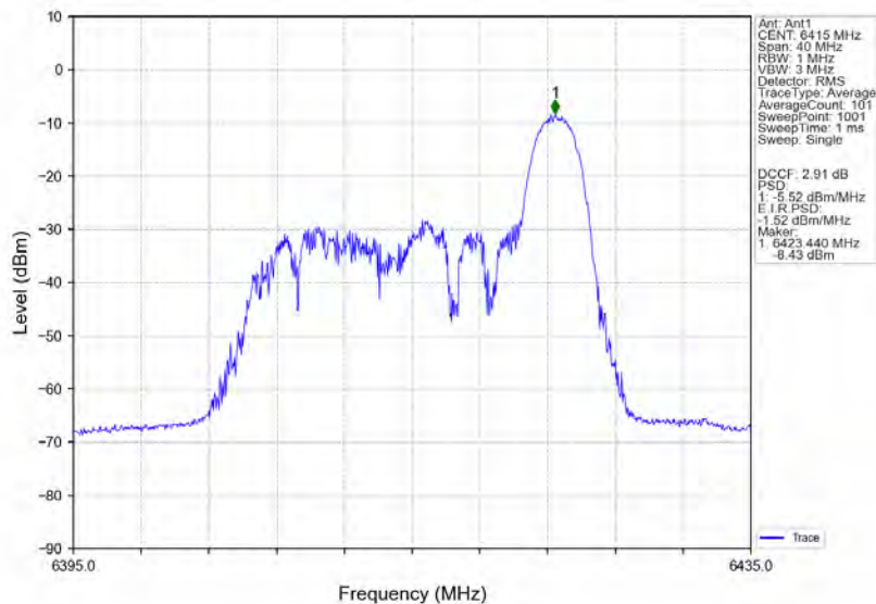
802.11ax(HE20) HCH_6415MHz_RU26_Right_Ant1_NTNV
