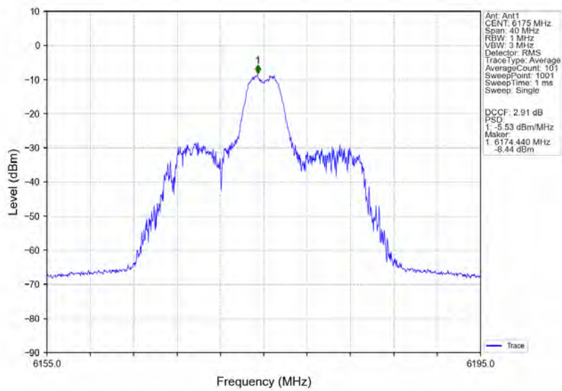
802.11ax(HE20)_MCH_6175MHz_RU26_Right_Ant1_NTNV
