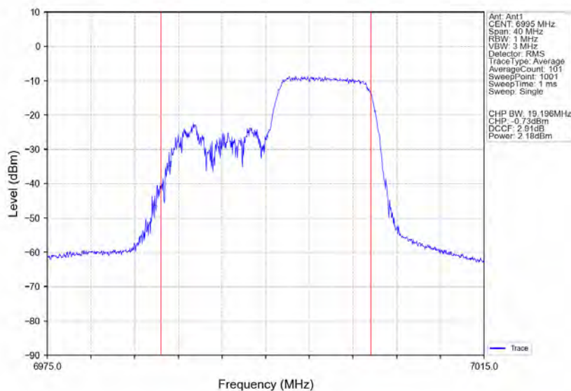
802.11ax(HE20)_MCH_6995MHz_RU106_Right_Ant1_NTNV
