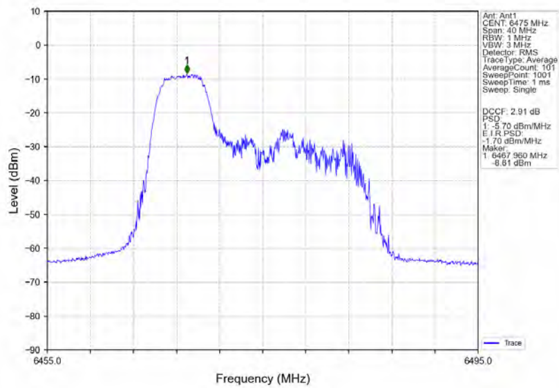
802.11ax(HE20)_MCH_6475MHz_RU52_Right_Ant1_NTNV
