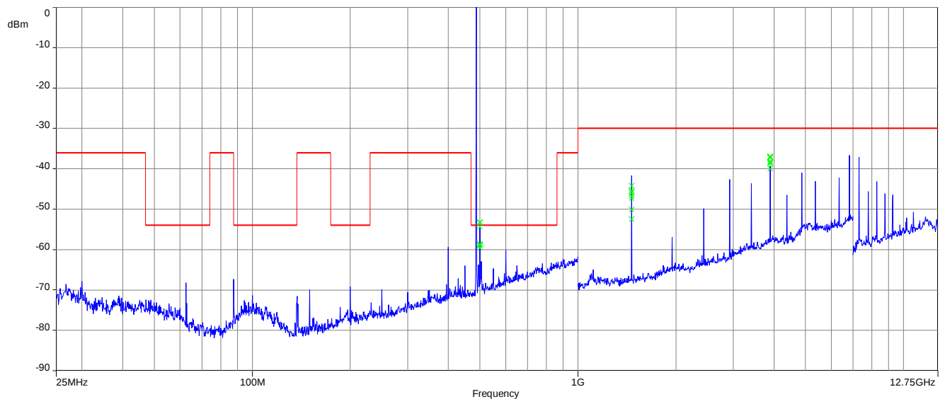
Plot 1: 487.125 MHz, spurious emissions, 25 MHz – 12.75 GHz
