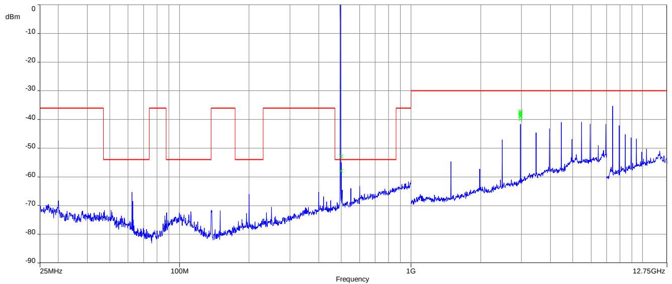
Plot 2: 495.375 MHz, spurious emissions, 25 MHz – 12.75 GHz
