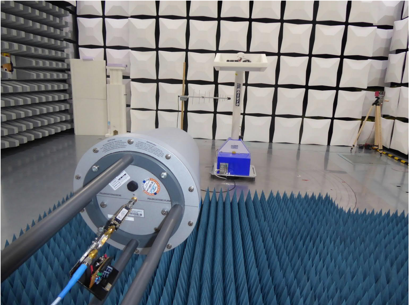
Test setup from 4 to 18 GHz
