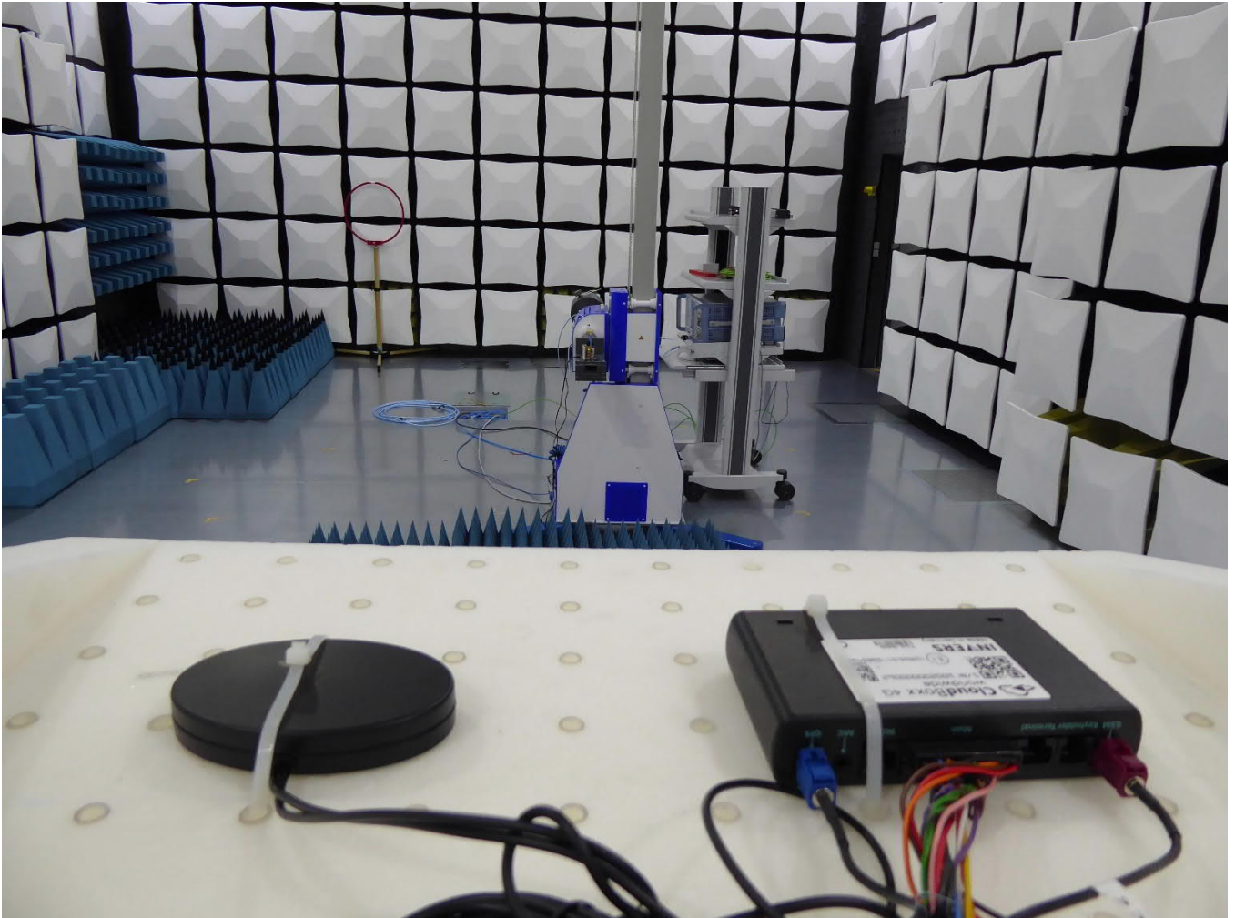
Test setup from 18 to 26.5 GHz
