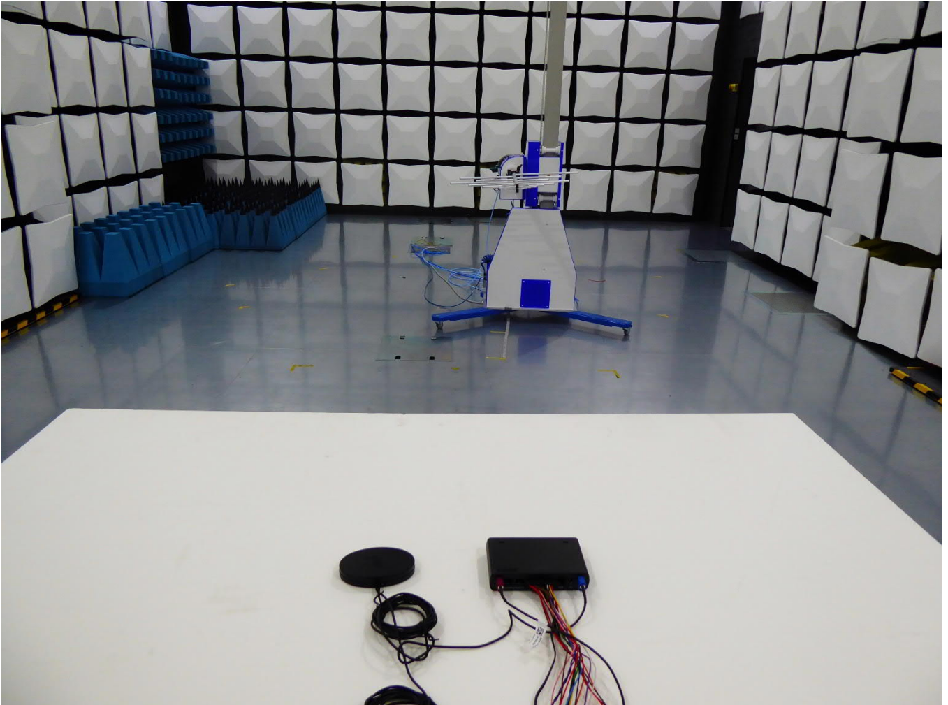
Test setup from 200 to 1000 MHz
