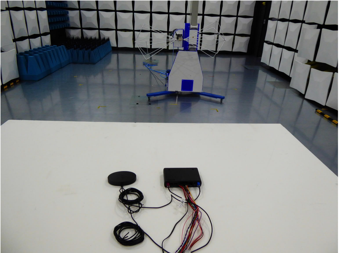
Test setup from 30 to 200 MHz
