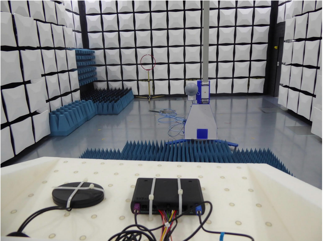
Test setup from 1 to 4 GHz
