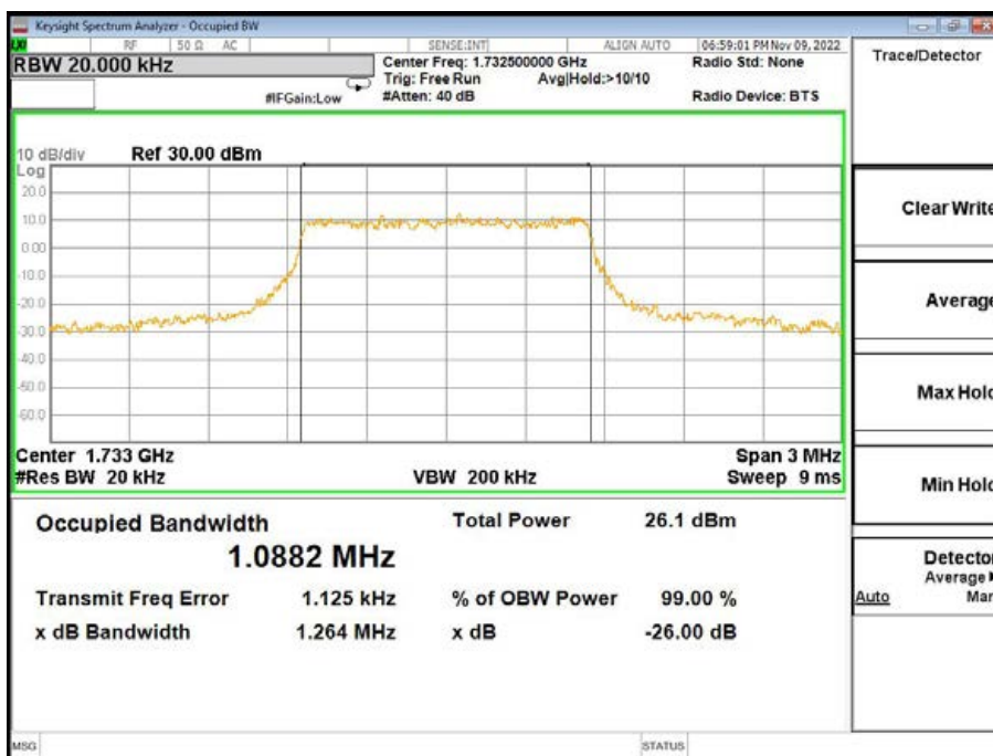
Band4-1.4MHz Bandwidth-QPSK
