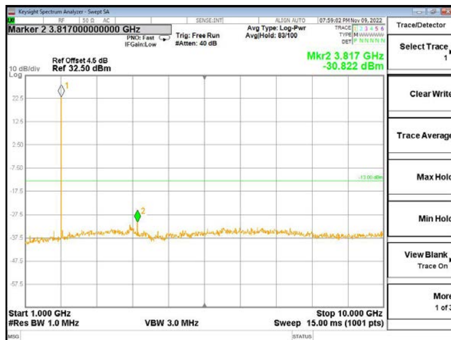
Band2-High Channel-1.4MHz Bandwidth-1RB-QPSK-1GHz to 10GHz
