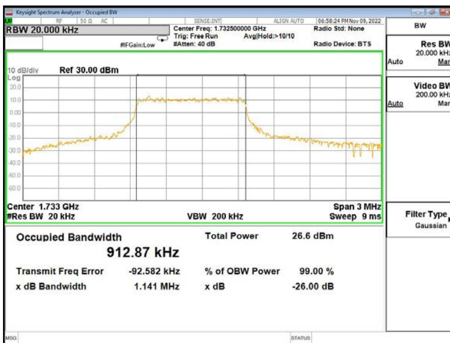
Band4-1.4MHz Bandwidth-16QAM
