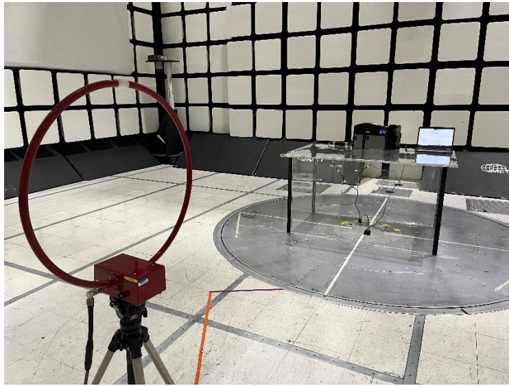
Photograph 3. Spurious Emissions Below 30 MHz, Test Setup Front View
