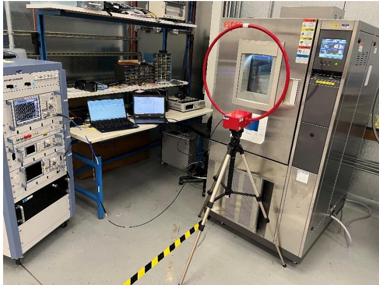
Photograph 6. Frequency Stability Test Setup
