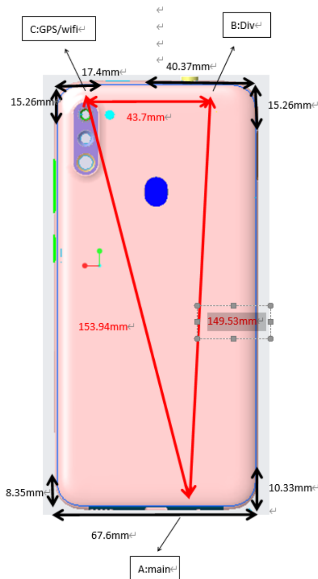
Picture 12.1 Antenna Locations
