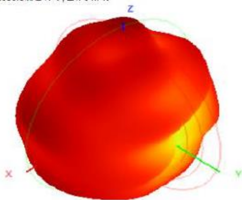
2500.0MHz H+V, Eff: 64.7%
