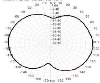
Total(H-XY), Max= 0.21dBi, CirD=16.76
