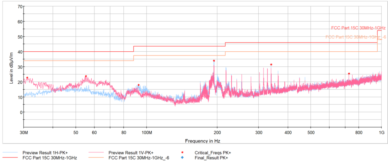
Plot 7-53. Radiated Spurious Emissions Below 1GHz (4Mbps, – Ch.73 with AC/DC Adapter and USB-C cable)
