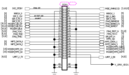
Debug connector
