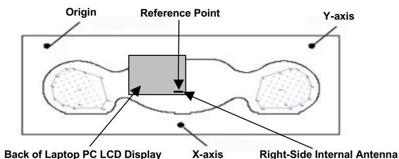
Figure 3. Phantom Reference Point & EUT Positioning Back Top Right Side of LCD Display (Closed)- Right-Side Antenna
