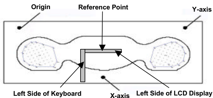
Figure 5. Phantom Reference Point & EUT Positioning Left Side of Laptop PC LCD Display (Open) - Left-Side Antenna
