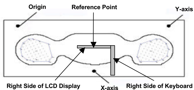
Figure 4. Phantom Reference Point & EUT Positioning Right Side of Laptop PC LCD Display (Open) - Right-Side Antenna
