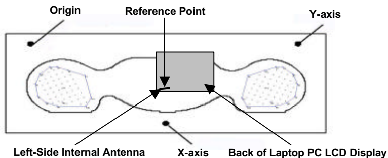
Figure 2. Phantom Reference Point & EUT Positioning Back Top Left Side of LCD Display (Closed)- Left-Side Antenna
