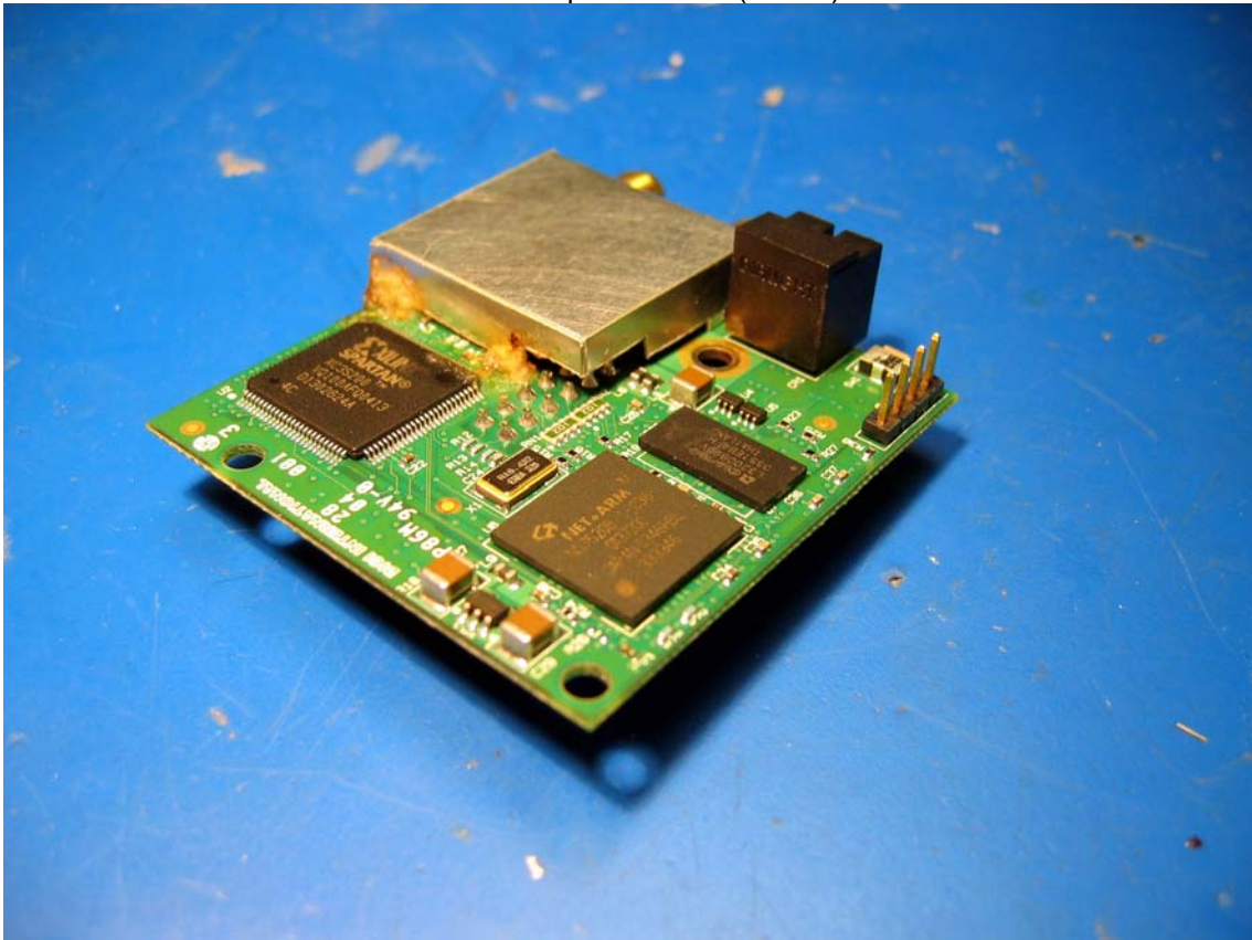
Wi-EM - Top with shield (open)
