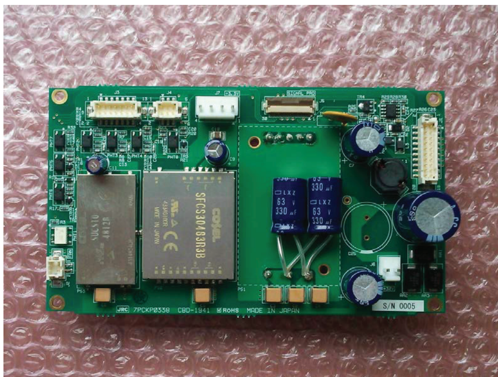
PS I/F CIRCUIT Top view
