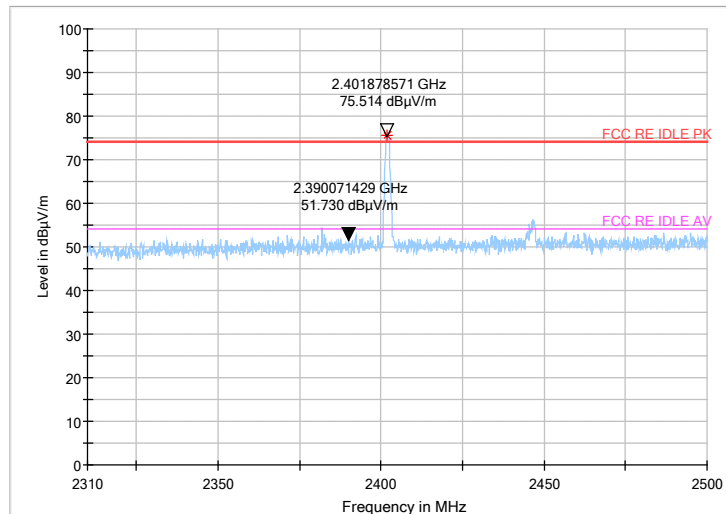
Peak Detector
