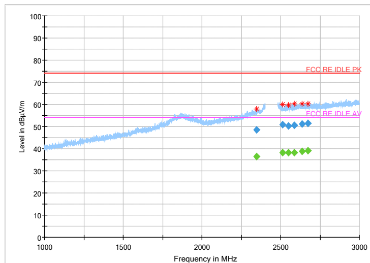
Fig.2 Radiated emission: Ch39, 1GHz~3GHz
