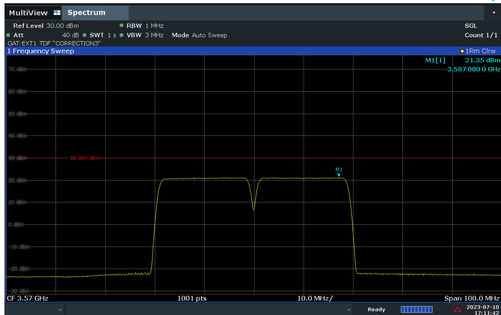
Plot 7.92. Peak Power Spectral Density Measurement (40MHz BW, Low Channel, 256-QAM)
