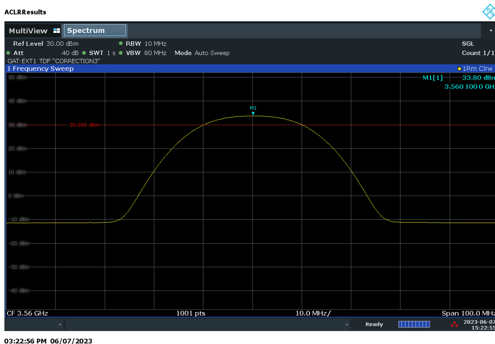
Plot 7.62. Conducted Power / 10MHz Measurement (20MHz BW, Low Channel, 16-QAM)
