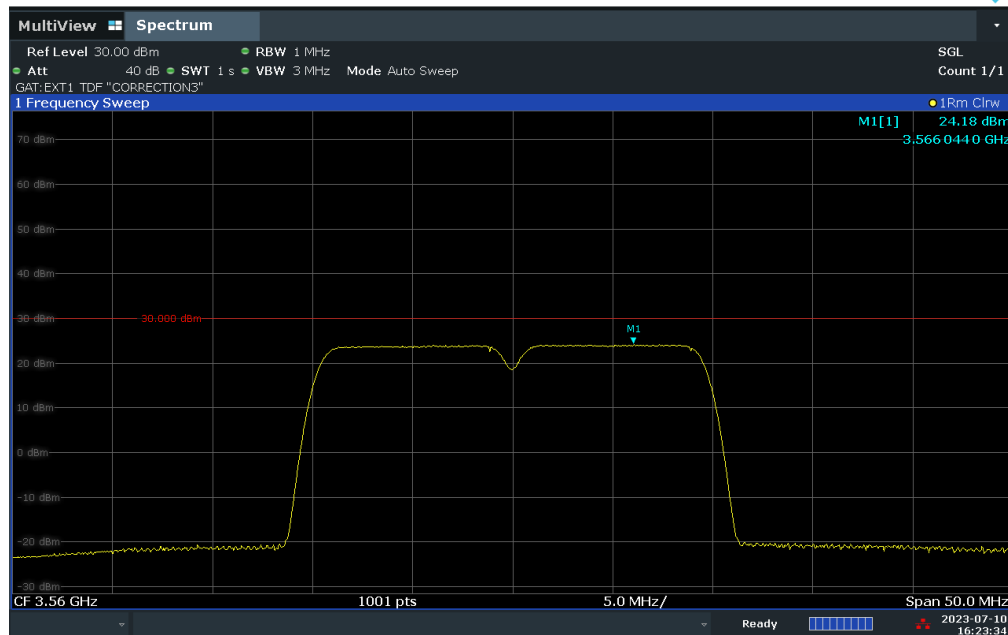
Plot 7.100. Peak Power Spectral Density Measurement (20MHz BW, Low Channel, 256-QAM)
