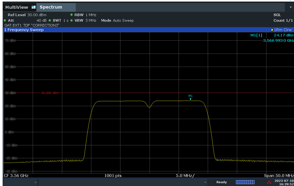
Plot 7.99. Peak Power Spectral Density Measurement (20MHz BW, Low Channel, 64-QAM)
