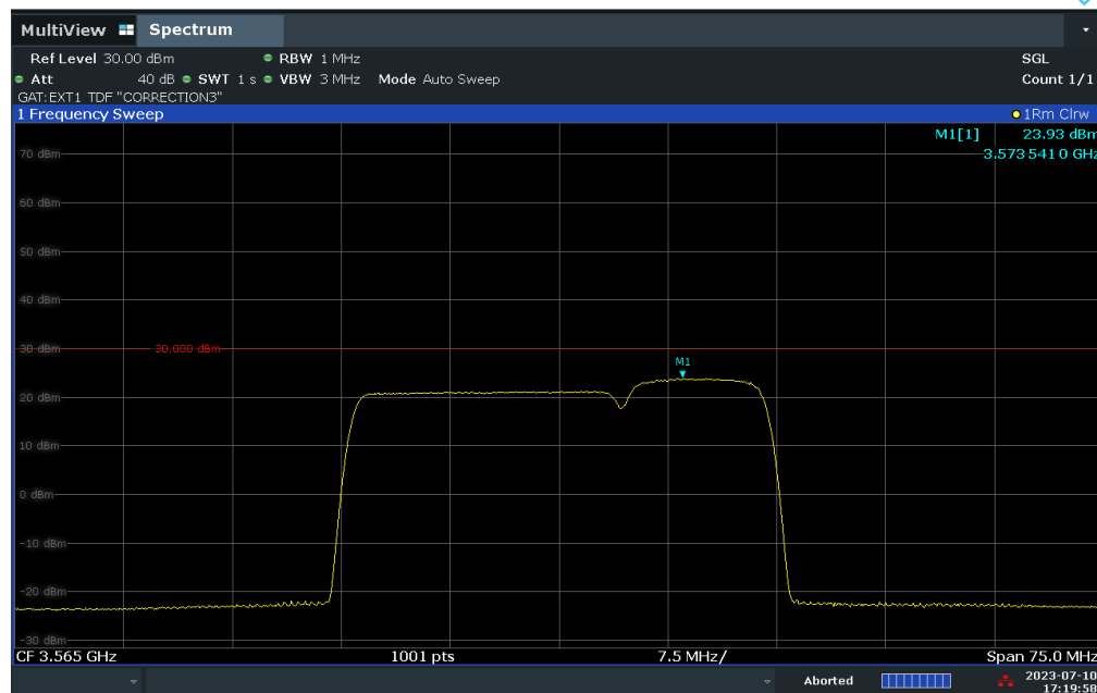
Plot 7.94. Peak Power Spectral Density Measurement (30MHz BW, Low Channel, 16-QAM)
