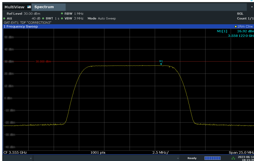
Plot 7.88. Peak Power Spectral Density Measurement (10MHz BW, Low Channel, 256-QAM)
