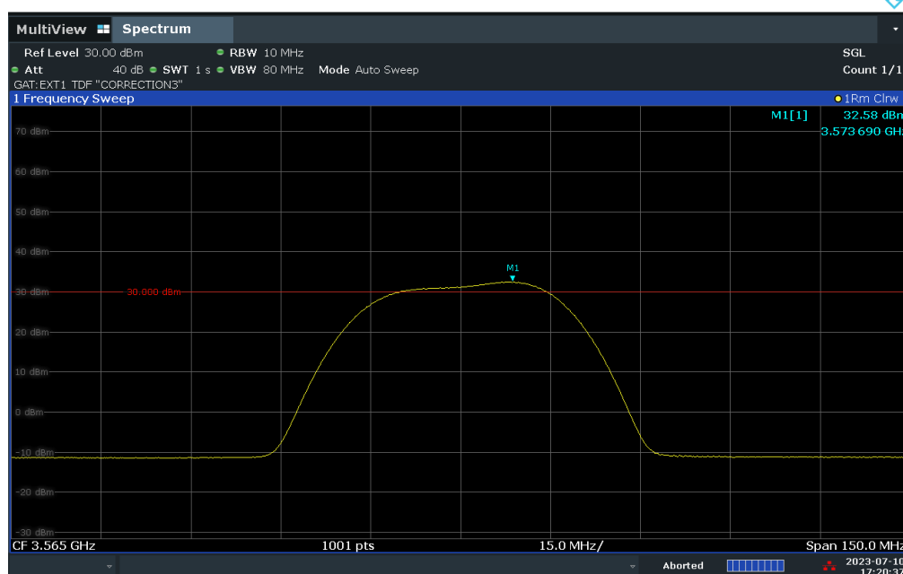
Plot 7.73. Conducted Power / 10MHz Measurement (30MHz BW, Low Channel, QPSK)
