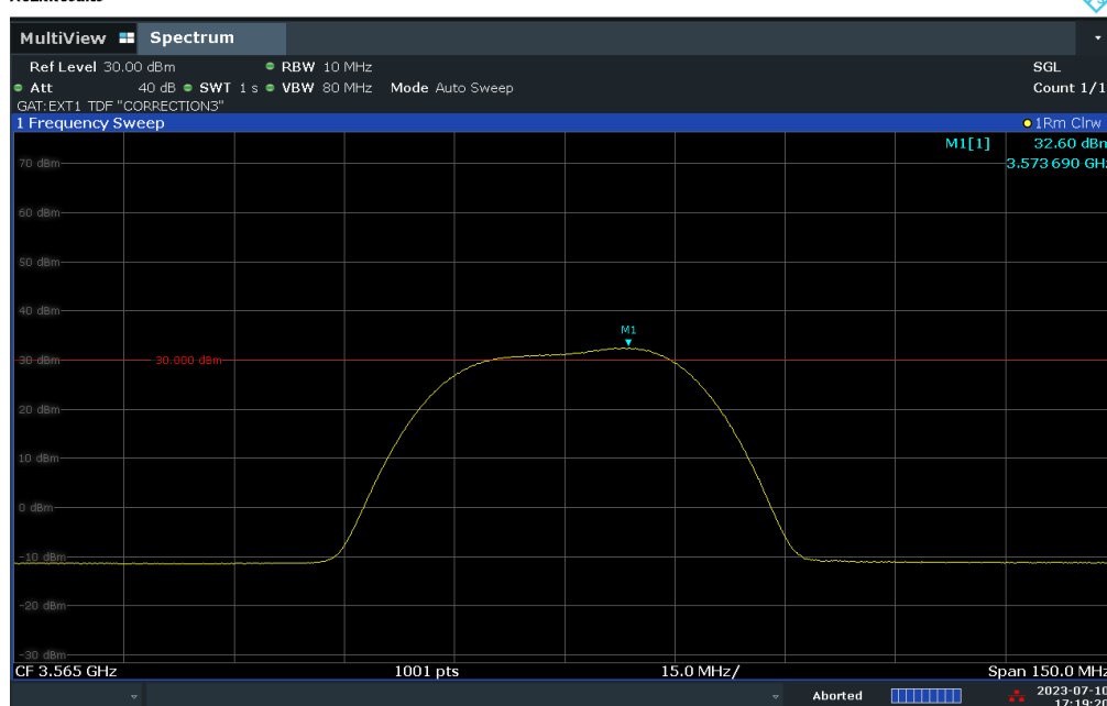
Plot 7.74. Conducted Power / 10MHz Measurement (30MHz BW, Low Channel, 16-QAM)
