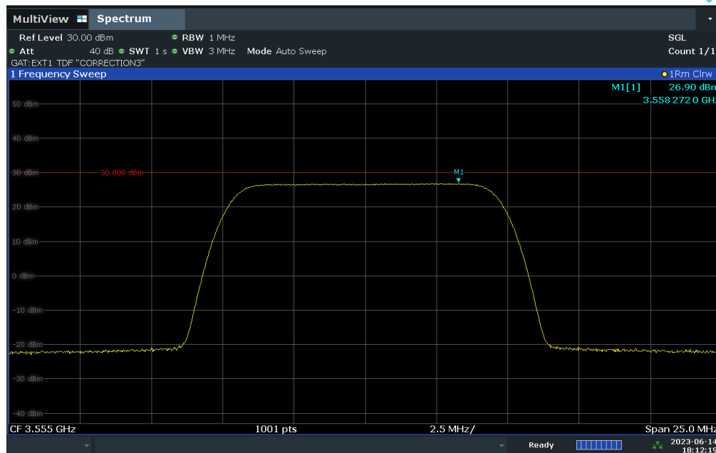
Plot 7.87. Peak Power Spectral Density Measurement (10MHz BW, Low Channel, 64-QAM)
