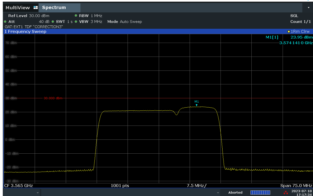
Plot 7.95. Peak Power Spectral Density Measurement (30MHz BW, Low Channel, 64-QAM)
