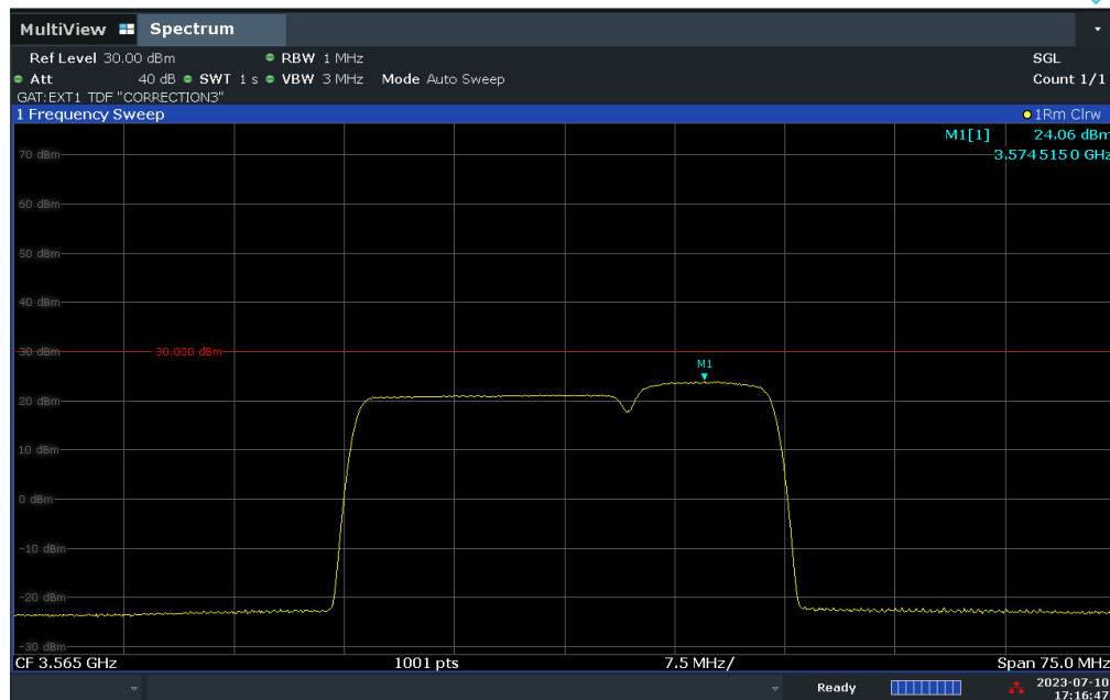
Plot 7.93. Peak Power Spectral Density Measurement (30MHz BW, Low Channel, QPSK)
