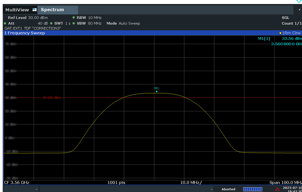
Plot 7.78. Conducted Power / 10MHz Measurement (20MHz BW, Low Channel, 16-QAM)
