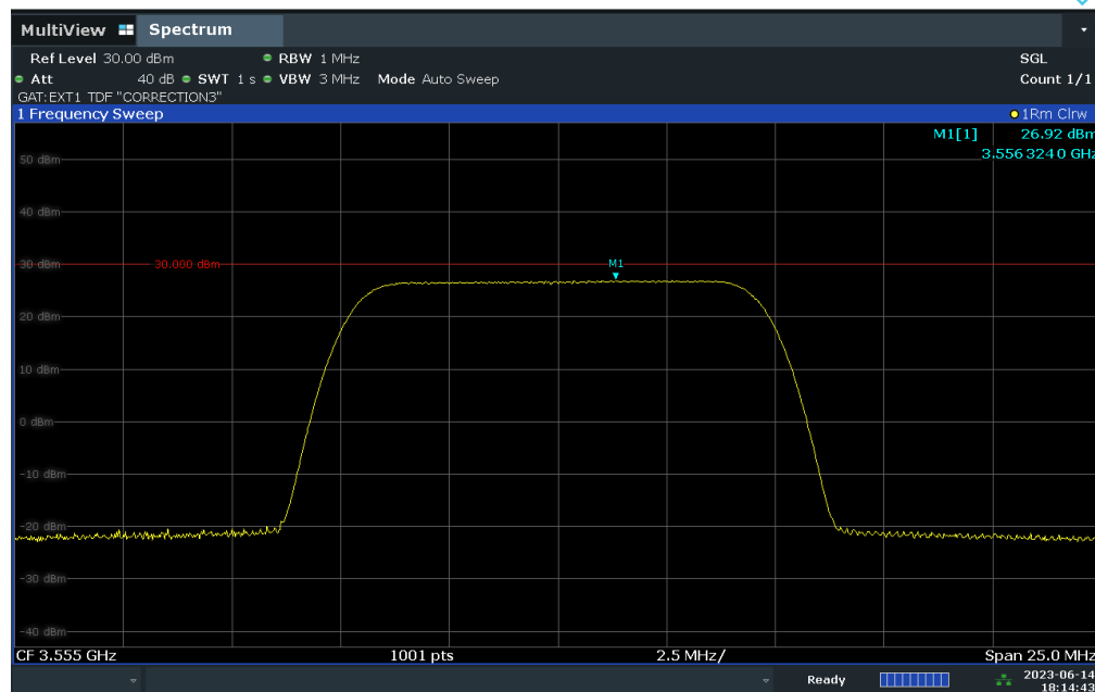
Plot 7.86. Peak Power Spectral Density Measurement (10MHz BW, Low Channel, 16-QAM)
