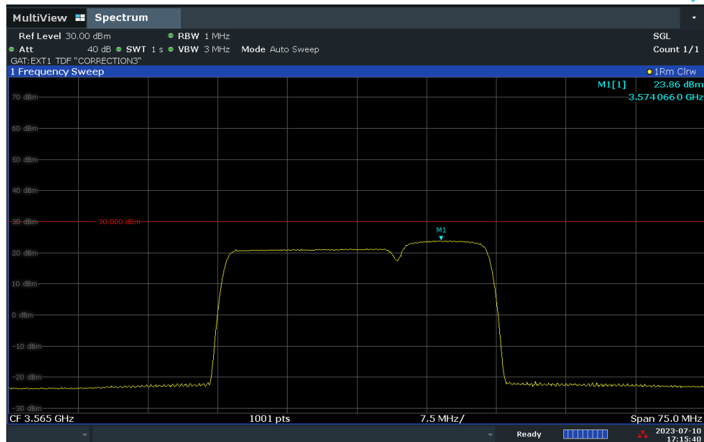
Plot 7.96. Peak Power Spectral Density Measurement (30MHz BW, Low Channel, 256-QAM)
