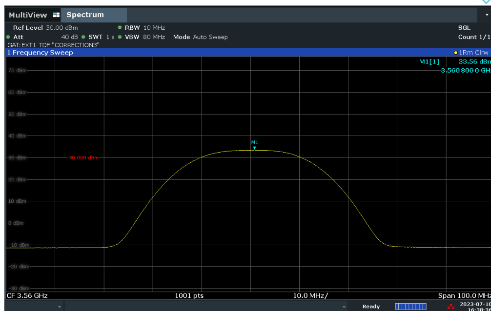
Plot 7.77. Conducted Power / 10MHz Measurement (20MHz BW, Low Channel, QPSK)
