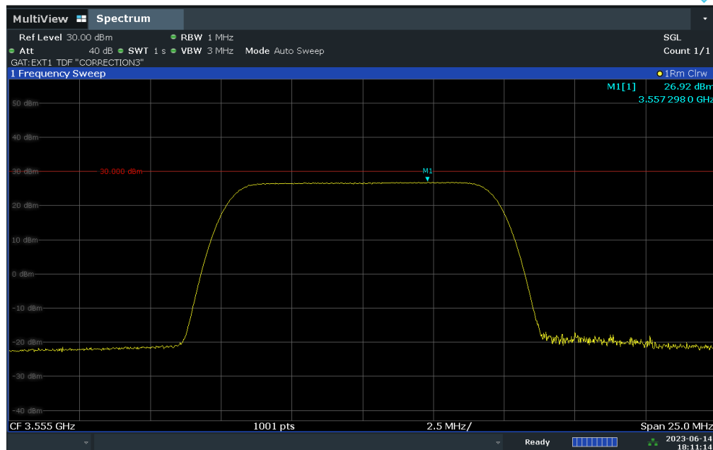
Plot 7.85. Peak Power Spectral Density Measurement (10MHz BW, Low Channel, QPSK)
