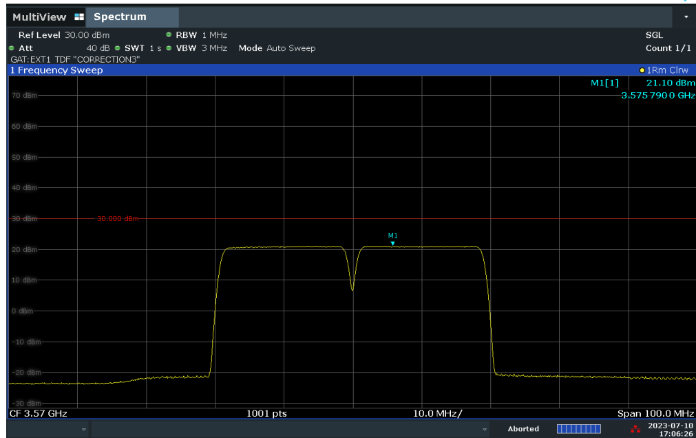
Plot 7.91. Peak Power Spectral Density Measurement (40MHz BW, Low Channel, 64-QAM)
