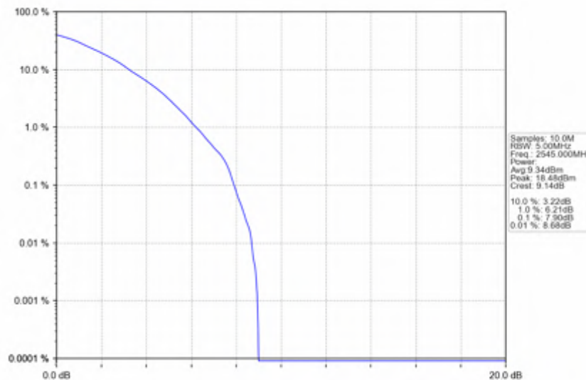
n7_15kHz_SISO_NTNV_50MHz_DFT-s-OFDM_256_QAM_2545MHz_Outer_Full
