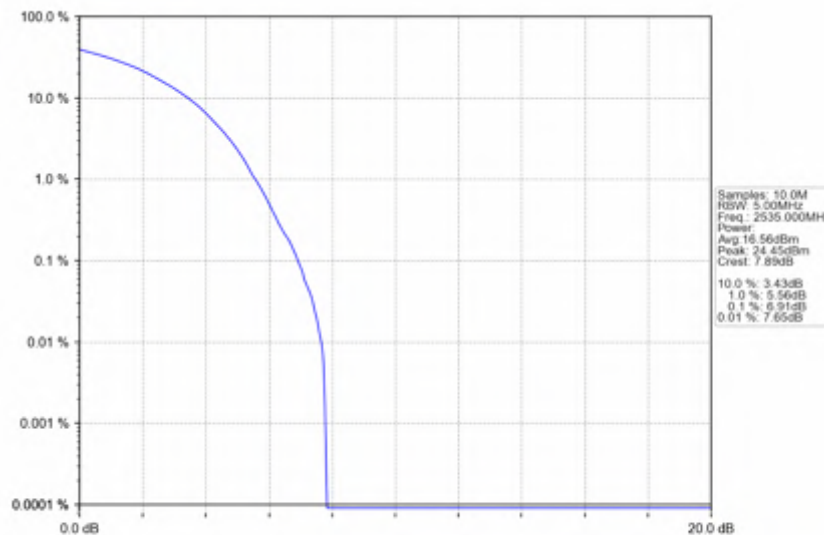
n7_15kHz_SISO_NTNV_10MHz_DFT-s-OFDM_256_QAM_2535MHz_Outer_Full
