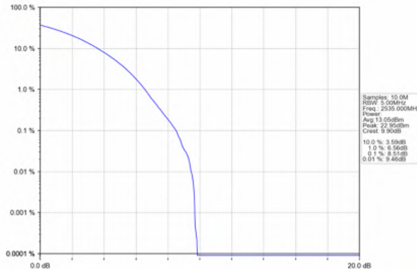
n7_15kHz_SISO_NTNV_30MHz_CP-OFDM_QPSK_2535MHz_Outer_Full
