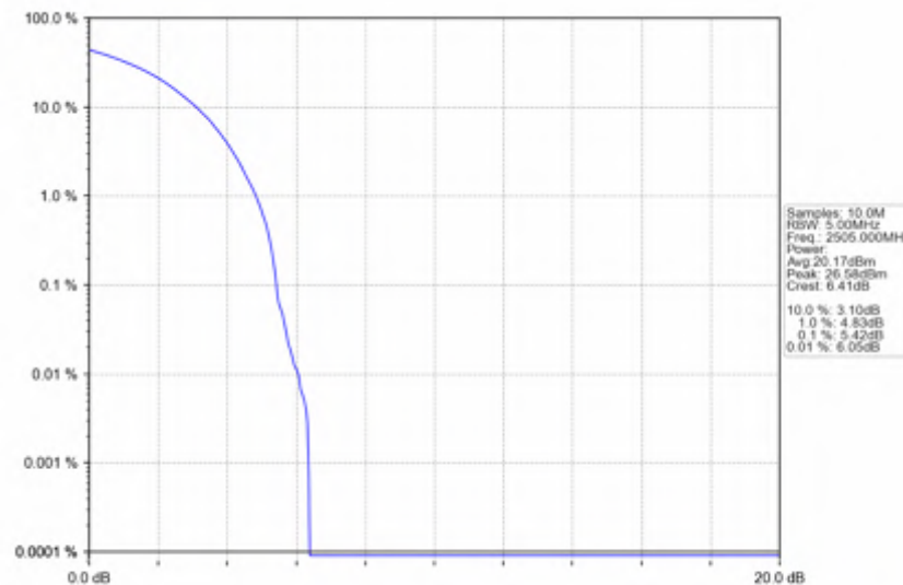
n7_15kHz_SISO_NTNV_10MHz_DFT-s-OFDM QPSK_2505MHz_Outer_Full
