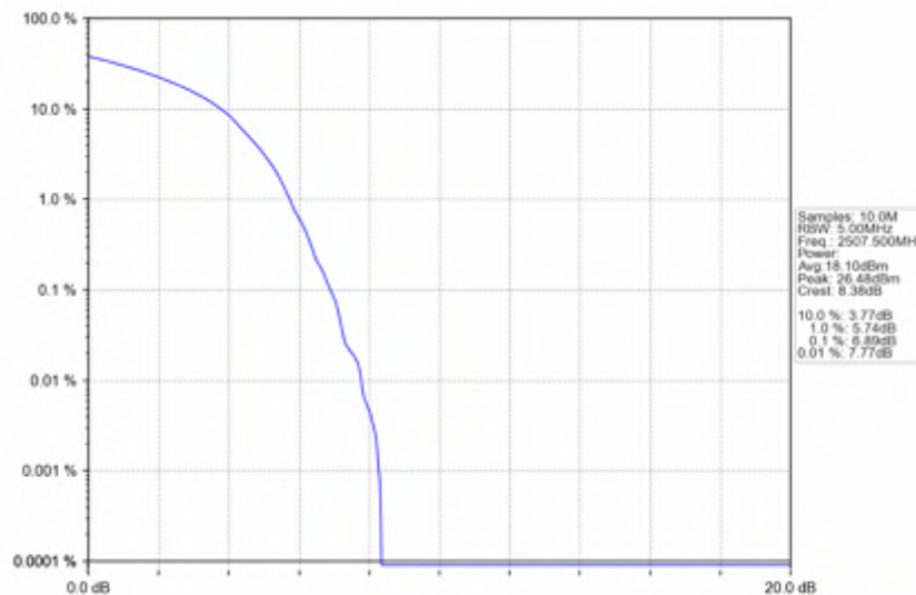
n7_30kHz_SISO_NTNV_15MHz_DFT-s-OFDM_16_QAM_2507.5MHz_Outer_Full
