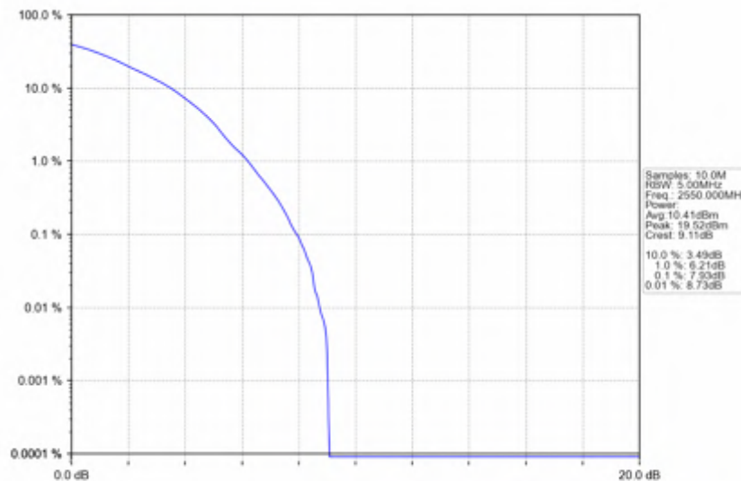
n7_15kHz_SISO_NTNV_40MHz_DFT-s-OFDM_256_QAM_2550MHz_Outer_Full
