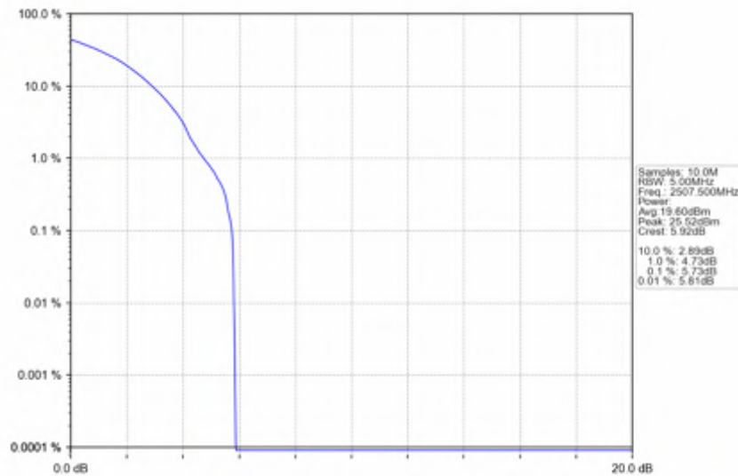
n7_30kHz_SISO_NTNV_15MHz_DFT-s-OFDM_PI/2_BPSK_2507.5MHz_Outer_Full
