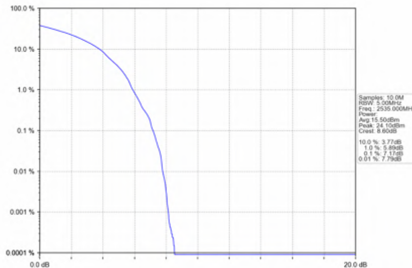
n7_30kHz_SISO_NTNV_15MHz_DFT-s-OFDM_256_QAM_2535MHz_Outer_Full
