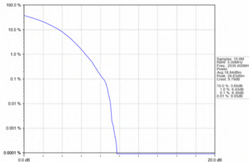
n7_30kHz_SISO_NTNV_10MHz_CP-OFDM_QPSK_2535MHz_Outer_Full
