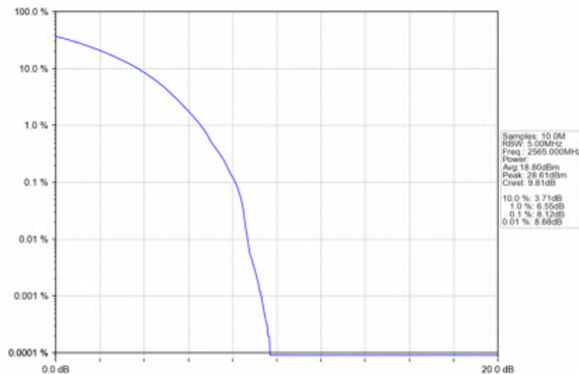
n7_30kHz_SISO_NTNV_10MHz_CP-OFDM 16 QAM_2565MHz_Outer_Full
