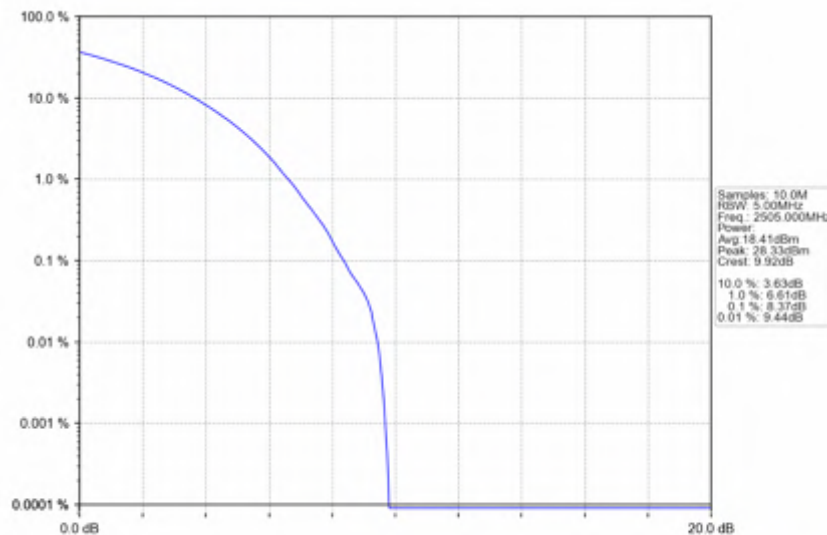
n7_30kHz_SISO_NTNV_10MHz_CP-OFDM 64 QAM_2505MHz_Outer_Full
