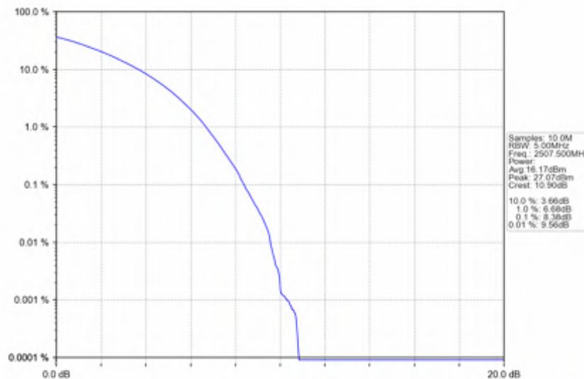
n7_15kHz_SISO_NTNV_15MHz_CP-OFDM QPSK_2507.5MHz_Outer_Full
