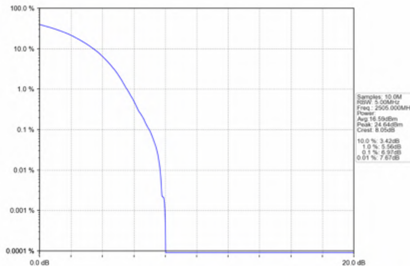
n7_15kHz_SISO_NTNV_10MHz_DFT-s-OFDM_256_QAM_2505MHz_Outer_Full
