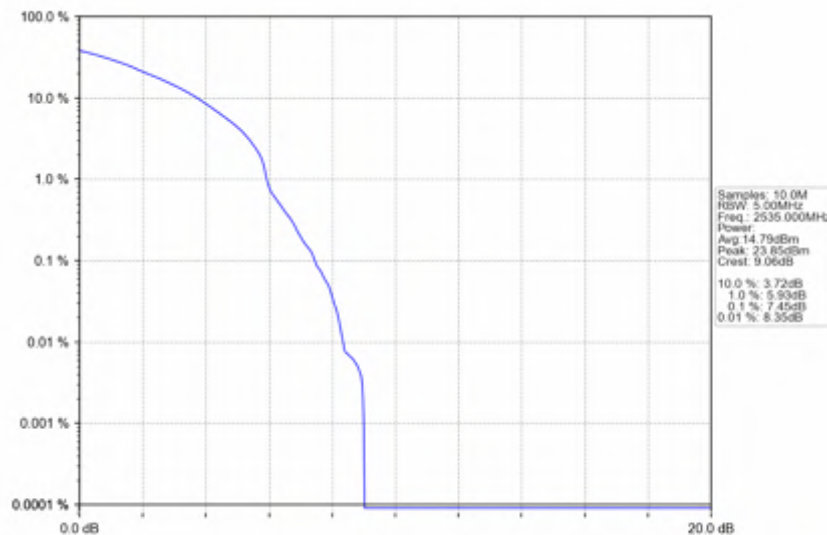
n7_15kHz_SISO_NTNV_15MHz_DFT-s-OFDM_256_QAM_2535MHz_Outer_Full
