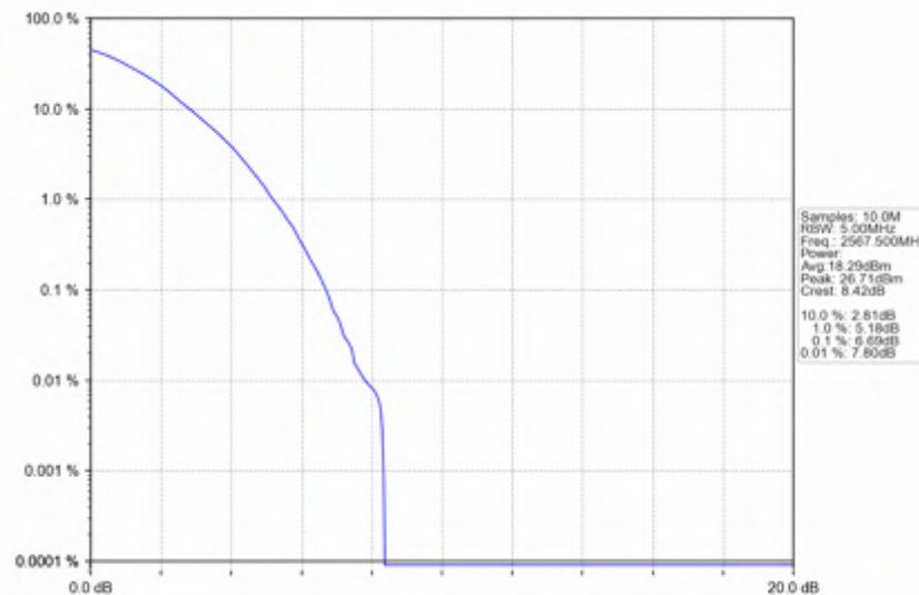
n7_15kHz_SISO_NTNV_5MHz_DFT-s-OFDM_256_QAM_2567.5MHz_Outer_Full
