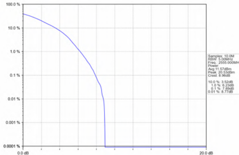
n7_15kHz_SISO_NTNV_30MHz_DFT-s-OFDM_256_QAM_2555MHz_Outer_Full
