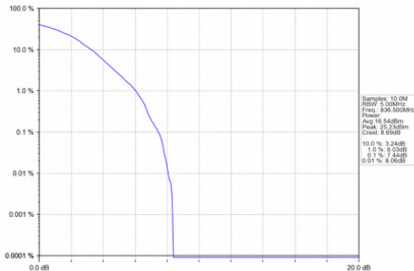
n5_30kHz_SISO_NTNV_20MHz_DFT-s-OFDM_16_QAM_836.5MHz_Outer_Full
