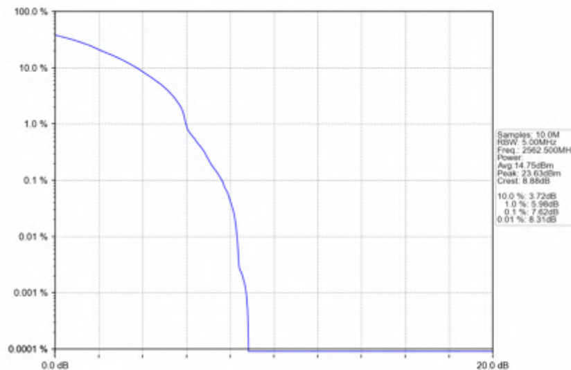
n7_15kHz_SISO_NTNV_15MHz_DFT-s-OFDM 256 QAM_2562.5MHz_Outer_Full
