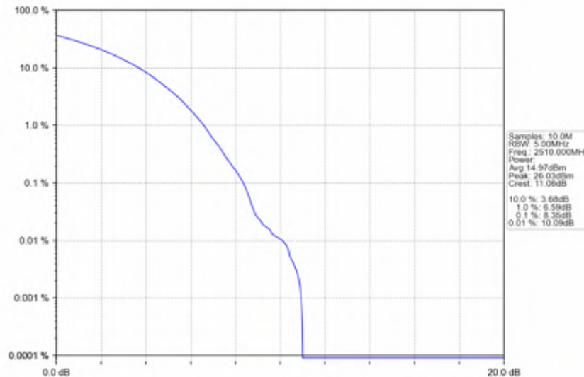
n7_15kHz_SISO_NTNV_20MHz_CP-OFDM_QPSK_2510MHz_Outer_Full
