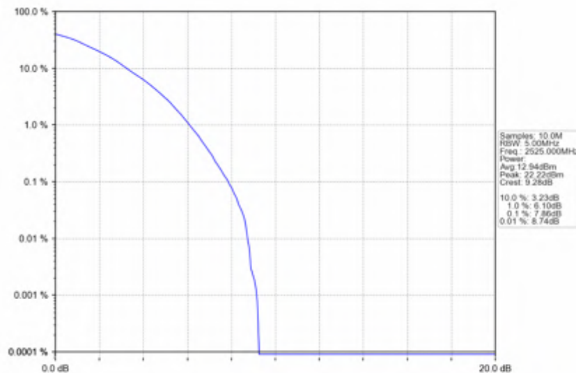
n7_15kHz_SISO_NTNV_50MHz_DFT-s-OFDM QPSK_2525MHz_Outer_Full
