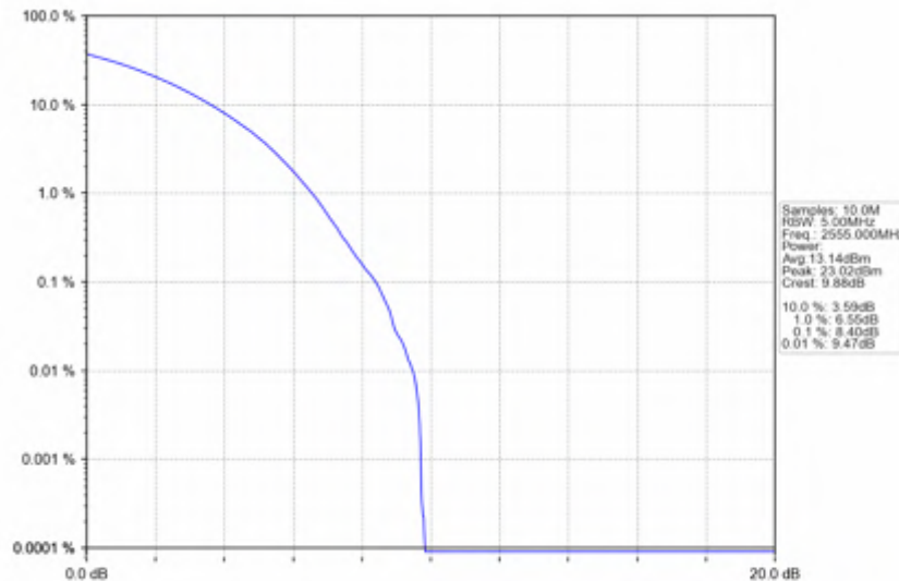
n7_15kHz_SISO_NTNV_30MHz_CP-OFDM_QPSK_2555MHz_Outer_Full
