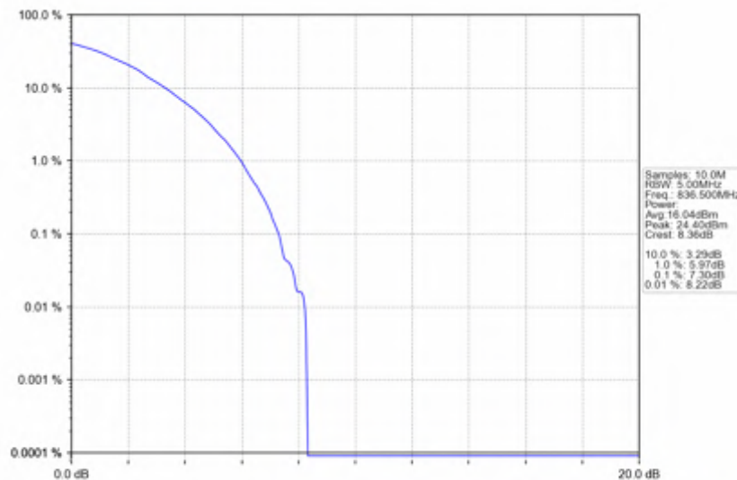
n5_30kHz_SISO_NTNV_20MHz_DFT-s-OFDM 64 QAM_836.5MHz_Outer_Full
