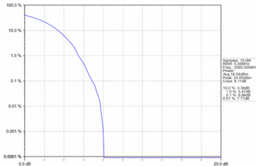
n7_15kHz_SISO_NTNV_10MHz_DFT-s-OFDM_256_QAM_2565MHz_Outer_Full
