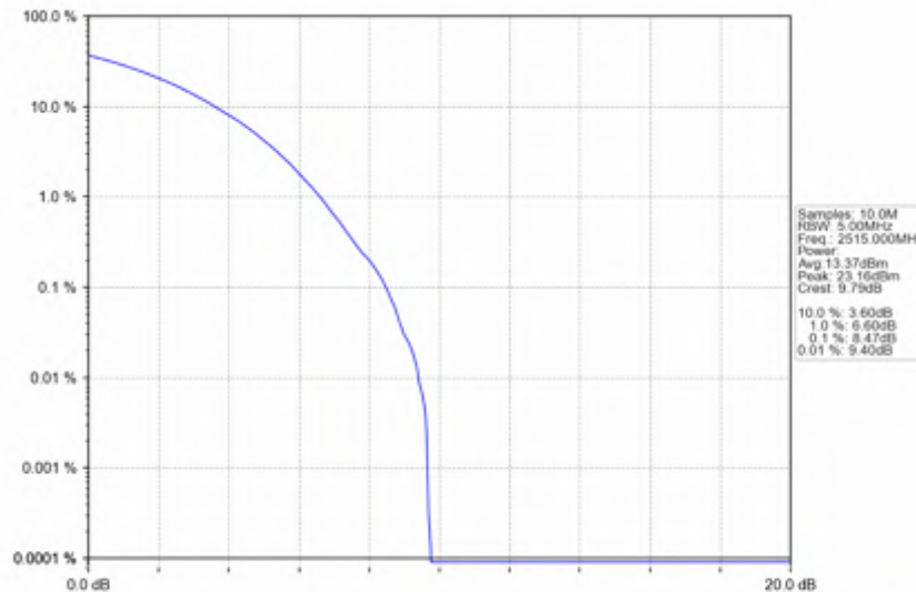
n7_15kHz_SISO_NTNV_30MHz_CP-OFDM_QPSK_2515MHz_Outer_Full
