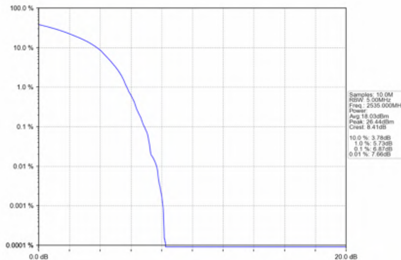
n7_30kHz_SISO_NTNV_15MHz_DFT-s-OFDM_16_QAM_2535MHz_Outer_Full
