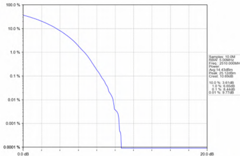
n7_15kHz_SISO_NTNV_20MHz_CP-OFDM 64 QAM_2510MHz_Outer_Full
