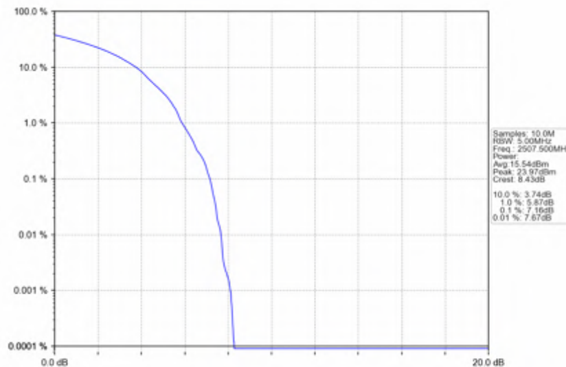
n7_30kHz_SISO_NTNV_15MHz_DFT-s-OFDM_256_QAM_2507.5MHz_Outer_Full
