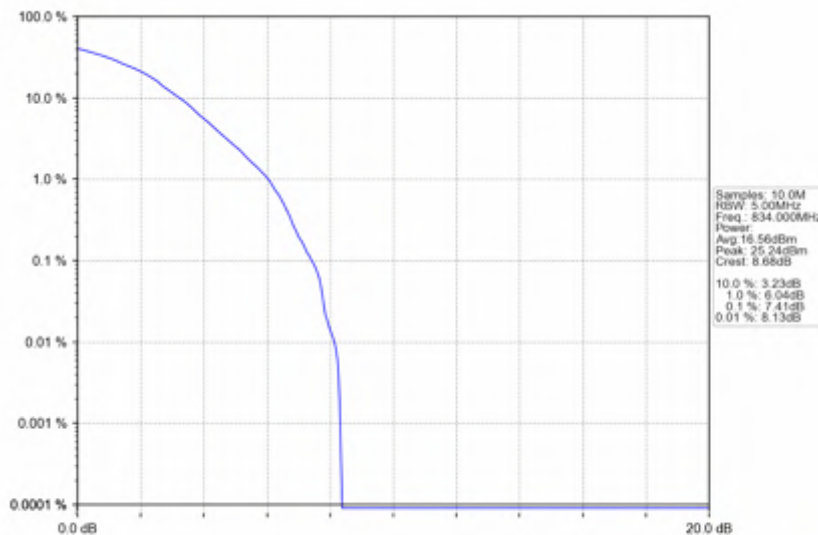
n5_30kHz_SISO_NTNV_20MHz_DFT-s-OFDM_16_QAM_834MHz_Outer_Full
