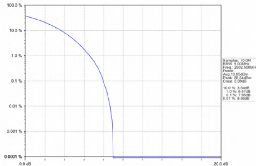
n7_15kHz_SISO_NTNV_5MHz_CP-OFDM_QPSK_2502.5MHz_Outer_Full
