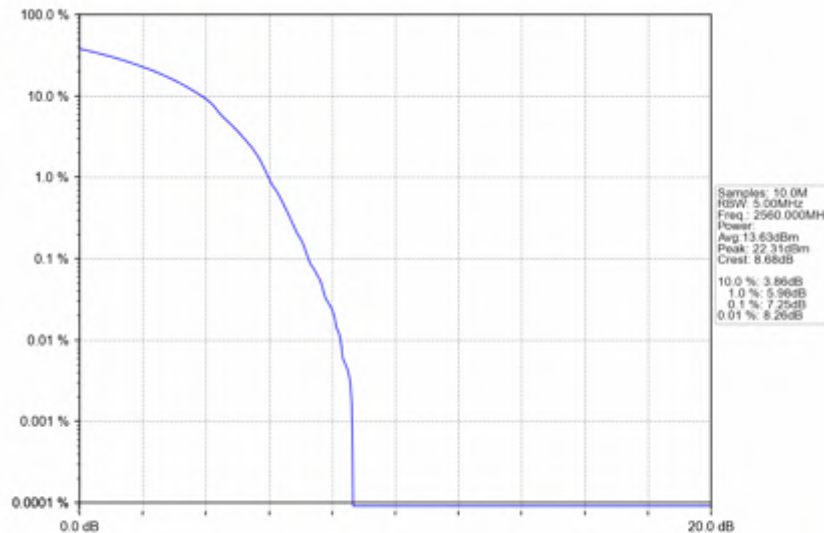
n7_15kHz_SISO_NTNV_20MHz_DFT-s-OFDM_256_QAM_2560MHz_Outer_Full
