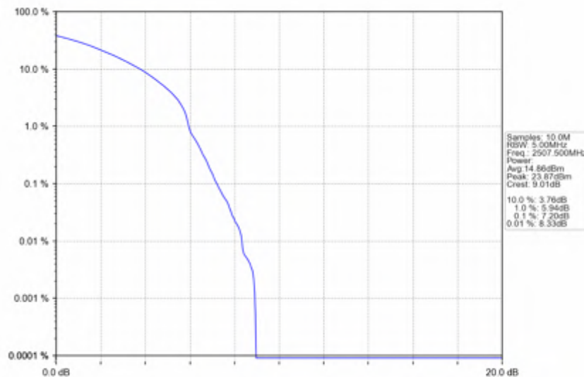
n7_15kHz_SISO_NTNV_15MHz_DFT-s-OFDM_256_QAM_2507.5MHz_Outer_Full
