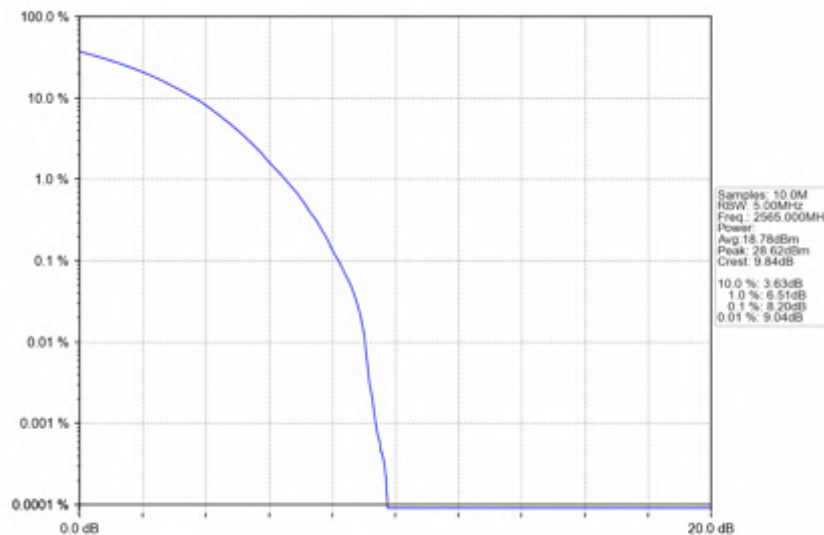
n7_30kHz_SISO_NTNV_10MHz_CP-OFDM_QPSK_2565MHz_Outer_Full
