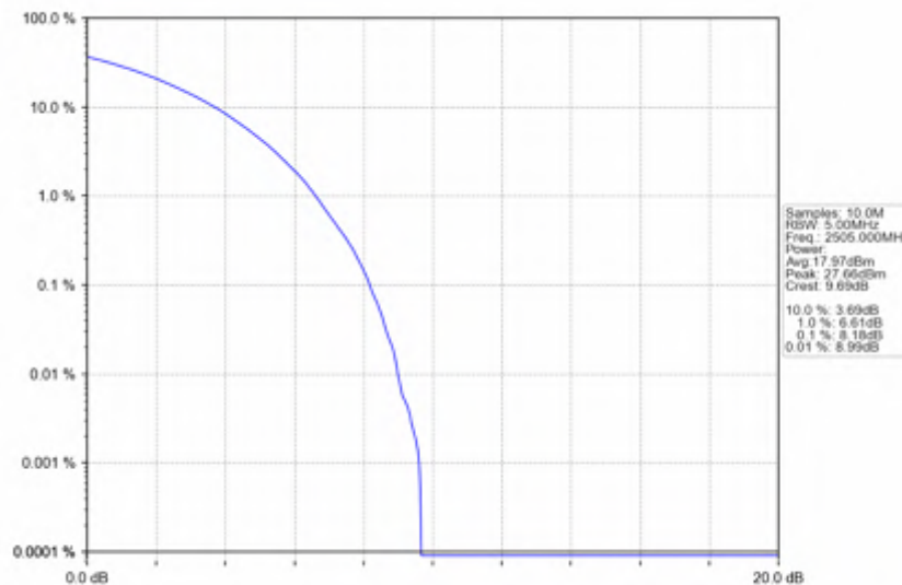
n7_15kHz_SISO_NTNV_10MHz_CP-OFDM_QPSK_2505MHz_Outer_Full
