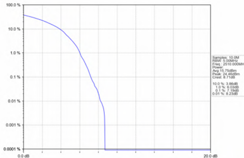
n7_15kHz_SISO_NTNV_20MHz_DFT-s-OFDM_64 QAM_2510MHz_Outer_Full
