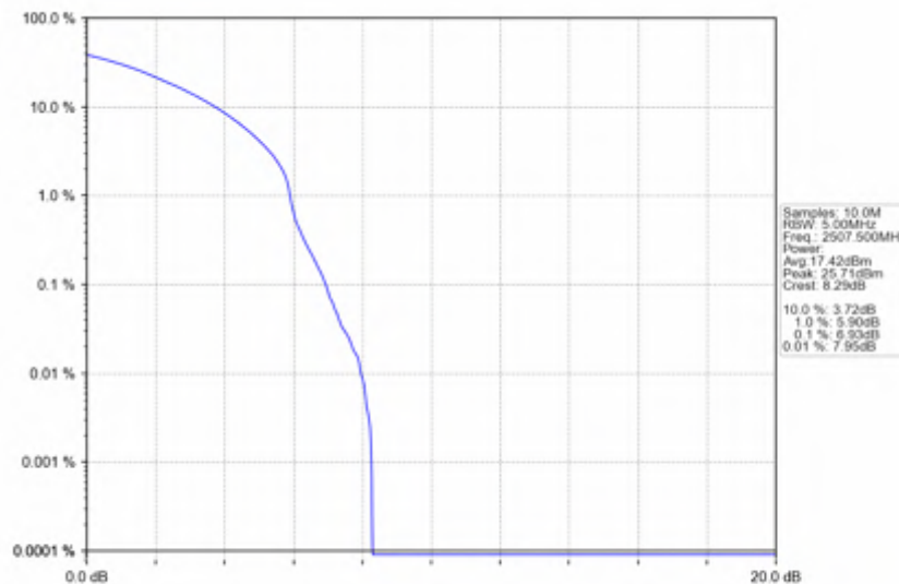
n7_15kHz_SISO_NTNV_15MHz_DFT-s-OFDM_16_QAM_2507.5MHz_Outer_Full
