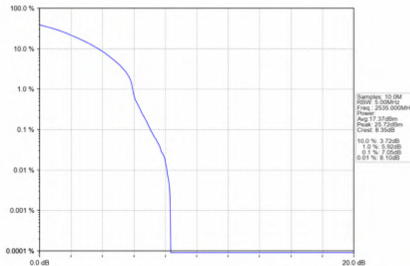
n7_15kHz_SISO_NTNV_15MHz_DFT-s-OFDM_16_QAM_2535MHz_Outer_Full
