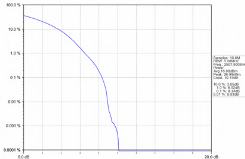
n7_30kHz_SISO_NTNV_15MHz_CP-OFDM_QPSK_2507.5MHz_Outer_Full
