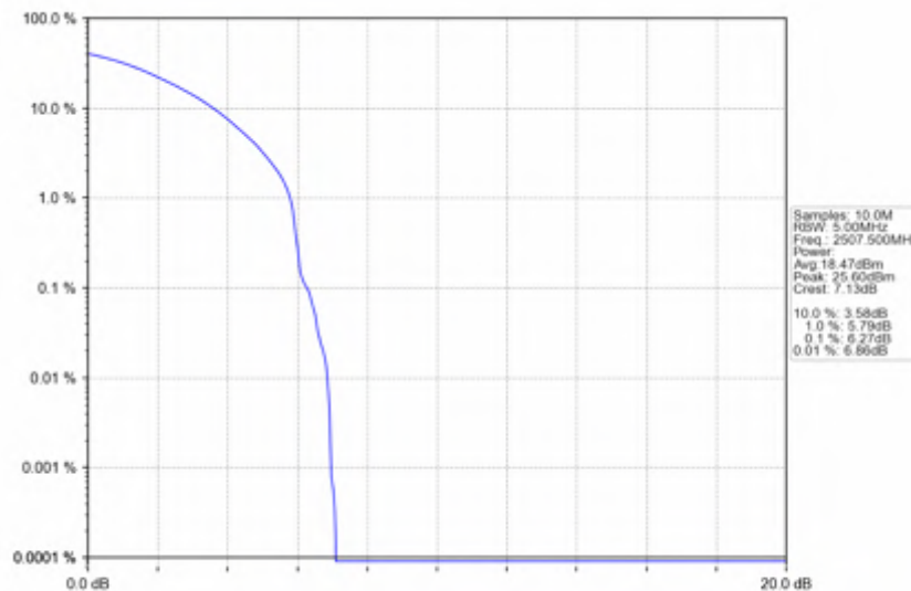
n7_15kHz_SISO_NTNV_15MHz_DFT-s-OFDM QPSK_2507.5MHz_Outer_Full
