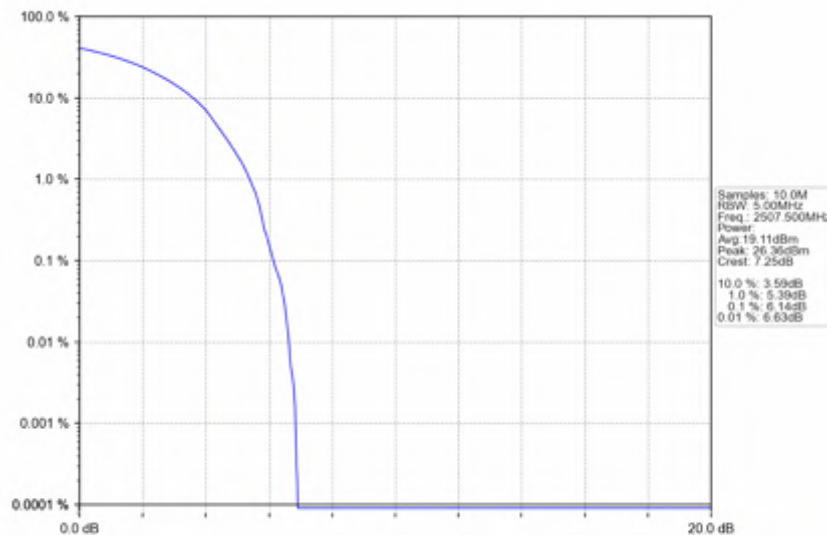
n7_30kHz_SISO_NTNV_15MHz_DFT-s-OFDM QPSK_2507.5MHz_Outer_Full
