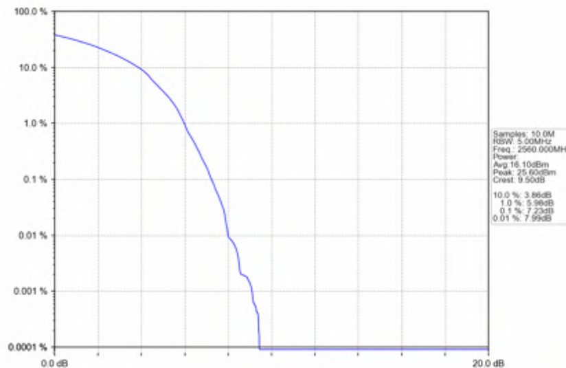
n7_15kHz_SISO_NTNV_20MHz_DFT-s-OFDM_16 QAM_2560MHz_Outer_Full
