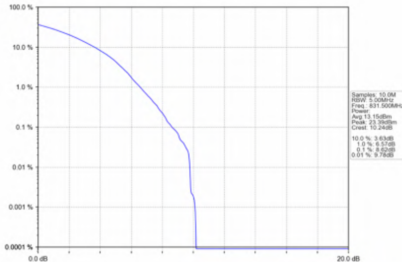
n5_30kHz_SISO_NTNV_15MHz_CP-OFDM_256_QAM_831.5MHz_Outer_Full
