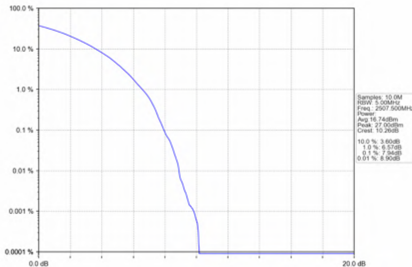
n7_30kHz_SISO_NTNV_15MHz_CP-OFDM_16_QAM_2507.5MHz_Outer_Full
