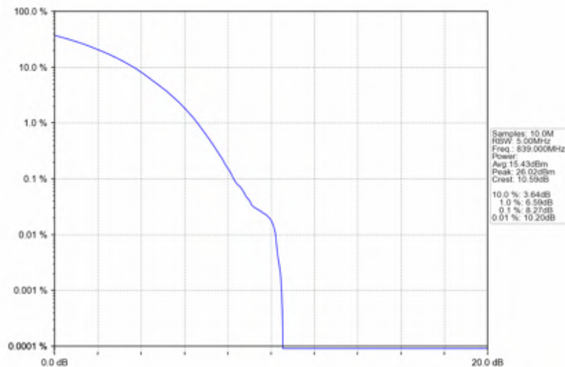
n5_30kHz_SISO_NTNV_20MHz_CP-OFDM_16_QAM_839MHz_Outer_Full
