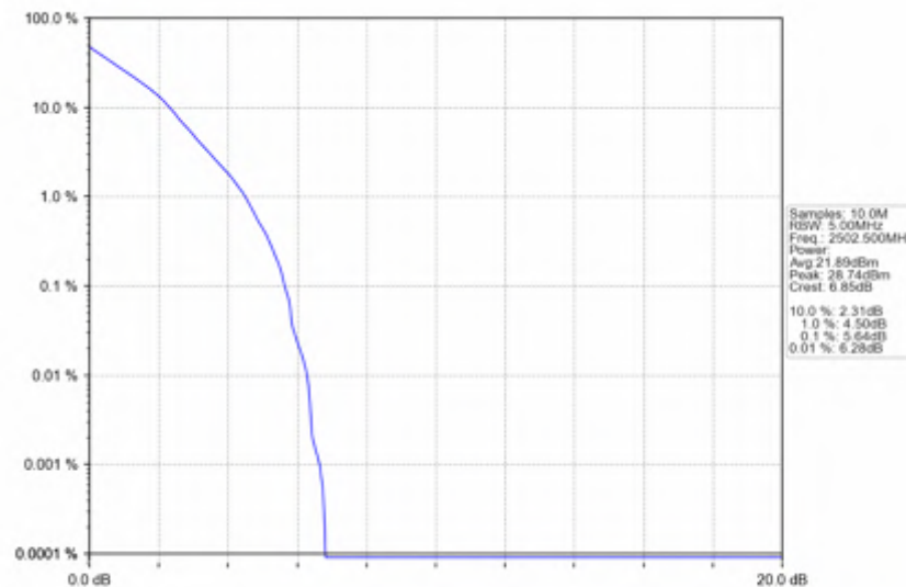
n7_15kHz_SISO_NTNV_5MHz_DFT-s-OFDM QPSK_2502.5MHz_Outer_Full
