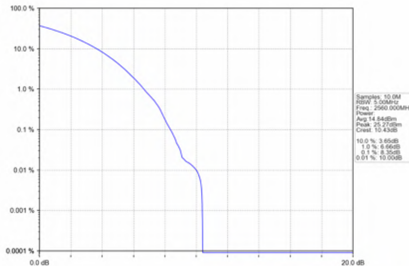
n7_15kHz_SISO_NTNV_20MHz_CP-OFDM 16 QAM_2560MHz_Outer_Full
