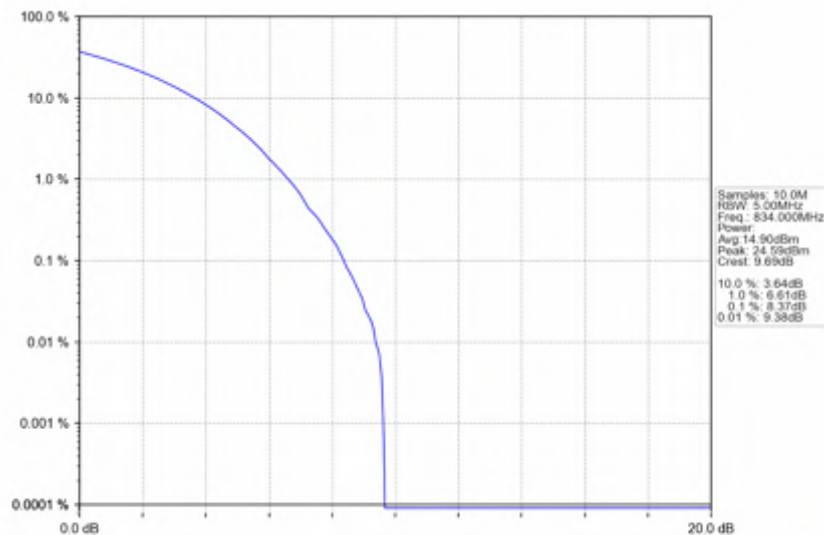
n5_30kHz_SISO_NTNV_20MHz_CP-OFDM_64_QAM_834MHz_Outer_Full
