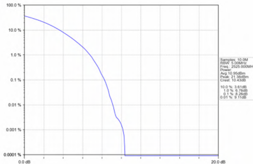
n7_15kHz_SISO_NTNV_50MHz_CP-OFDM_QPSK_2525MHz_Outer_Full
