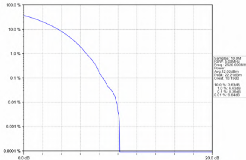
n7_15kHz_SISO_NTNV_40MHz_CP-OFDM_QPSK_2520MHz_Outer_Full
