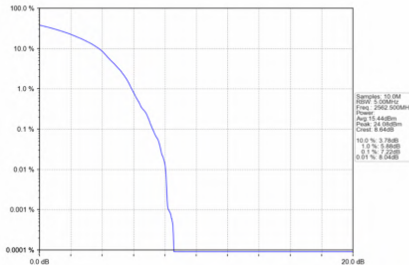
n7_30kHz_SISO_NTNV_15MHz_DFT-s-OFDM_256_QAM_2562.5MHz_Outer_Full
