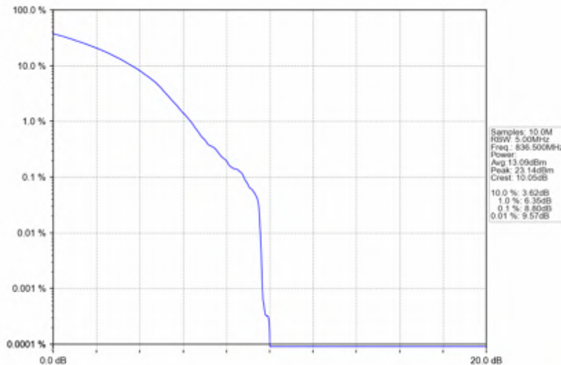
n5_30kHz_SISO_NTNV_15MHz_CP-OFDM_256_QAM_836.5MHz_Outer_Full
