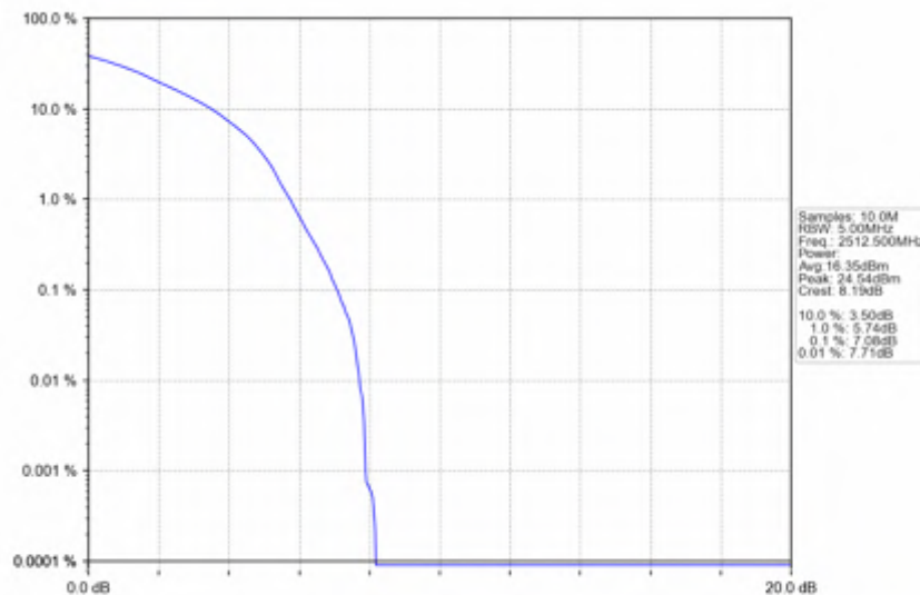
n7_15kHz_SISO_NTNV_25MHz_DFT-s-OFDM QPSK_2512.5MHz_Outer_Full
