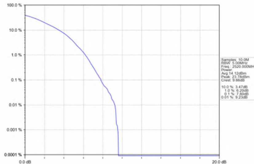
n7_15kHz_SISO_NTNV_40MHz_DFT-s-OFDM QPSK_2520MHz_Outer_Full
