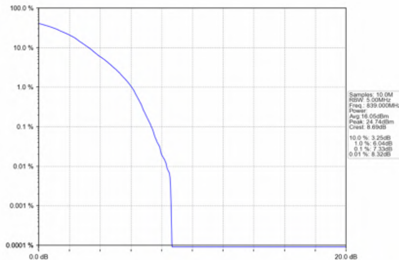
n5_30kHz_SISO_NTNV_20MHz_DFT-s-OFDM 64 QAM_839MHz_Outer_Full
