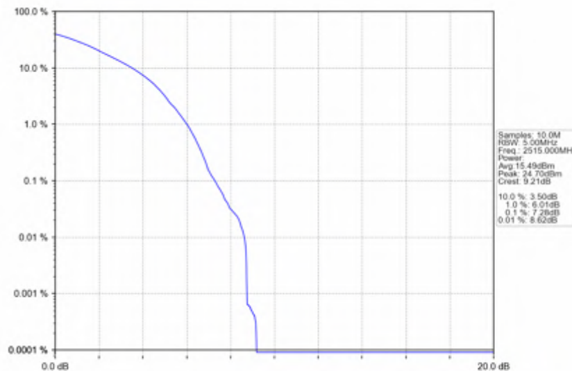
n7_15kHz_SISO_NTNV_30MHz_DFT-s-OFDM QPSK_2515MHz_Outer_Full
