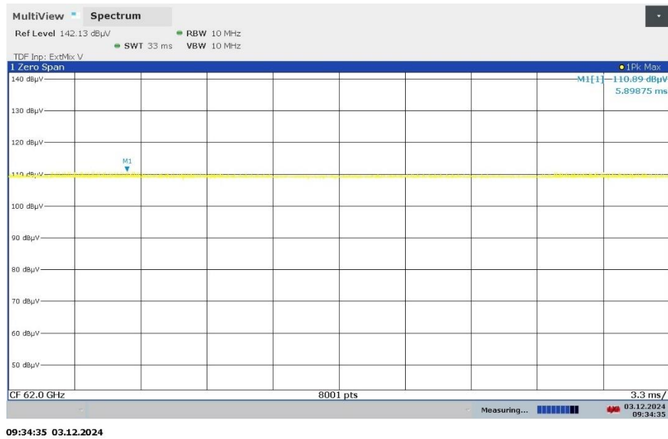
Figure 7.5-3: Field strength of fundamental emissions (middle part of the signal), Zero span
