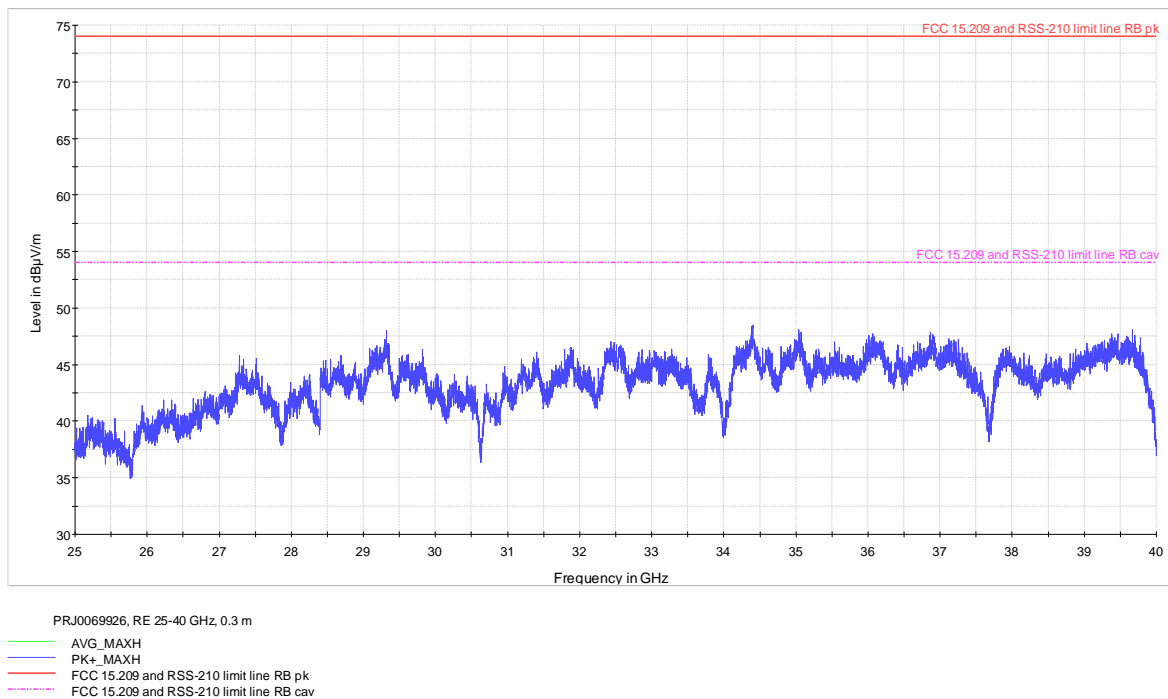
Figure 7.6-4: Radiated spurious emissions 25-40 GHz
