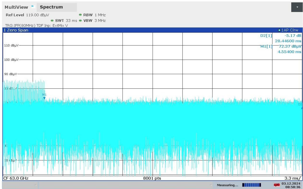
Figure 7.5-5: Off-time duration within 33 ms interval
