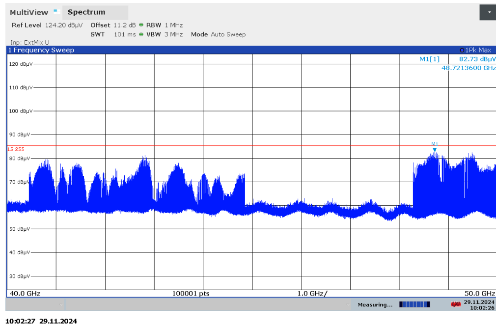
Figure 7.6-5: Radiated spurious emissions 40-50 GHz
