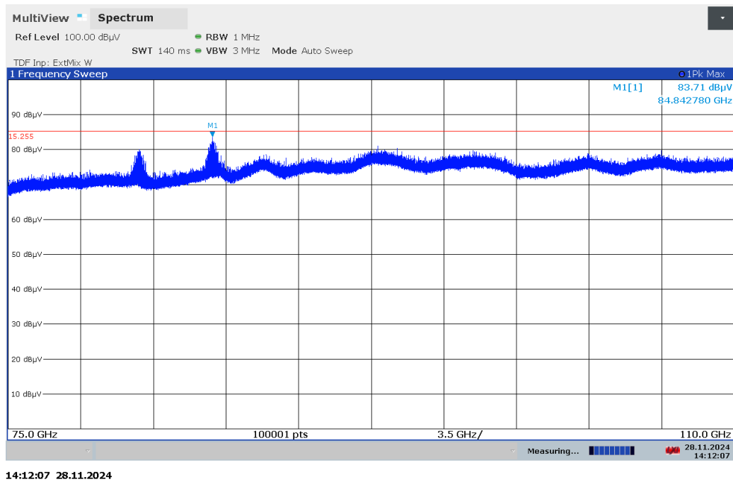
Figure 7.6-7: Radiated spurious emissions 75-110 GHz
