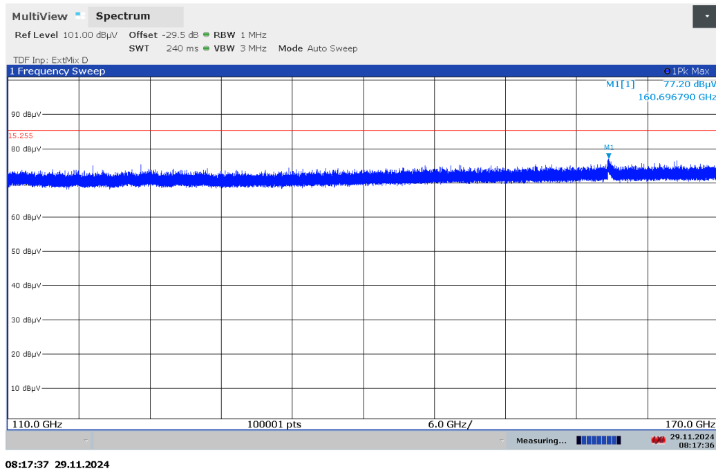
Figure 7.6-8: Radiated spurious emissions 110-170 GHz
