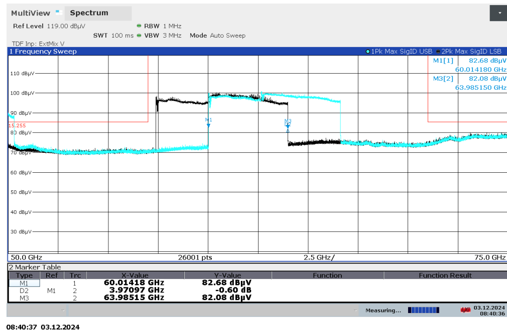
Figure 7.6-6: Radiated spurious emissions 50-75 GHz
