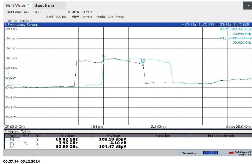
Figure 7.5-1: Fundamental emission view
