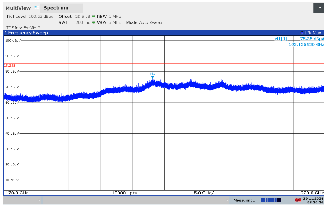
Figure 7.6-9: Radiated spurious emissions 170-220 GHz
