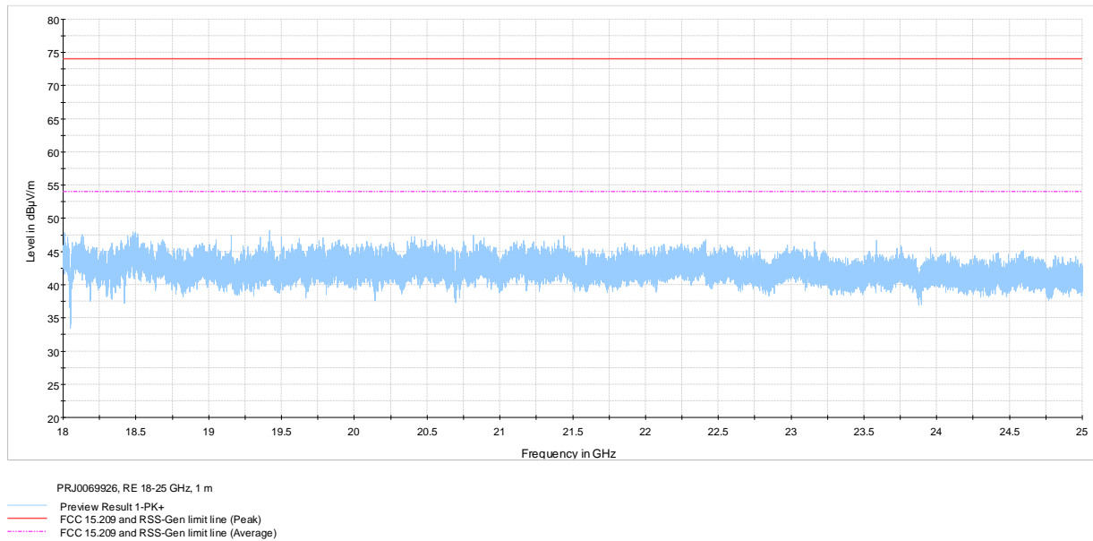
Figure 7.6-3: Radiated spurious emissions 18-25 GHz
