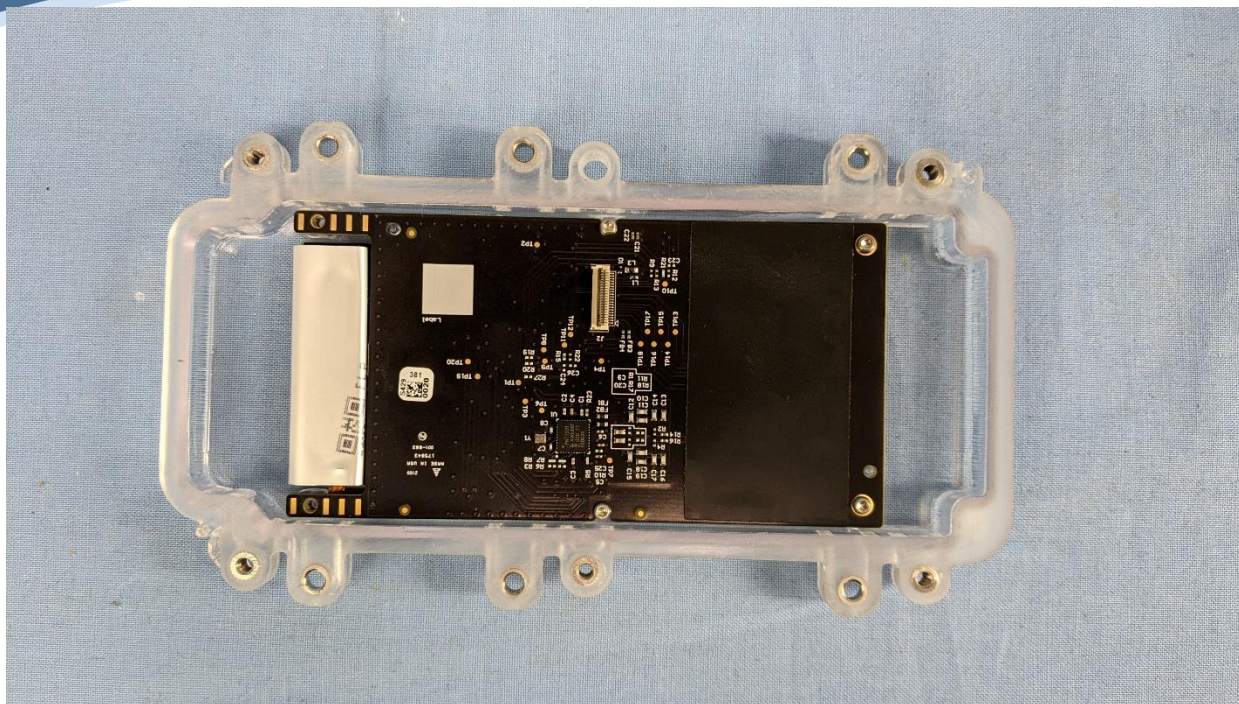
Screen/NFC Board Back
