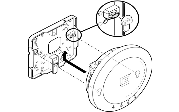
Figure 4 Mounting the AP using the optional wall and box bracket
