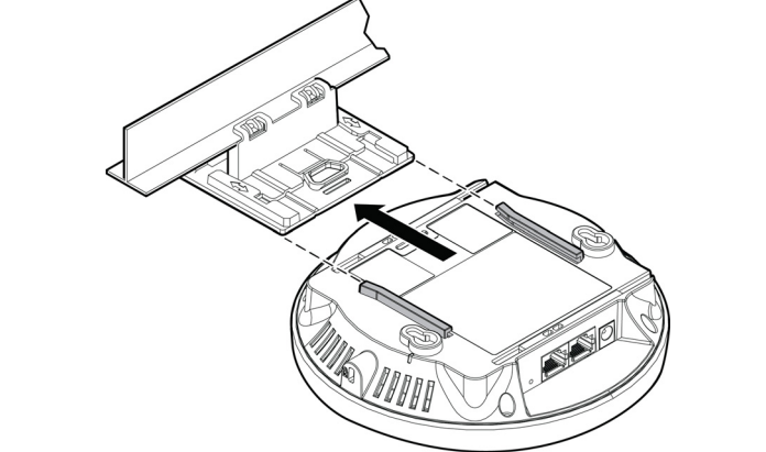
Figure 5 AP3915i Mounted on Drop Ceiling T-bar Rail
