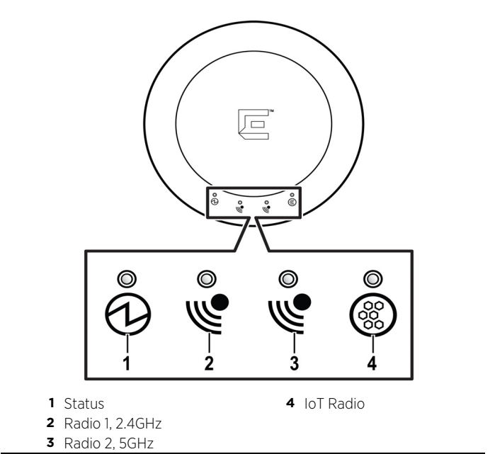
Figure 2 LEDs on AP Front Face
