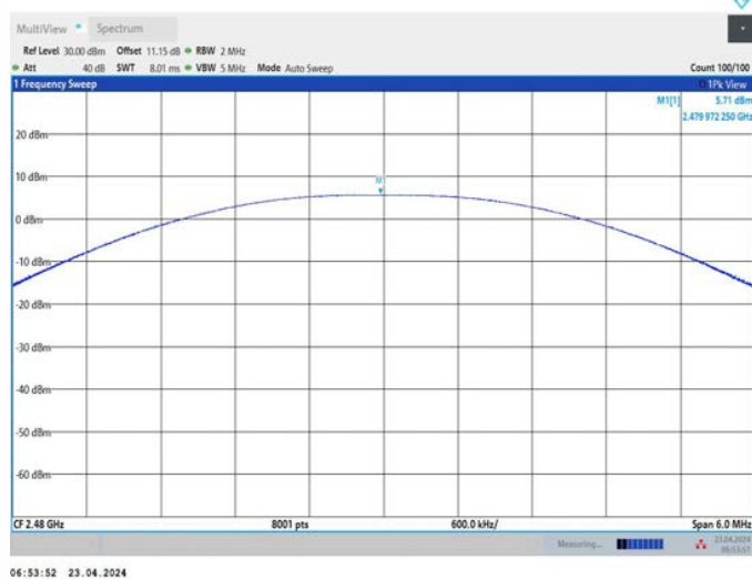
BLE_1M_Ant1_2480
