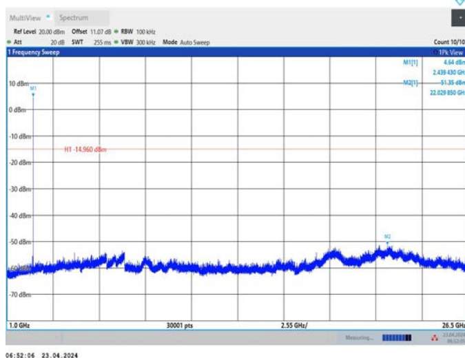
BLE_1M_Ant1_2440_1000~26500
