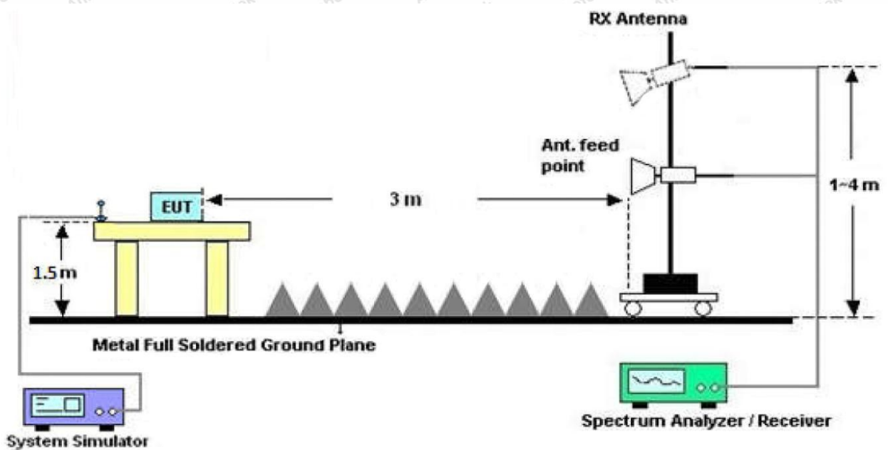
Figure 3. Above 1 GHz
