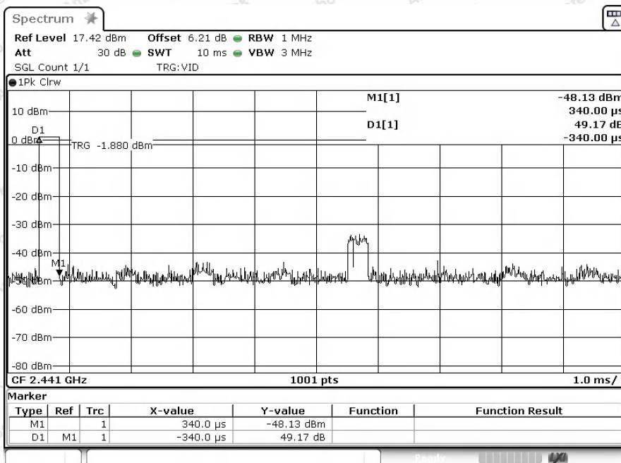
Dwell_Time_(Hopping)_NVNT_ANT1_1-DH5_2441_One_Burst_Time
