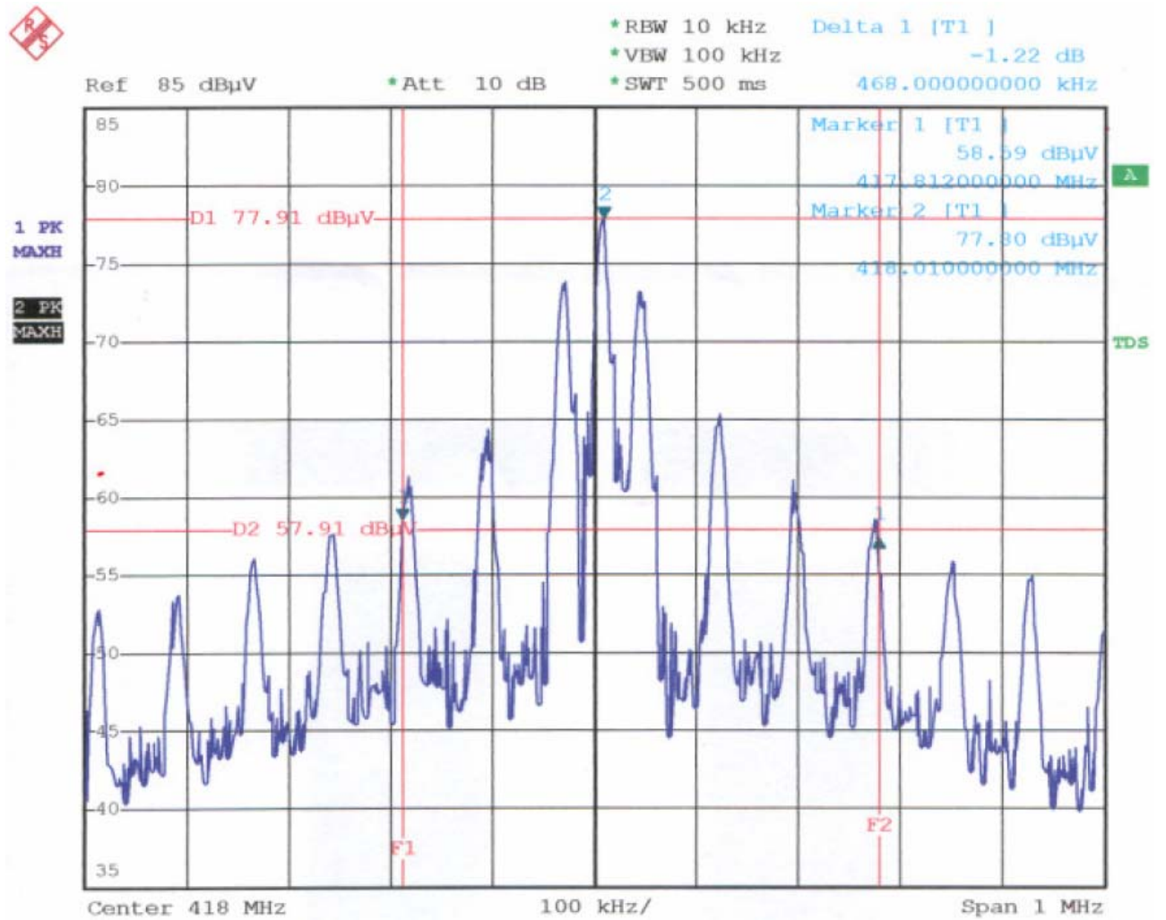
<Plot of occupied bandwidth >
