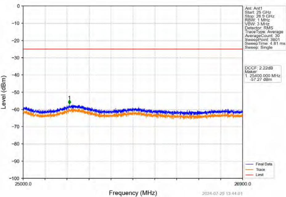
Band41_20MHz_16QAM_LCH_2506MHz_RB_100_0_NTNV
