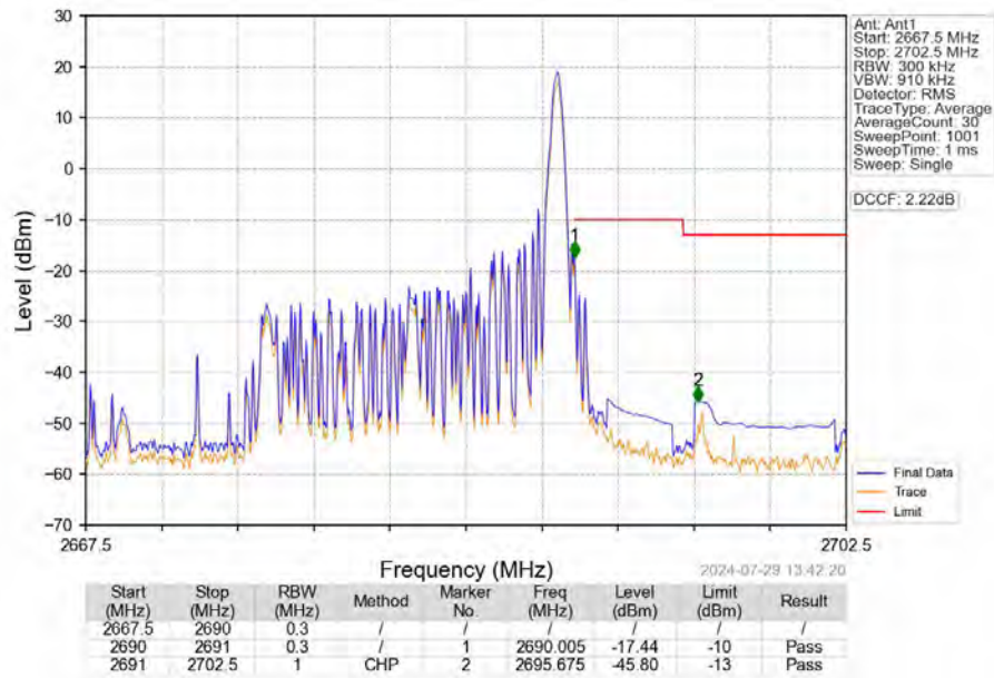
Band41_15MHz_16QAM_HCH_2682.5MHz_RB_1_74_NTNV
