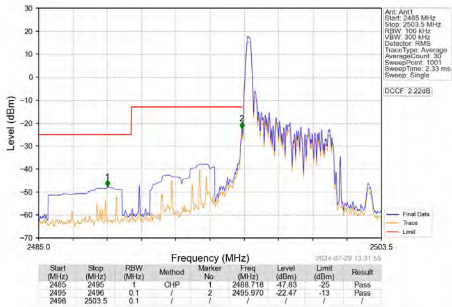
Band41_5MHz_16QAM_LCH_2498.5MHz_RB_1_0_NTNV
