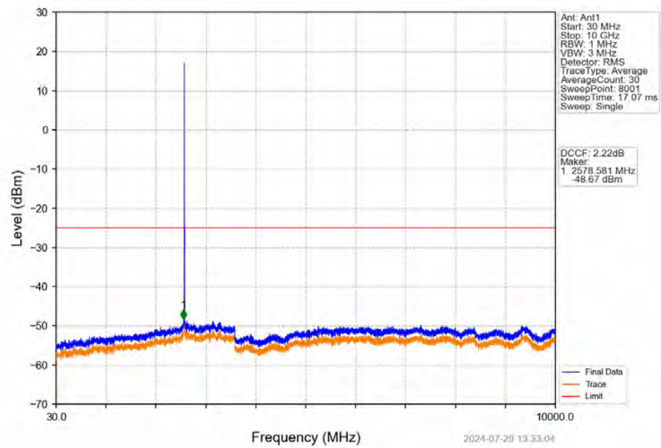
Band41_5MHz_16QAM_MCH_2593MHz_RB_1_0_NTNV
