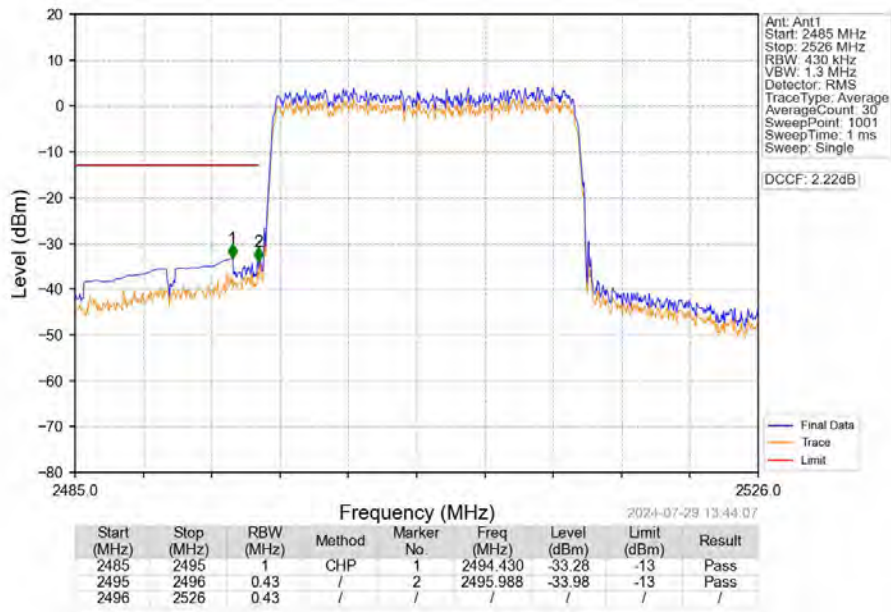
Band41_20MHz_16QAM_LCH_2506MHz_RB_100_0_NTNV
