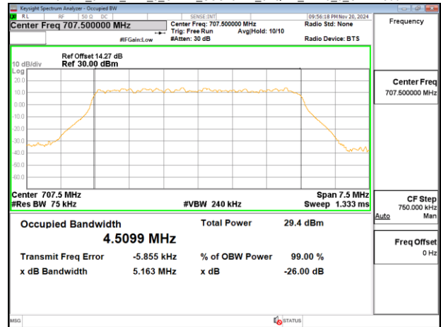
Band12_5MHz_DFT_s_OFDM_SCS15kHz_64QAM_RB25_0_CH142700
