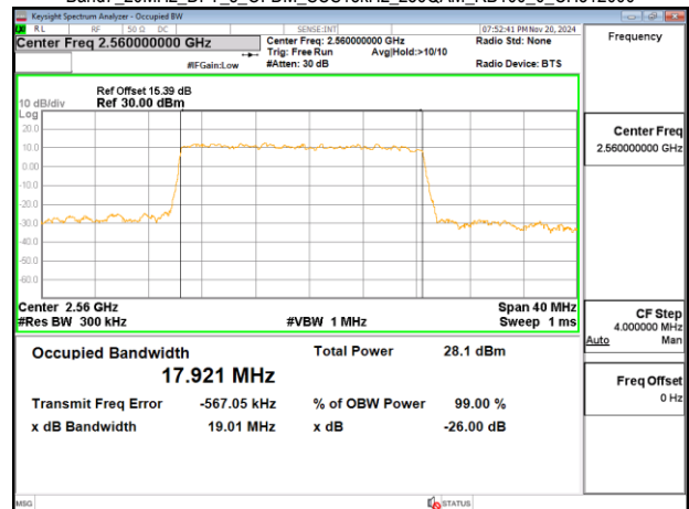
Band7_20MHz_DFT_s_OFDM_SCS15kHz_256QAM_RB100_0_CH512000
