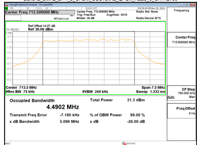
Band12_5MHz_DFT_s_OFDM_SCS15kHz_QPSK_RB25_0_CH142700
