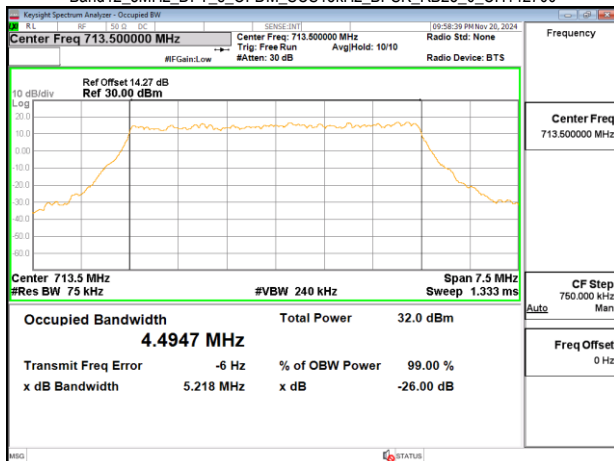
Band12_5MHz_DFT_s_OFDM_SCS15kHz_BPSK_RB25_0_CH142700
