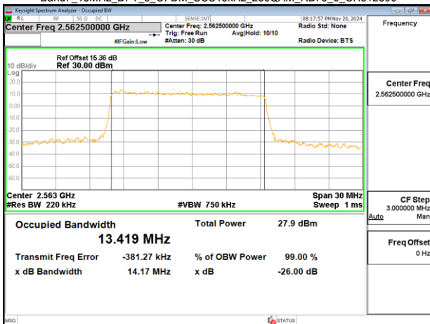
Band7_15MHz_DFT_s_OFDM_SCS15kHz_256QAM_RB75_0_CH512500
