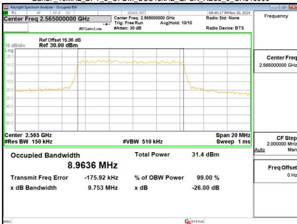
Band7_10MHz_DFT_s_OFDM_SCS15kHz_QPSK_RB50_0_CH513000
