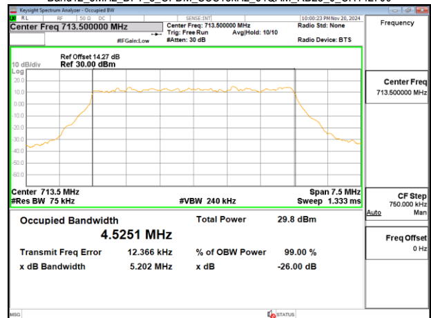
Band12_5MHz_DFT_s_OFDM_SCS15kHz_64QAM_RB25_0_CH142700
