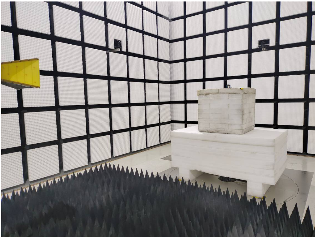
Radiated Emission Above 1GHz View-Ceramic ANT1
