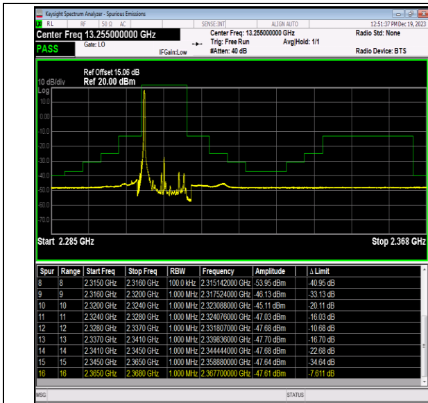
Band40_10MHz_64QAM_38750_1RB#0
