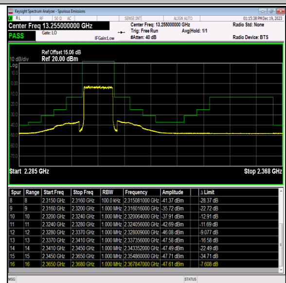
Band40_10MHz_16QAM_38750_50RB#0
