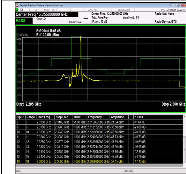
Band40_5MHz_16QAM_38775_1RB#24
