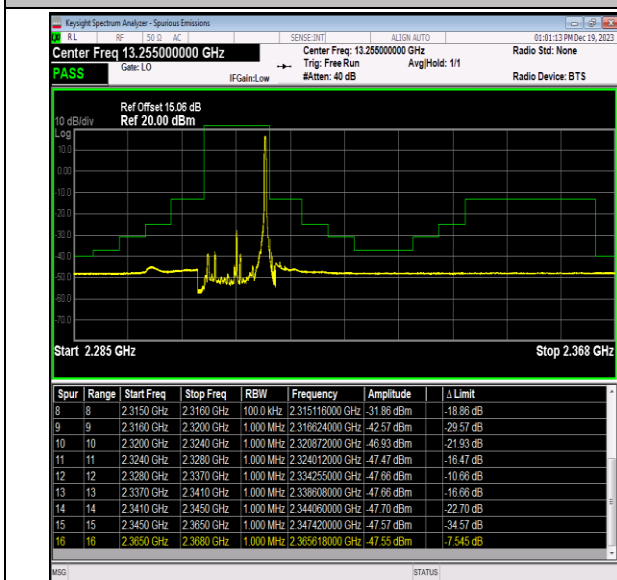
Band40_10MHz_16QAM_38750_1RB#49
