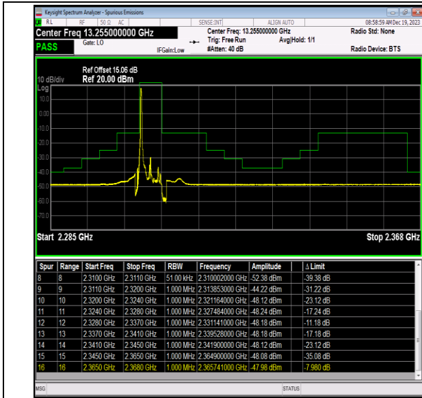
Band40_5MHz_64QAM_38725_1RB#0
