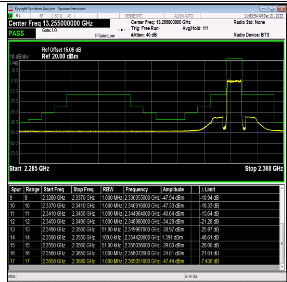
Band40_5MHz_QPSK_39175_25RB#0
