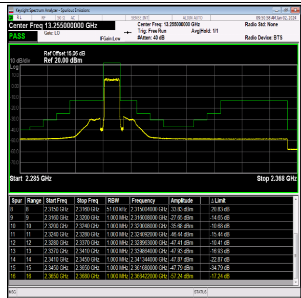
Band40_5MHz_64QAM_38775_25RB#0
