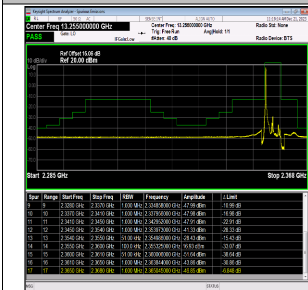
Band40_5MHz_QPSK_39225_1RB#0
