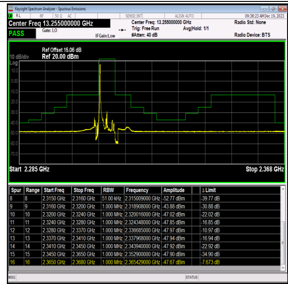
Band40_5MHz_16QAM_38775_1RB#0
