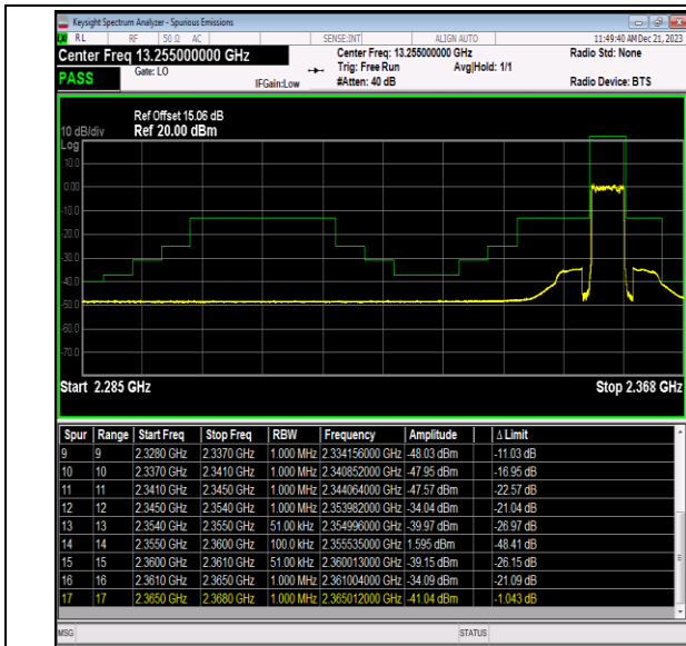
Band40_5MHz_QPSK_39225_25RB#0
