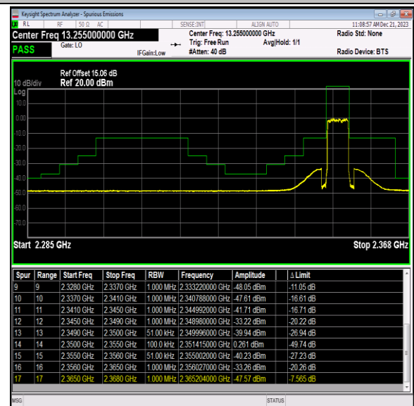
Band40_5MHz_16QAM_39175_25RB#0
