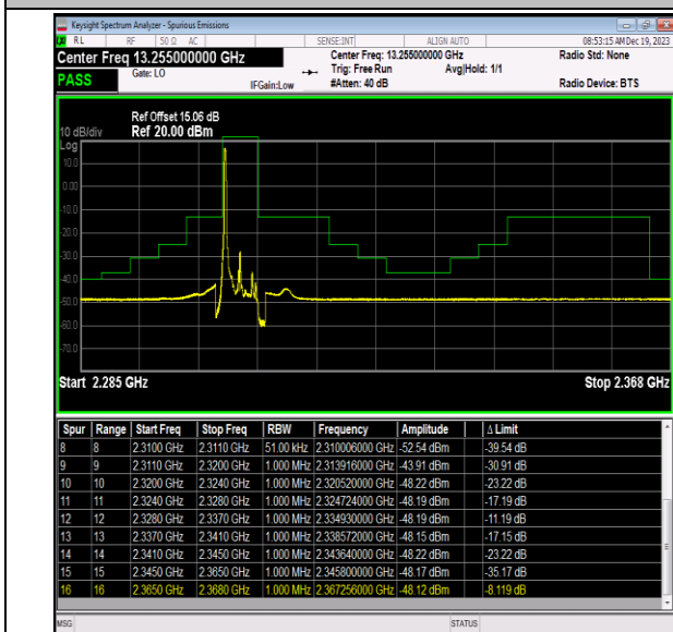
Band40_5MHz_16QAM_38725_1RB#0
