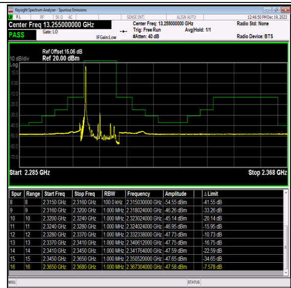
Band40_10MHz_16QAM_38750_1RB#0
