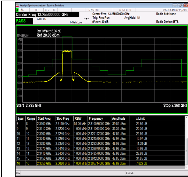
Band40_5MHz_16QAM_38725_25RB#0
