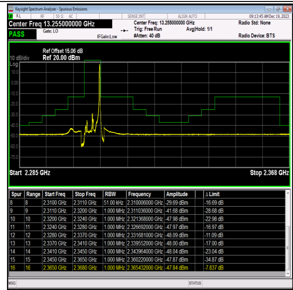
Band40_5MHz_64QAM_38725_1RB#24
