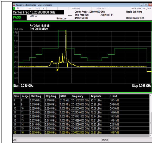
Band40_5MHz_QPSK_38775_1RB#24
