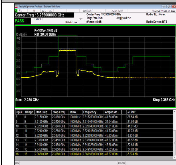
Band40_10MHz_64QAM_38750_50RB#0
