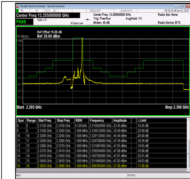
Band40_5MHz_64QAM_38775_1RB#24
