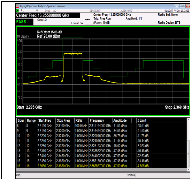
Band40_10MHz_QPSK_38750_50RB#0
