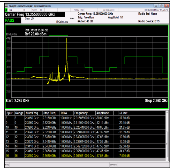
Band40_10MHz_64QAM_38750_1RB#49
