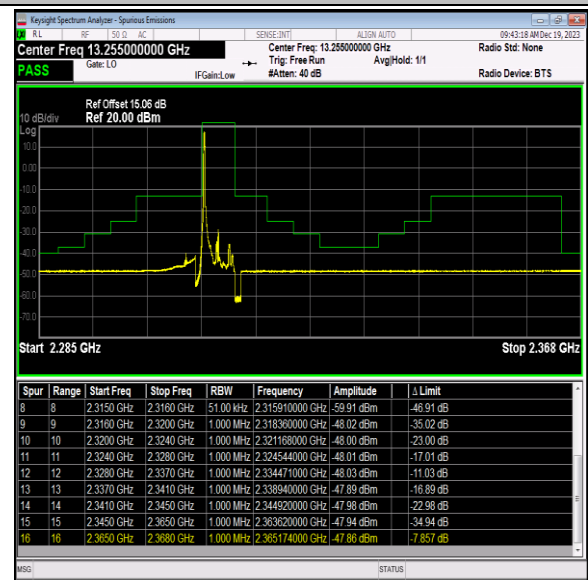
Band40_5MHz_64QAM_38775_1RB#0
