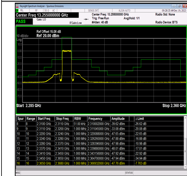
Band40_5MHz_64QAM_38725_25RB#0
