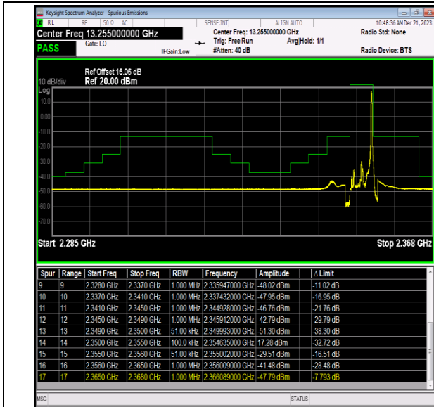
Band40_5MHz_QPSK_39175_1RB#24
