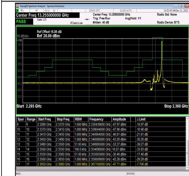
Band40_5MHz_16QAM_39175_1RB#24
