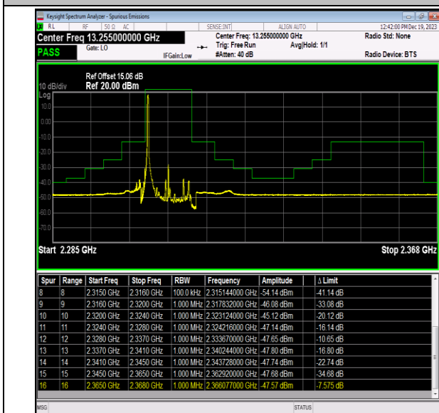
Band40_10MHz_QPSK_38750_1RB#0
