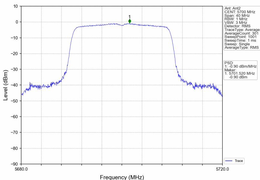
802.11ax(HEW20)_HCH_5700MHz_RU242_Left_Ant2_NTNV
