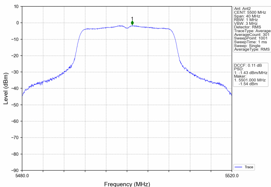
802.11ac(VHT20)_LCH_5500MHz_Ant2_NTNV
