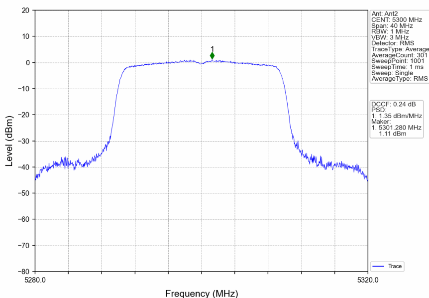
802.11ax(HEW20)_MCH_5300MHz_RU242_Left_Ant2_NTNV
