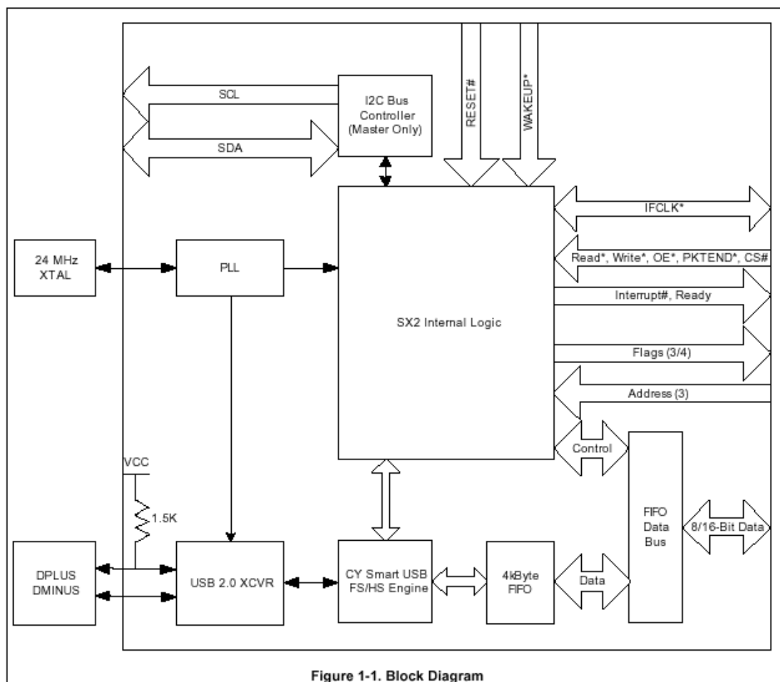
Figure 1-1. Block Diagram
