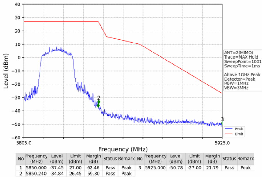
802.11ax(HEW20)_HCH_5825MHz_RU242_Left_Ant2_NTNV
