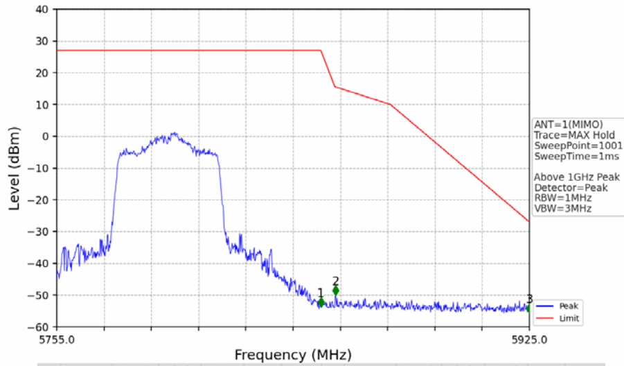
802.11ac(VHT40)_HCH_5795MHz_Ant1_NTNV
