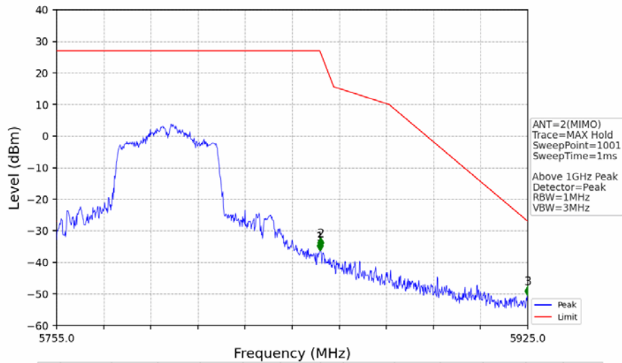
802.11ac(VHT40)_HCH_5795MHz_Ant2_NTNV
