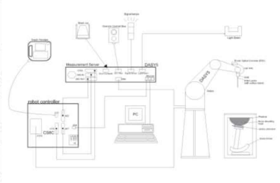
Figures 7.1-1 SAR Measurement Set-up
