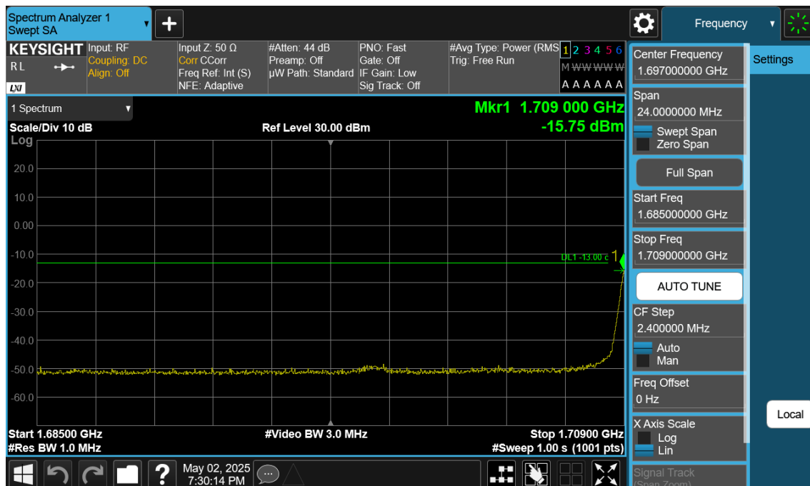
25 MHz / \pi/2 BPSK / RB Size/Offset (1/Edge Left)
