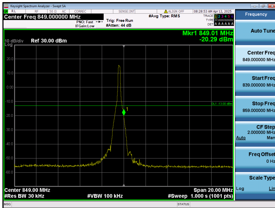
10 MHz / QPSK / RB Size/Offset (1/Edge Right)
