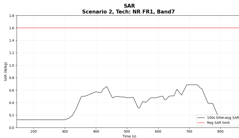
Figure 6-11 Time-averaged SAR for case 2.4(sub6 NR n7)
