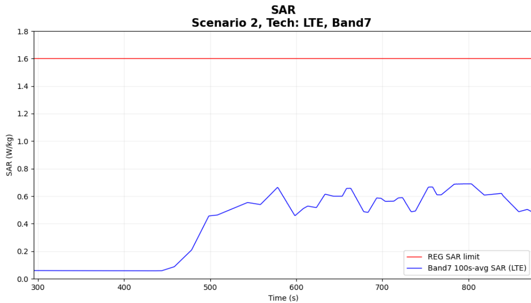
Figure 7-9 Time-averaged SAR for case 8 in table 7-1 (4G LTE B7)
