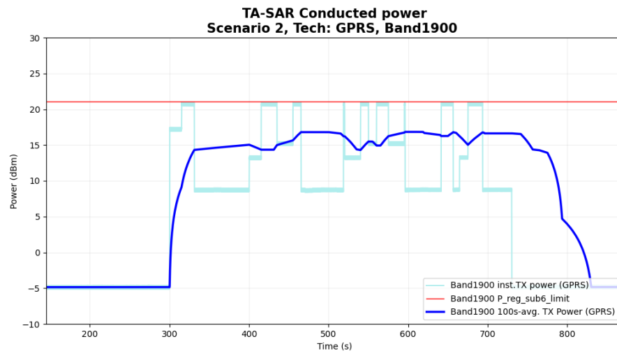
Figure 6-34 Time-averaged conducted TX power over time for case 2.16(2G PCS1900)
