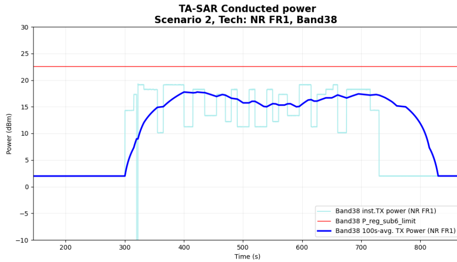
Figure 6-10 Time-averaged conducted TX power over time for case 2.2(sub6 NR n38)
