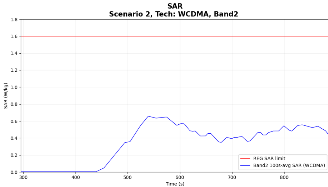
Figure 7-11 Time-averaged SAR for case 10 in table 7-1 (3G WCDMA B2)
