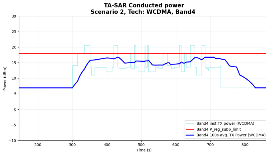
Figure 6-26 Time-averaged conducted TX power over time for case 2.12(WCDMA B4)
