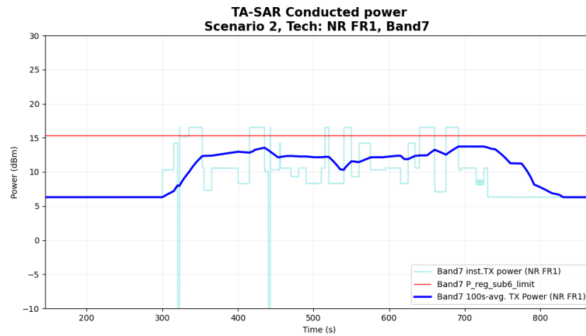
Figure 6-10 Time-averaged conducted TX power over time for case 2.4(sub6 NR n7)
