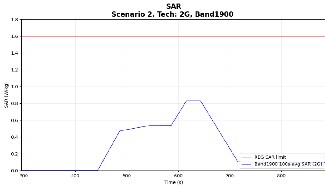
Figure 7-14 Time-averaged SAR for case 13 in table 7-1 (2G GSM 1900)
