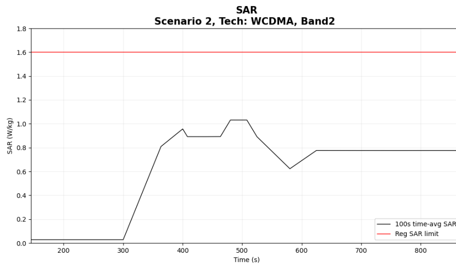
Figure 6-21 Time-averaged SAR for case 2.9(WCDMA B2)
