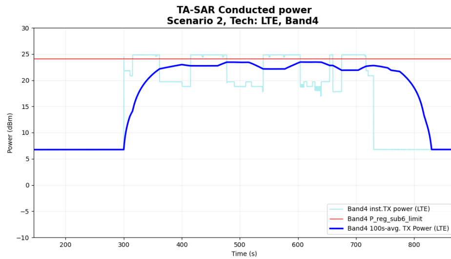
Figure 6-14 Time-averaged conducted TX power over time for case 2.6(LTE B4)
