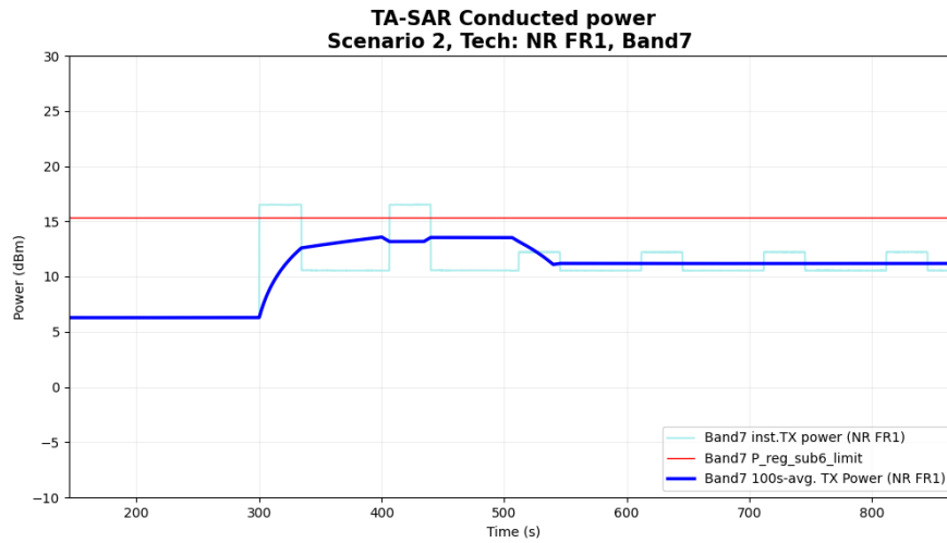
Figure 6-8 Time-averaged conducted TX power over time for case 2.3(sub6 NR n7)
