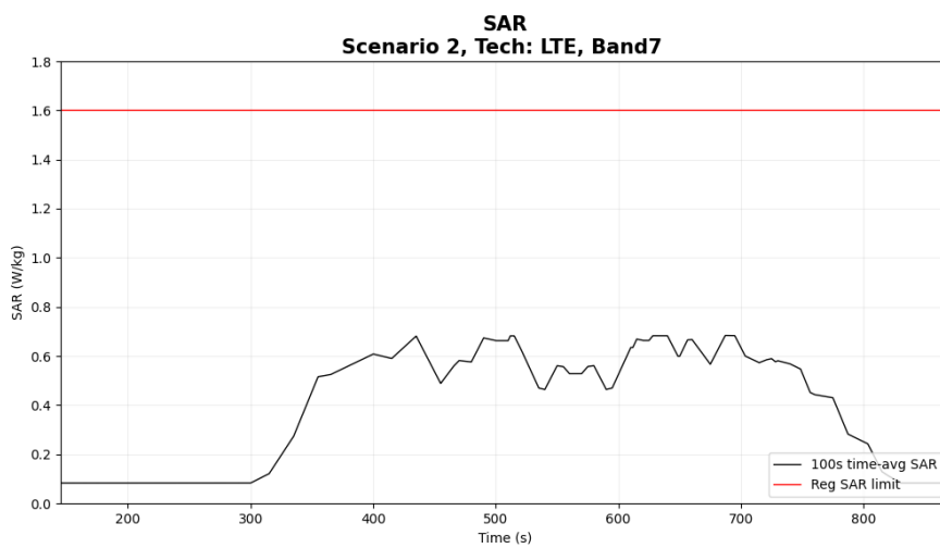
Figure 6-19 Time-averaged SAR for case 2.8(LTE B7)
