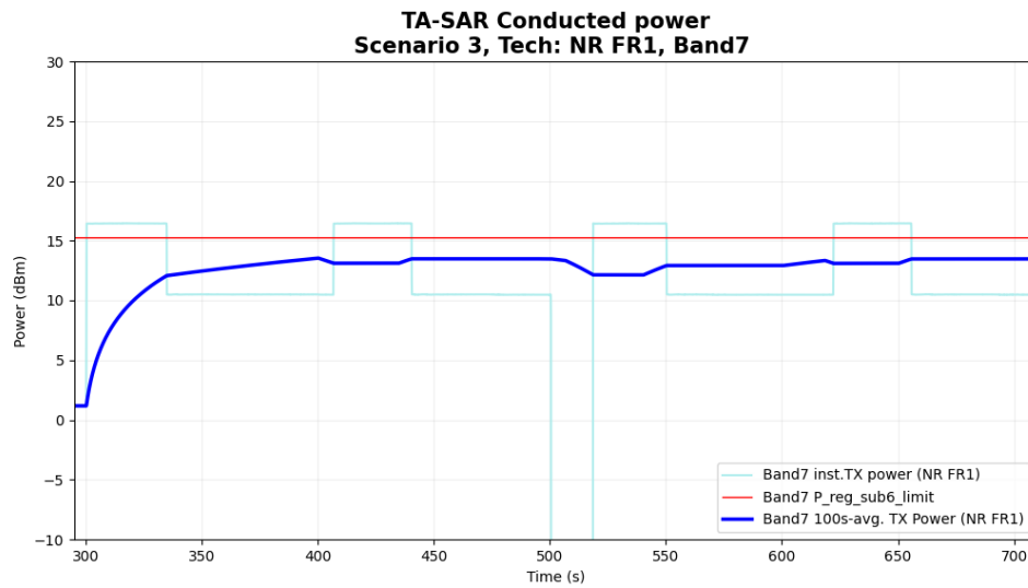
Figure 6-36 Time-averaged conducted TX power over time for case 3.1(sub6 NR n7)
