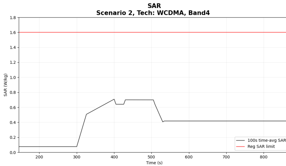
Figure 6-25 Time-averaged SAR for use 2.11(WCDMA B4)
