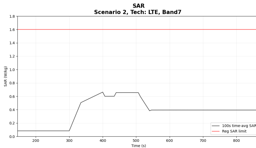
Figure 6-17 Time-averaged SAR for case 2.7(LTE B7)
