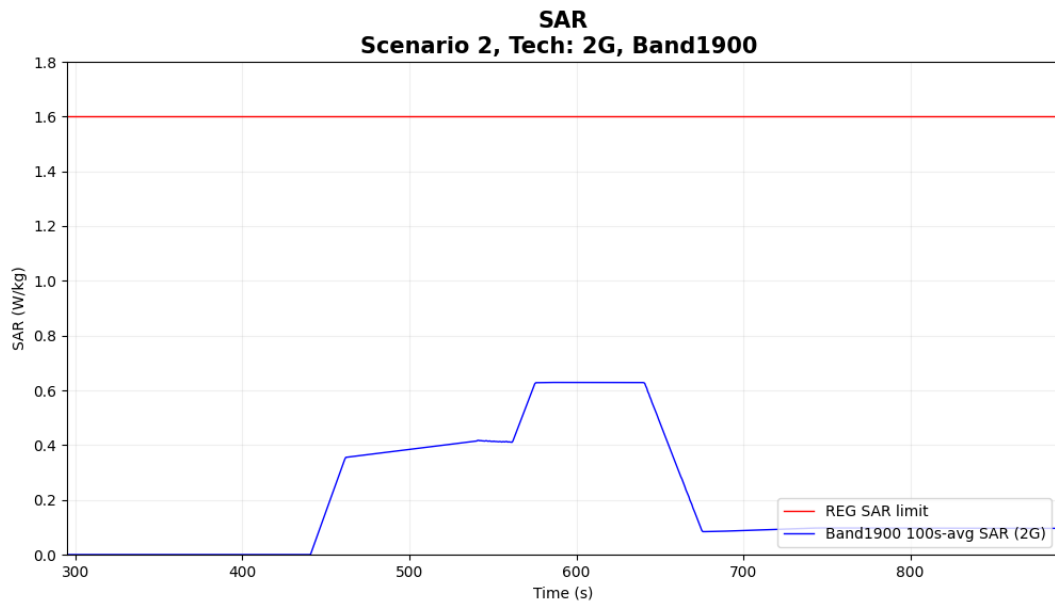
Figure 7-16 Time-averaged SAR for case 15 in table 7-1 (2G GSM 1900)
