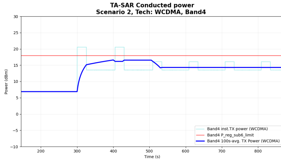
Figure 6-24 Time-averaged conducted TX power over time for case 2.11(WCDMA B4)
