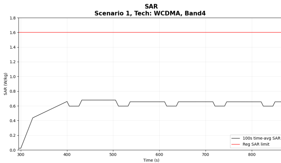
Figure 6-7 Time-averaged SAR for case 0
