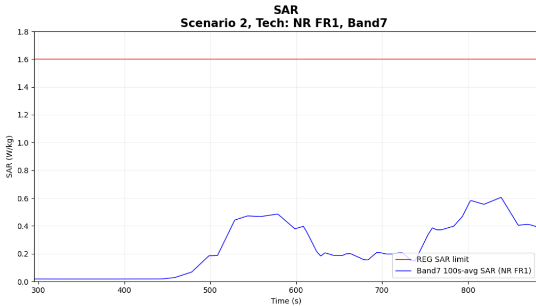
Figure 7-5 Time-averaged SAR for case 4 in table 7-1 (sub NR n7)
