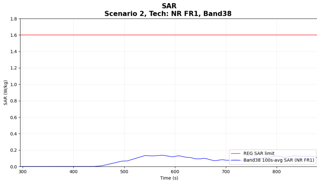
Figure 7-3 Time-averaged SAR for case 2 in table 7-1 (sub NR n38)
