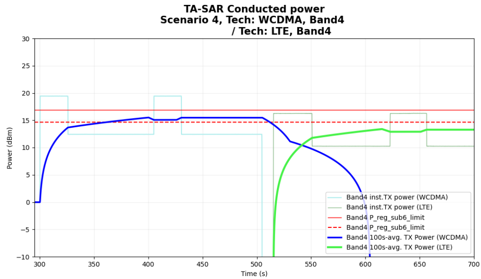
Figure 6-38 Time-averaged conducted TX power over time for case 4.1(WCDMA B4, LTE B4)
