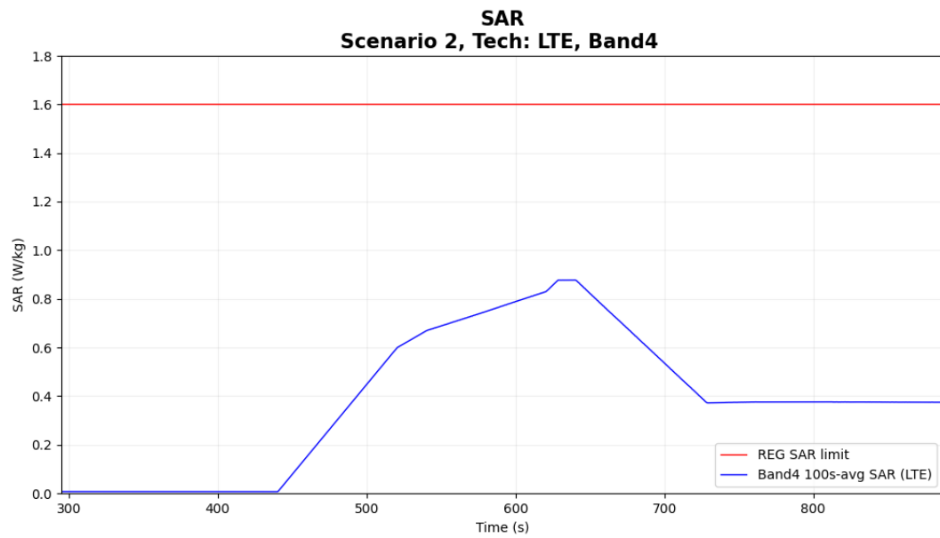
Figure 7-6 Time-averaged SAR for case 5 in table 7-1 (4G LTE B4)
