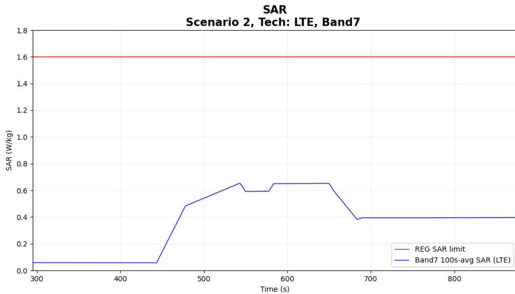
Figure 7-8 Time-averaged SAR for case 7 in table 7-1 (4G LTE B7)
