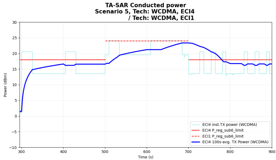
Figure 6-40 Time-averaged conducted TX power over time for case 5.1(WCDMA B4)
