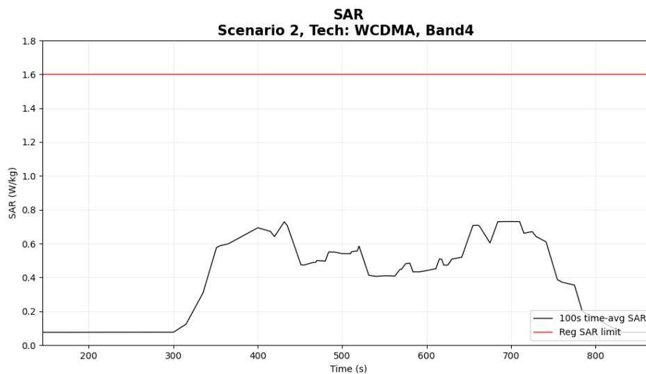
Figure 6-27 Time-averaged SAR for case case 2.12(WCDMA B4)
