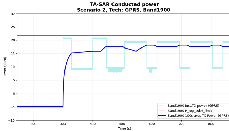
Figure 6-28 Time-averaged conducted TX power over time for case 2.13(2G PCS1900)
