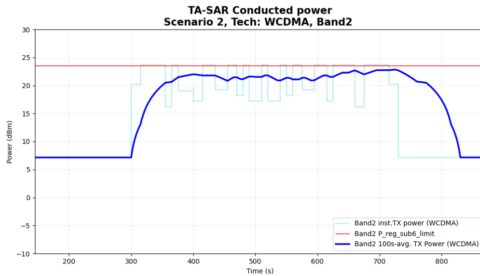
Figure 6-22 Time-averaged conducted TX power over time for case 2.10(WCDMA B2)
