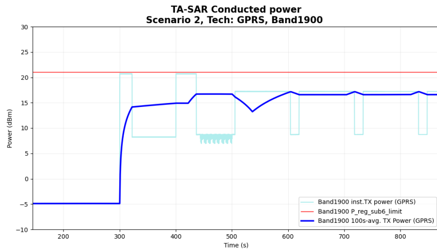
Figure 6-32 Time-averaged conducted TX power over time for case 2.15(2G PCS1900)
