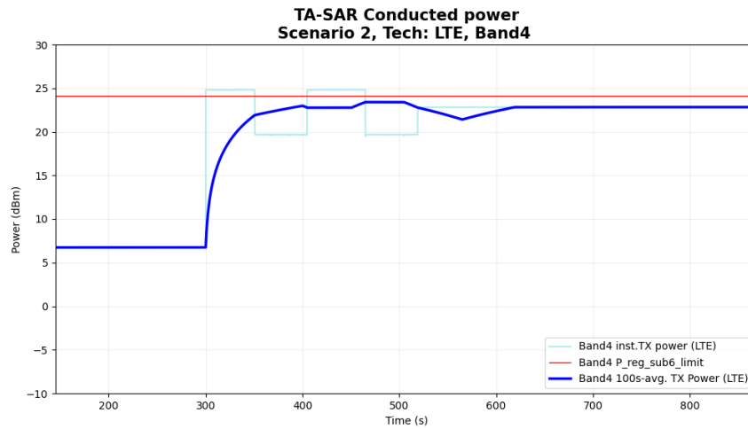
Figure 6-12 Time-averaged conducted TX power over time for case 2.5(LTE B4)
