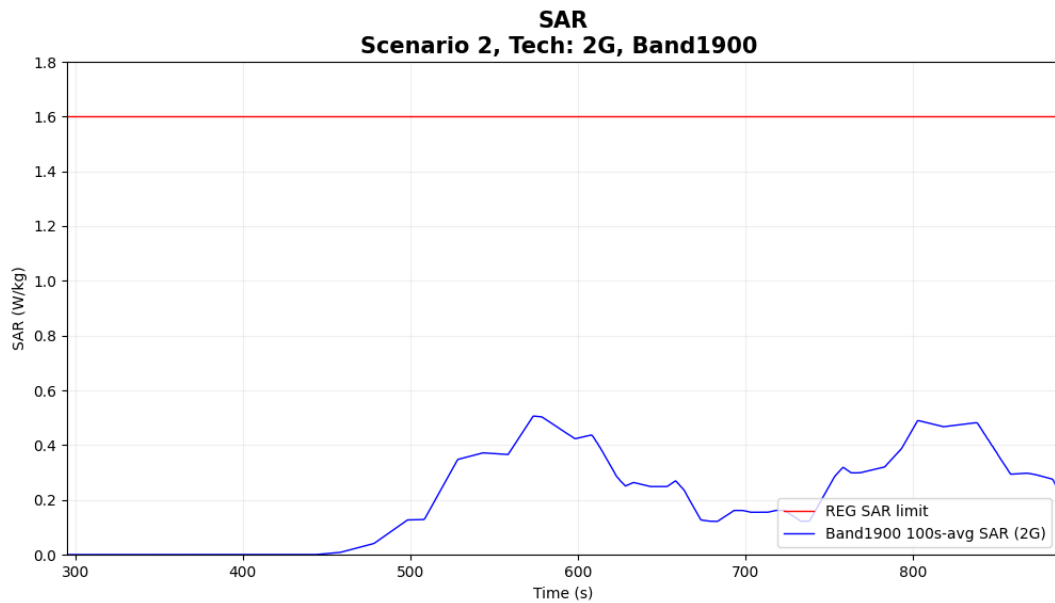
Figure 7-15 Time-averaged SAR for case 14 in table 7-1 (2G GSM 1900)
