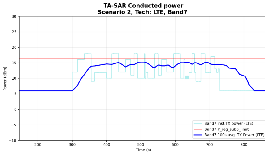
Figure 6-18 Time-averaged conducted TX power over time for case 2.8(LTE B7)
