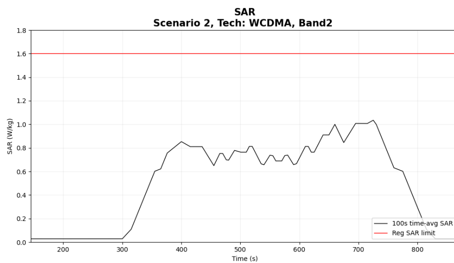
Figure 6-23 Time-averaged SAR for case 2.10(WCDMA B2)
