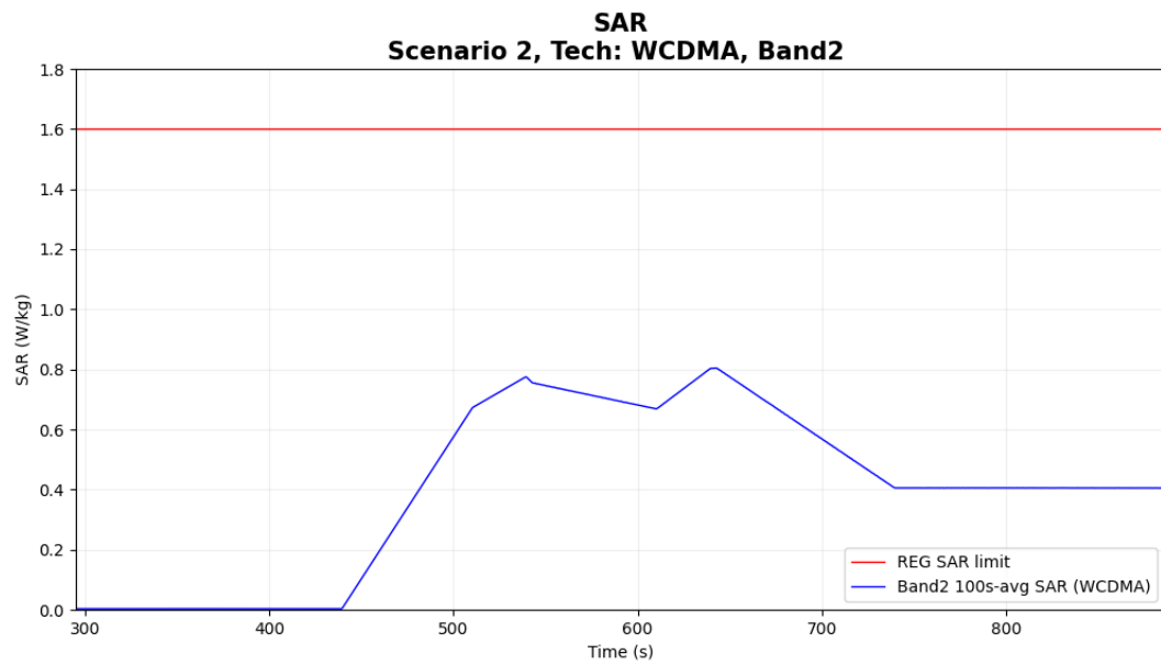
Figure 7-10 Time-averaged SAR for case 9 in table 7-1 (3G WCDMA B2)
