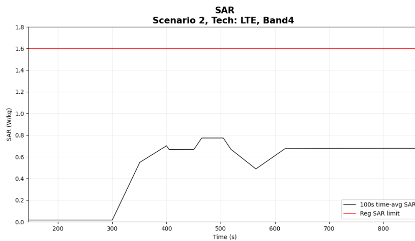
Figure 6-13 Time-averaged SAR for case 2.5(LTE B4)
