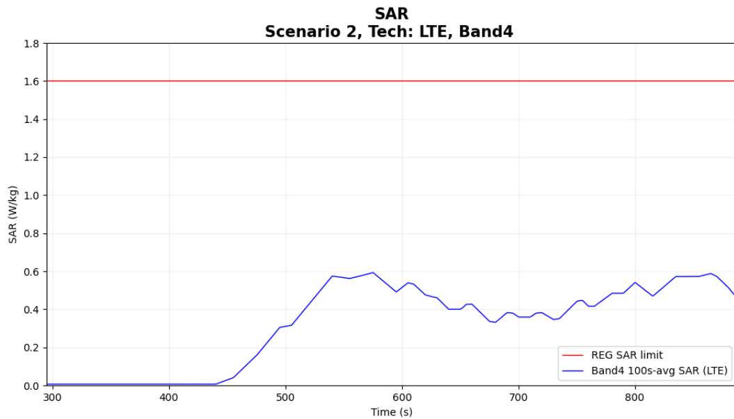
Figure 7-7 Time-averaged SAR for case 6 in table 7-1 (4G LTE B4)
