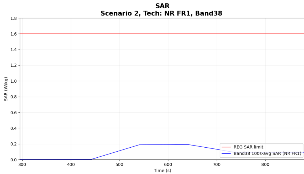
Figure 7-2 Time-averaged SAR for case 1 in table 7-1 (sub NR n38)
