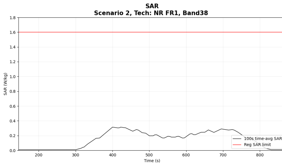
Figure 6-11 Time-averaged SAR for case 2.2(sub6 NR n38)
