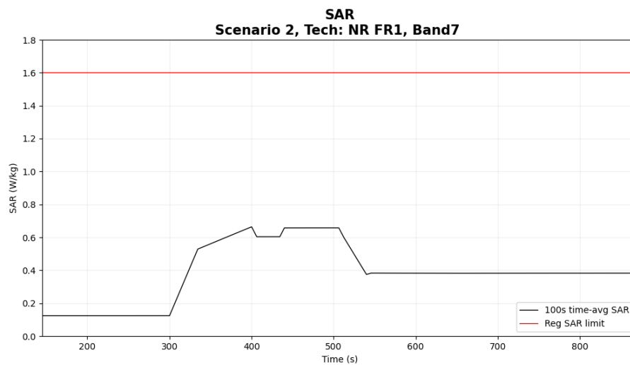
Figure 6-9 Time-averaged SAR for case 2.3(sub6 NR n7)
