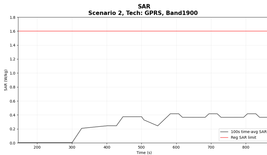
Figure 6-29 Time-averaged SAR for case 2.13(2G PCS1900)
