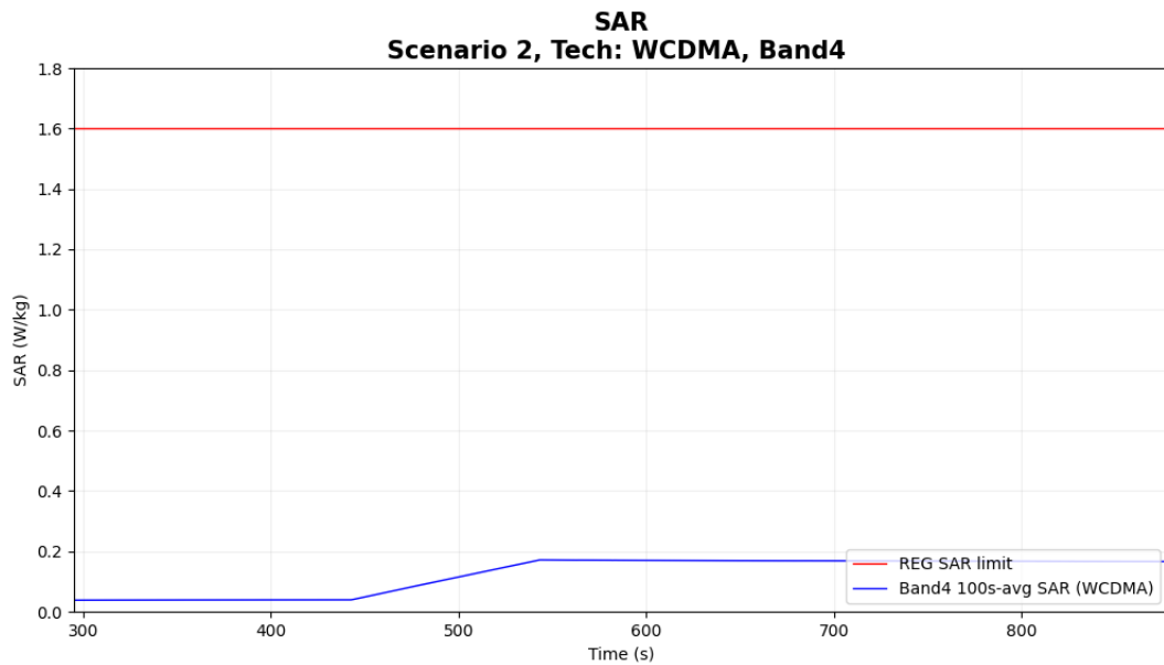
Figure 7-12 Time-averaged SAR for case 11 in table 7-1 (3G WCDMA B4)
