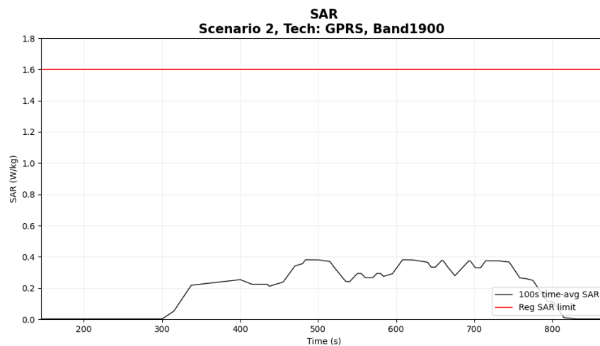
Figure 6-31 Time-averaged SAR for case 2.14(2G PCS1900)
