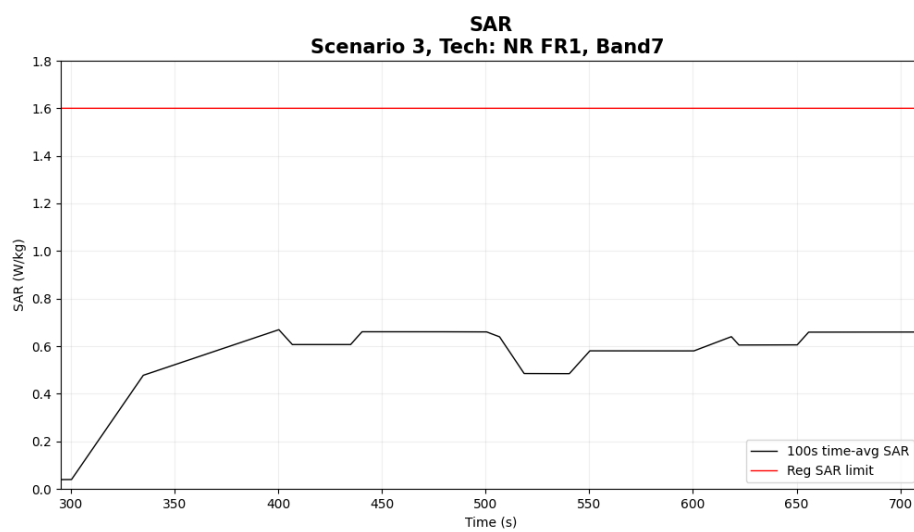
Figure 6-37 Time-averaged SAR for case 3.1(sub6 NR n7)
