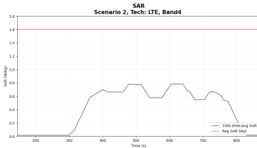
Figure 6-15 Time-averaged SAR for case 2.6(LTE B4)
