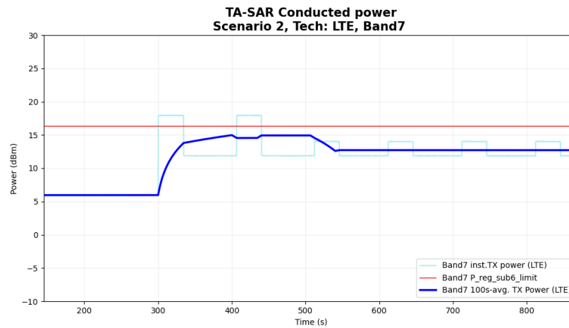
Figure 6-16 Time-averaged conducted TX power over time for case 2.7(LTE B7)
