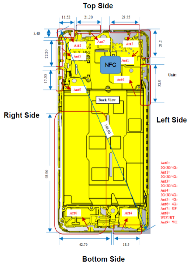
Figure 6-1 Antenna placement of the phone
