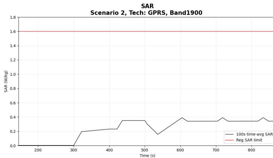
Figure 6-33 Time-averaged SAR for ase case 2.15(2G PCS1900)
