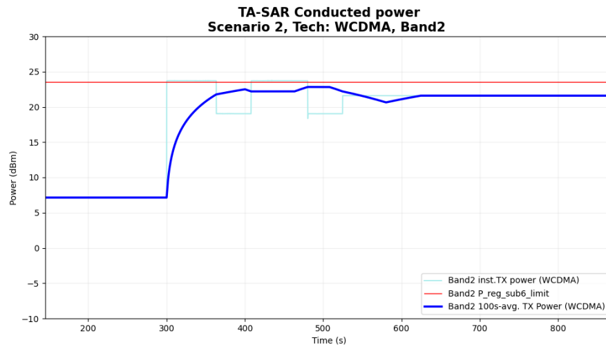
Figure 6-20 Time-averaged conducted TX power over time for case 2.9(WCDMA B2)
