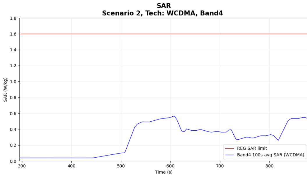
Figure 7-13 Time-averaged SAR for case 12 in table 7-1 (3G WCDMA B4)
