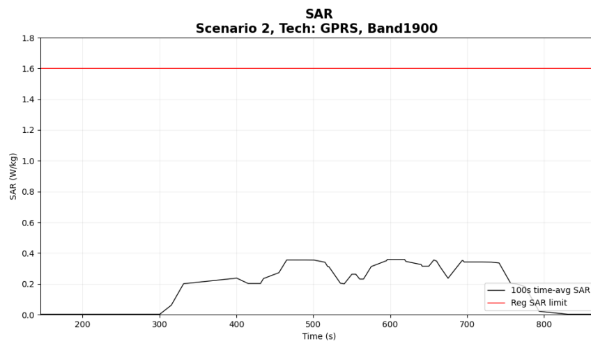
Figure 6-35 Time-averaged SAR for case 2.16(2G PCS1900)
