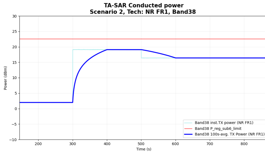
Figure 6-8 Time-averaged conducted TX power over time for case 2.1(sub6 NR n38)
