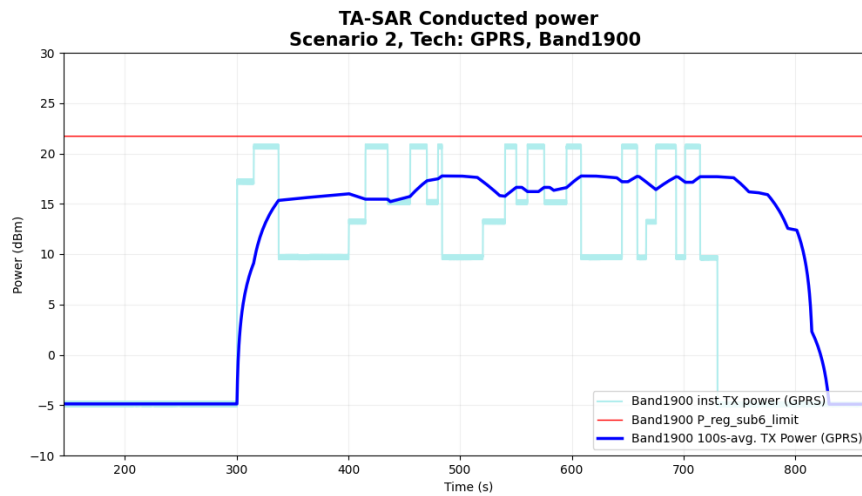
Figure 6-30 Time-averaged conducted TX power over time for case 2.14(2G PCS1900)
