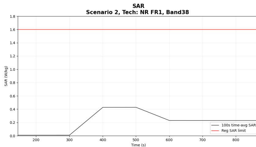
Figure 6-9 Time-averaged SAR for case 2.1(sub6 NR n38)
