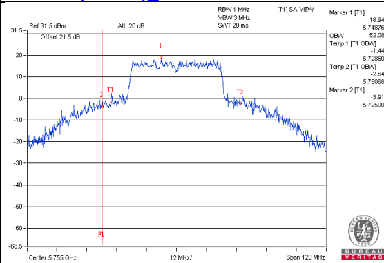
802.11ac(VHT40)_Chain1 / CH151
