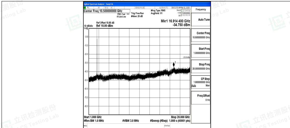
Band7_15MHz_QPSK_21375_1RB#0_1000~20000_1000~20000
