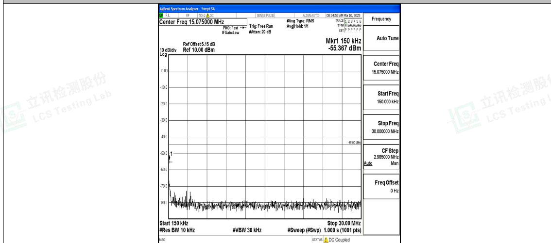
Band7_20MHz_QPSK_20850_1RB#0_0.15~30_0.15~30
