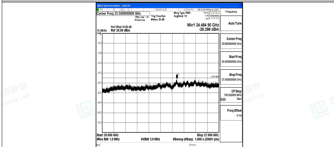
Band7_15MHz_QPSK_21375_1RB#0_20000~27000_20000~27000
