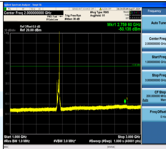
Band4_20MHz_16QAM_20300_1RB#99_1000~3000_1000~3000
