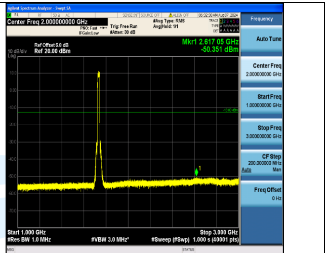
Band4_20MHz_16QAM_20175_100RB#0_1000~3000_1000~3000
