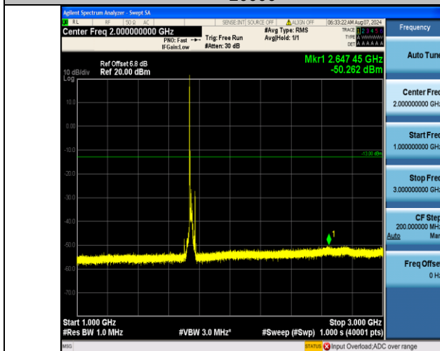
Band4_20MHz_16QAM_20300_1RB#0_1000~3000_1000~3000
