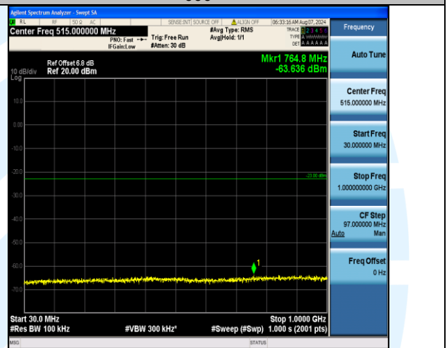
Band4_20MHz_16QAM_20300_1RB#0_30~1000_30~1000
