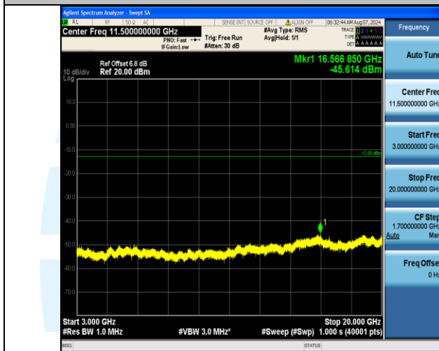
Band4_20MHz_16QAM_20175_100RB#0_3000~20000_3000~20000
