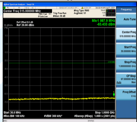
Band4_20MHz_QPSK_20175_1RB#0_30~1000_30~1000
