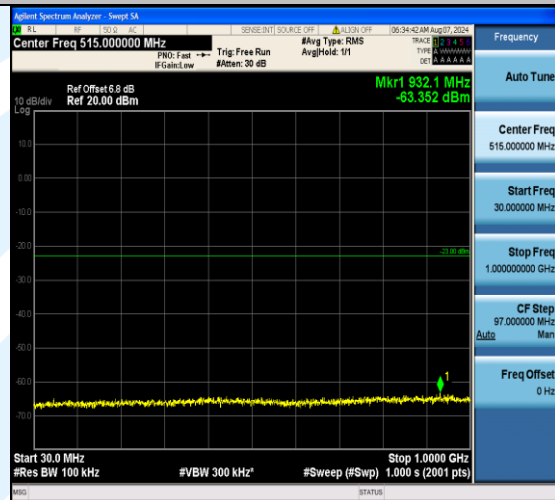
Band4_20MHz_16QAM_20300_100RB#0_30~1000_30~1000
