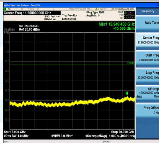
Band4_20MHz_16QAM_20300_100RB#0_3000~20000_3000~20000
