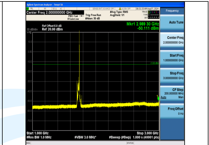
Band4_20MHz_QPSK_20175_1RB#99_1000~3000_1000~3000
