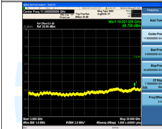
Band4_20MHz_QPSK_20050_100RB#0_3000~20000_3000~20000
