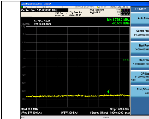
Band4_20MHz_16QAM_20175_100RB#0_30~1000_30~1000
