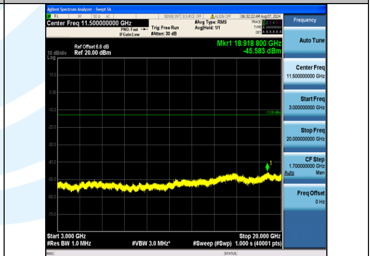
Band4_20MHz_QPSK_20175_100RB#0_3000~20000_3000~20000
