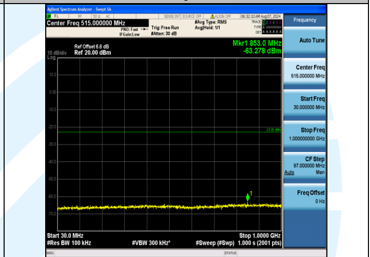
Band4_20MHz_QPSK_20175_100RB#0_30~1000_30~1000
