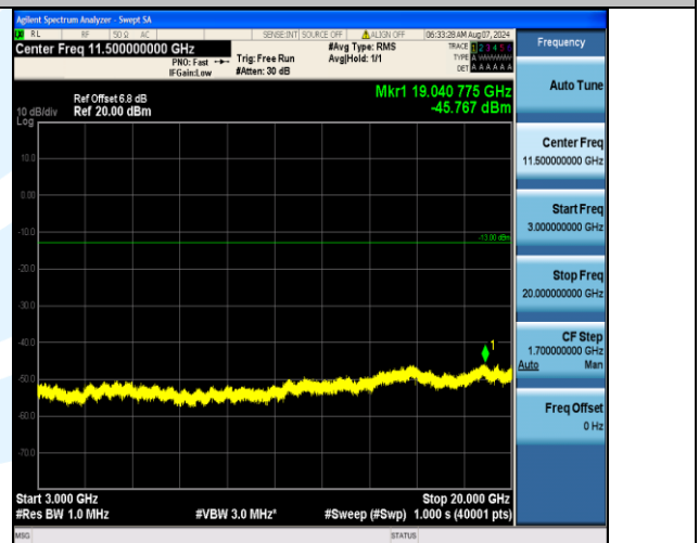
Band4_20MHz_16QAM_20300_1RB#0_3000~20000_3000~20000
