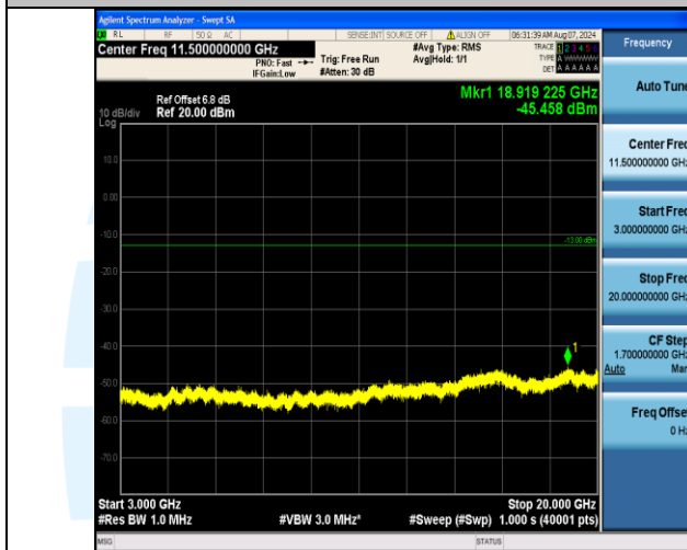
Band4_20MHz_QPSK_20175_1RB#99_3000~20000_3000~20000
